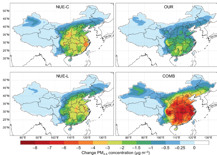
Figure 10. Changes of ground-level \text{PM}_{2.5} concentration of different mitigation scenarios.
