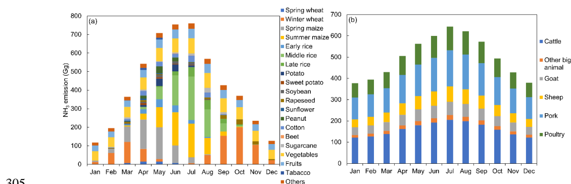
Figure 2. Monthly \text{NH}_3 emissions of specific crops (a) and livestock types (b).
