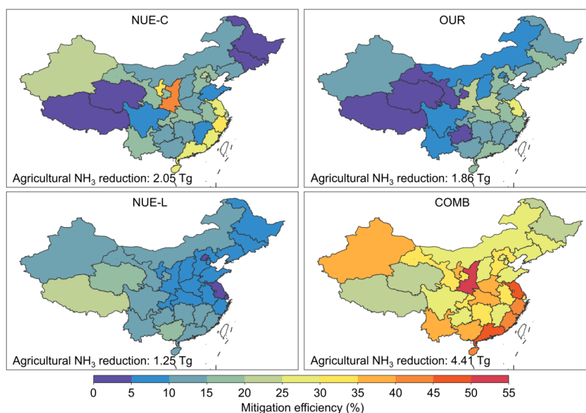
Figure 8. Mitigation efficiencies of NUE-C (a), OUR (b), NUE-L (c) and COMB (d) scenarios. Mitigation efficiency is the ratio of \text{NH}_3 emission reduction to baseline \text{NH}_3 emission.
