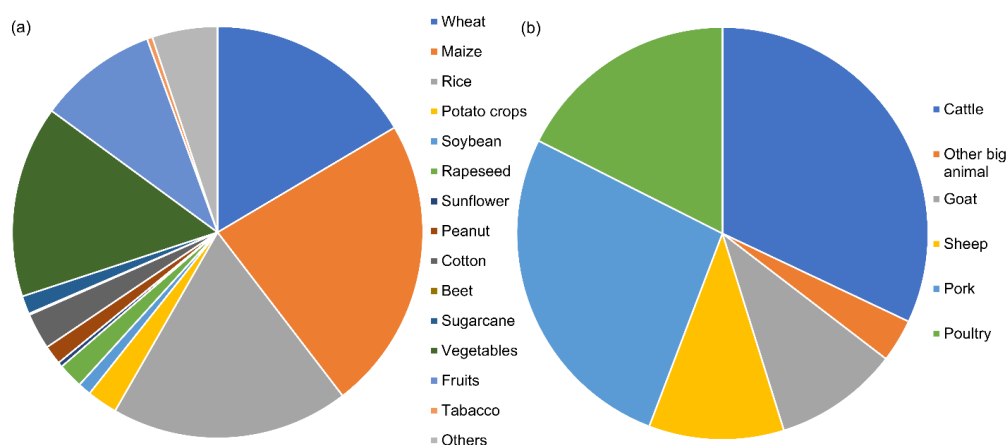
Figure 1. Different NH 3 emission sources associated with fertilizer application (a) and livestock manure (b).
