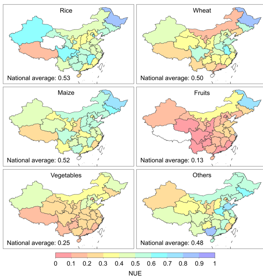
425 Figure 5. Nitrogen use efficiency of six crop types in China in 2017. The inserted values are the national average NUE for each crop type.
