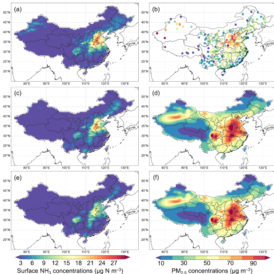
Figure 4. IASI-derived surface NH 3 concentrations (a) and observed PM 2.5 concentrations (b). The annual mean surface NH 3 concentration in 2017 simulated by our inventory (c) and MEIC (e). The annual mean ground-level PM 2.5 concentration in 2017 simulated by our inventory (d) and MEIC (f).
