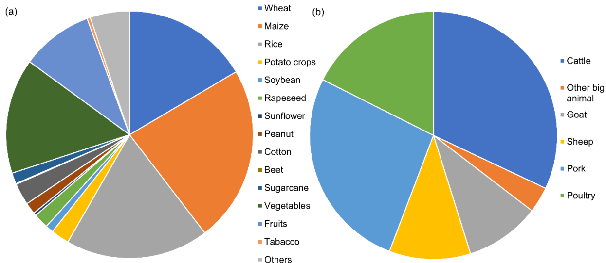
285 Figure 1. Different NH 3 emission sources associated with fertilizer application (a) and livestock manure (b).
