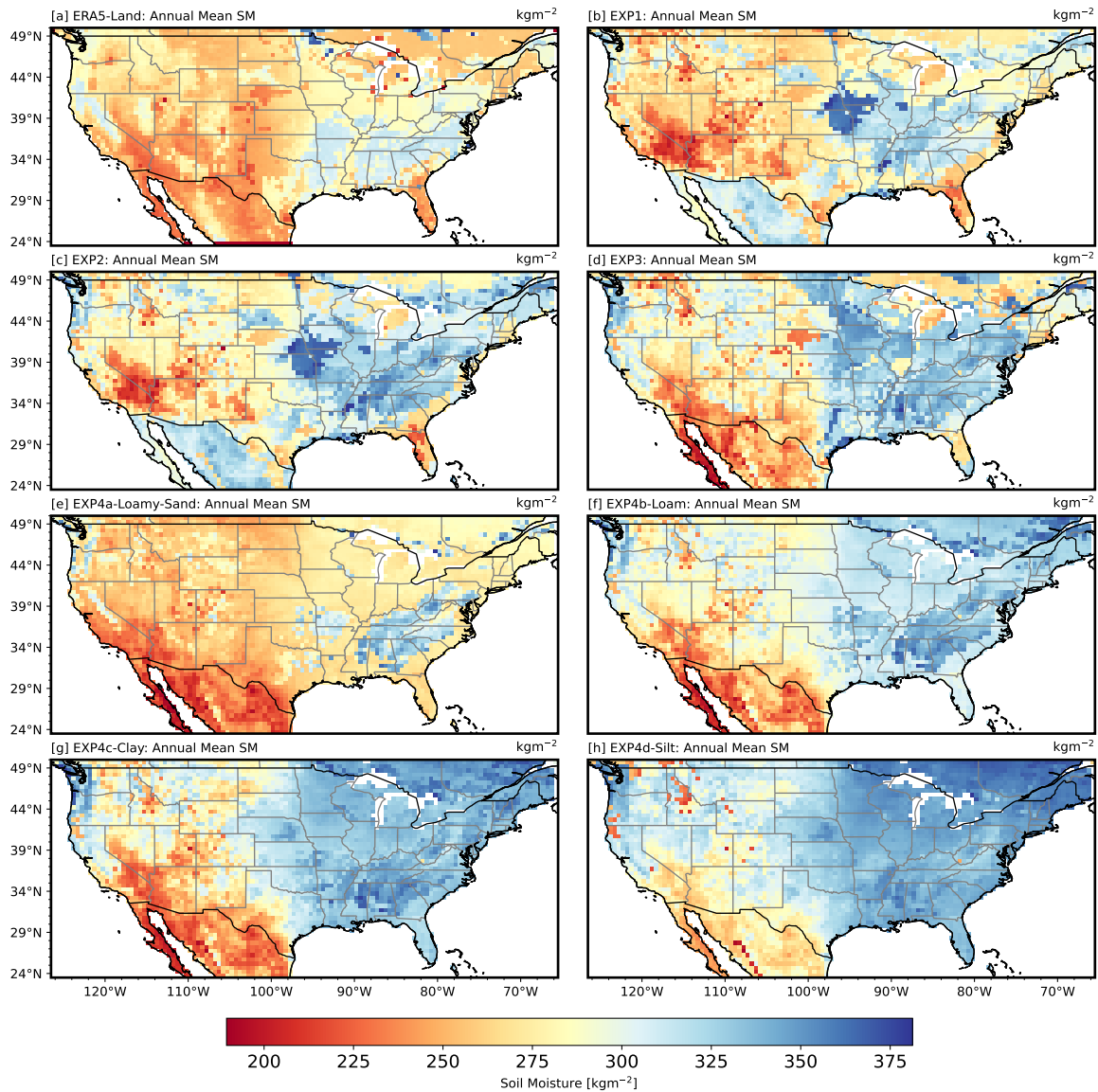
Figure 4. Annual mean soil moisture (1980–2010) over the CONUS region, simulated from four experiment types with spatially uniform soil parameter settings: EXP1 (b), EXP2 (c), EXP3 (d), and EXP4 (sub-experiments: EXP4a: loamy sand (e), EXP4b: loam (f), EXP4c: clay (g), and EXP4d: silt (h)). The color bar represents the range of soil moisture values ( \text{kg m}^{-2} ), with warmer colors (red and orange) indicating lower soil moisture levels and cooler colors (blue and purple) representing higher soil moisture levels.
