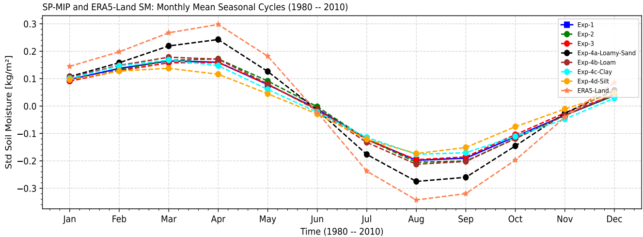
Figure 7. Monthly mean seasonal cycles of standardized root-zone soil moisture for the period 1980–2010 across the CONUS. CLM5 simulations (EXP1–EXP3 and EXP4a–d) are compared with ERA5-Land reanalysis. ERA5-Land exhibits the largest seasonal amplitude, with sharp increases during spring (March–June) and steep declines during summer (July–October). In contrast, EXP1–EXP3 form a tightly clustered group with flattened seasonal cycles, underestimating both the spring moisture accumulation and summer drawdown. EXP4a, which uses a loamy sand texture, shows greater seasonal responsiveness and more closely tracks ERA5-Land. The remaining EXP4 configurations (loam, clay, silt) progressively dampen seasonal variability, reflecting the influence of soil texture on water retention and hydrologic dynamics.
