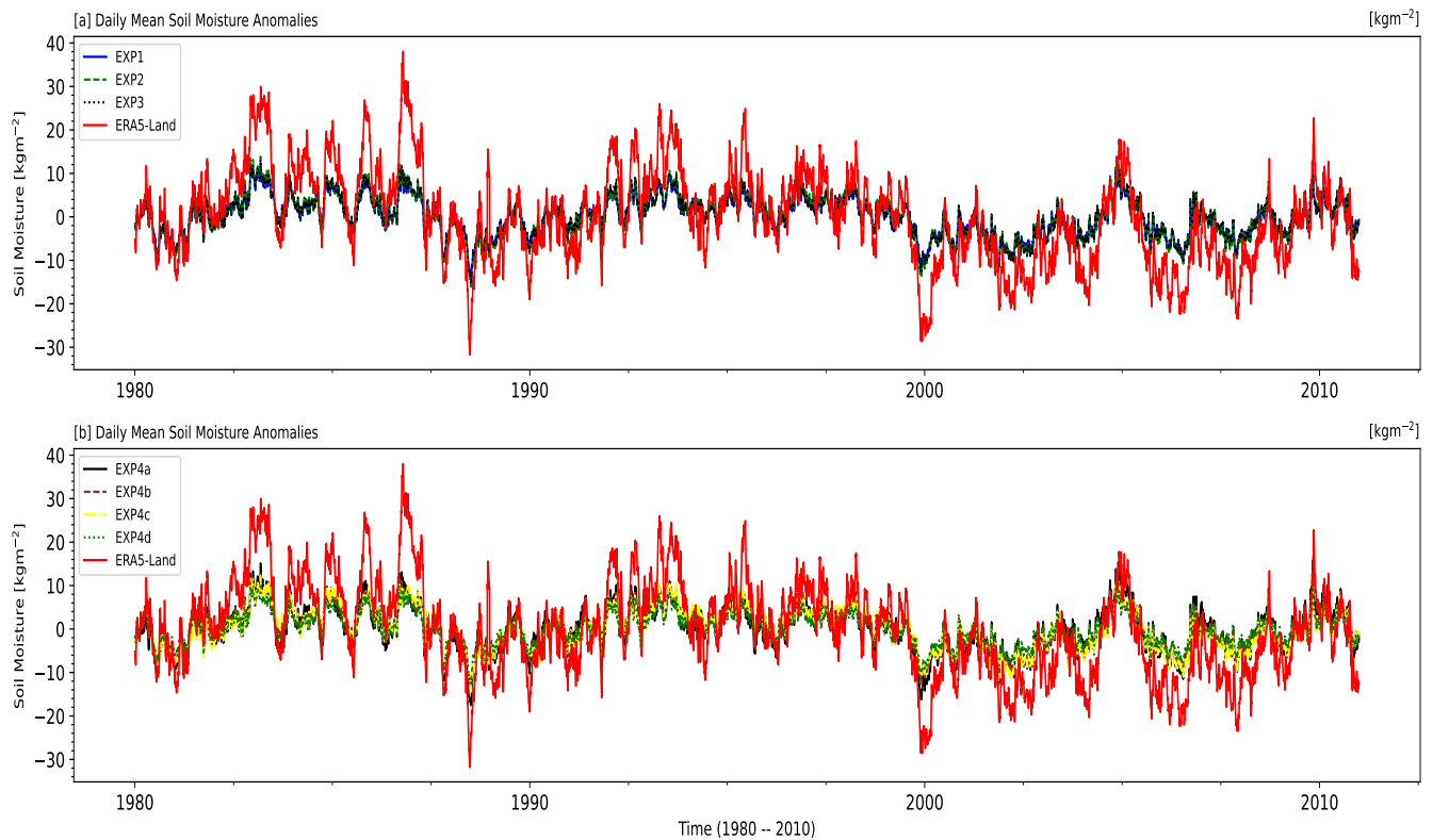
Figure 5. Time series of daily root-zone soil moisture anomalies from 1980 to 2010 over the CONUS region. Panel (a) shows anomalies for CLM5 simulations using EXP1, EXP2, and EXP3 configurations compared with ERA5-Land. Panel (b) includes EXP4 simulations with uniform soil texture classes (loamy sand, loam, clay, and silt), also compared against ERA5-Land. Anomalies are computed as deviations from the 30-year daily climatological mean. ERA5-Land exhibits a wider anomaly range, while CLM5 simulations show more constrained variability, highlighting differences in interannual amplitude across configurations.
