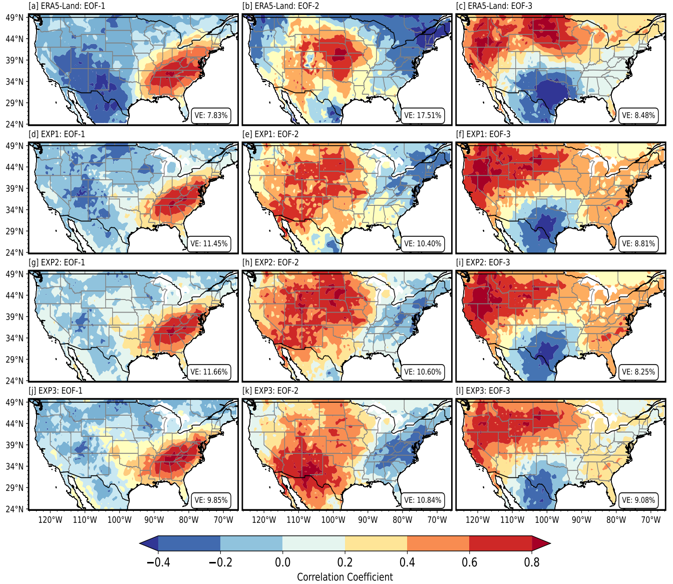
Figure 9. Spatial correlation maps of the first three EOFs of soil moisture anomalies for the CONUS, derived from ERA5-Land reanalysis data and three CLM5 experiments (EXP1, EXP2, EXP3). Panels (a) to (c) represent EOF-1, EOF-2, and EOF-3 from ERA5-Land, respectively. Panels (d–f), (g–i), and (j–l) show corresponding modes from EXP1, EXP2, and EXP3. The color shading represents the correlation coefficient between the PC time series of each EOF mode and the soil moisture anomaly time series at each grid point. Positive values indicate in-phase variability with the PC (regions that co-vary with the dominant mode), while negative values indicate anti-phase behavior. These maps illustrate the spatial coherence and phase relationships of soil moisture variability associated with each mode.
