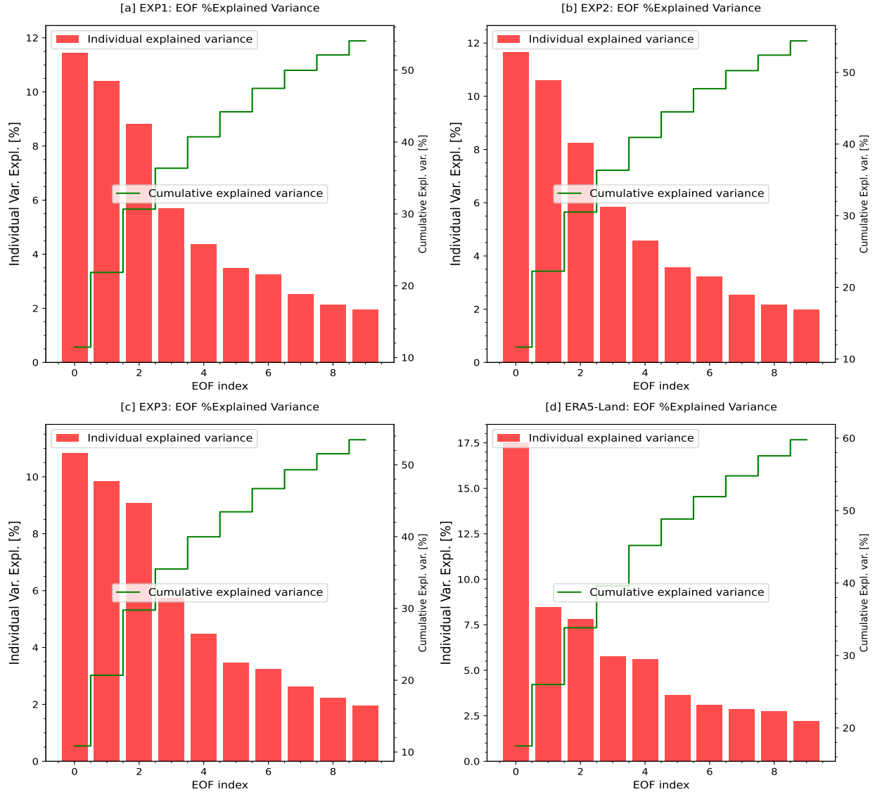
Figure 8. The variance explained by each separate and combined EOF in the CLM5 soil moisture experiment is depicted. Red bars represent the contribution of each EOF individually, while the green line shows the cumulative proportion for the initial 10 EOF modes.
