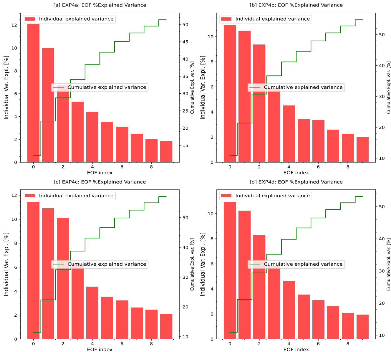
Figure A1. Contribution of Variance by Individual and Cumulative EOFs in CLM5 Soil Moisture Experiments. The red bars indicate the portion of variance each separate EOF mode accounts for, whereas the green line depicts the cumulative percentage of variance explained by the first ten EOF modes. These plots reveal the significant impact of the early EOF modes in accounting for variance. Panels (a) to (d) relate to different experimental configurations or scenarios, offering a comparative assessment of EOF variance contributions.
