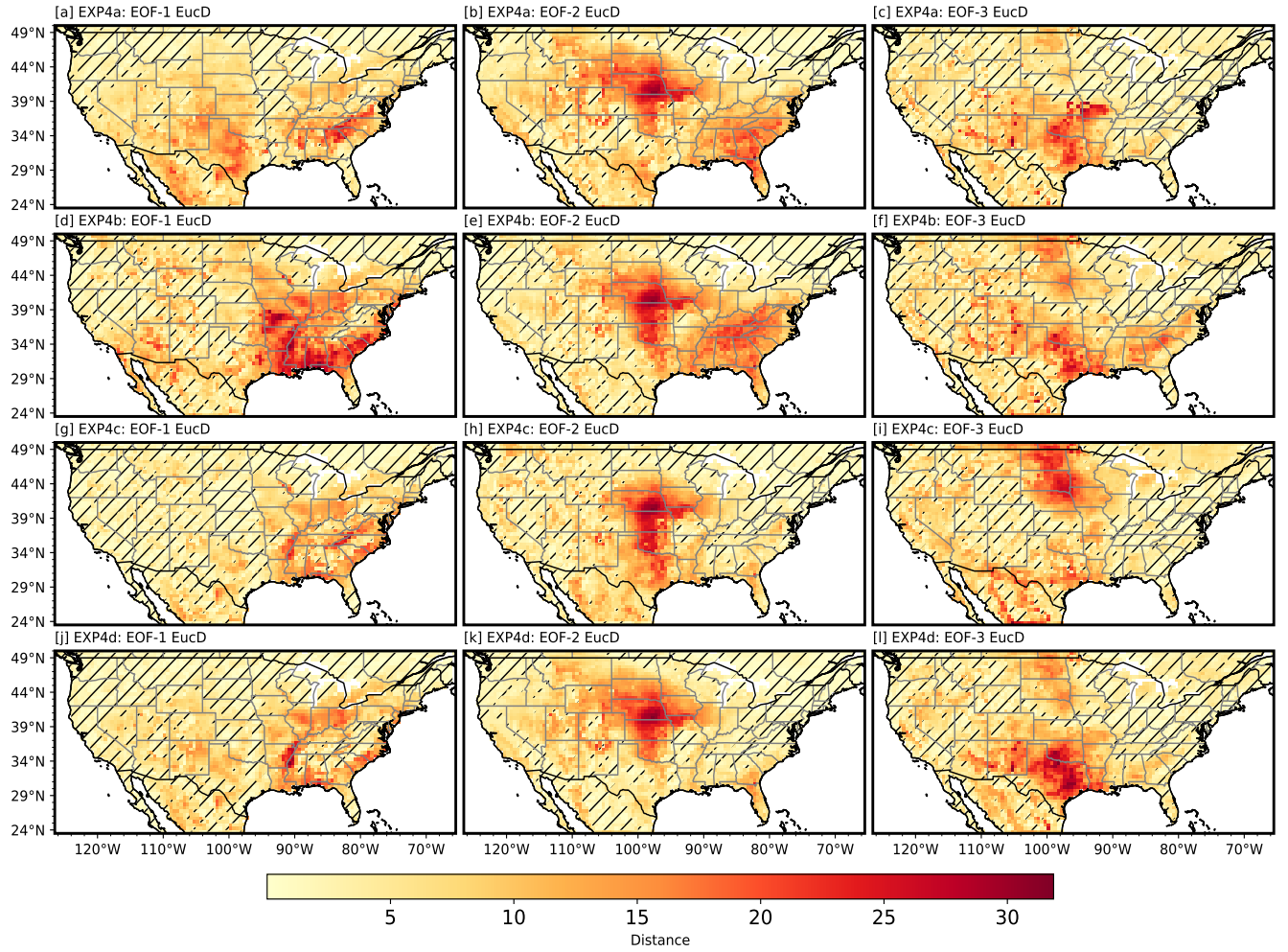
Figure A4. The Euclidean distance between EOF modes from SP-MIP experiments (EXP4a, EXP4b, EXP4c, EXP4d) and ERA5-Land is depicted. Panels (a–c) illustrate results for Experiment 4a (Loamy Sand), while panels (d–f), (g–i), and (j–l) pertain to Experiments 4b (Loam), 4c (Clay), and 4d (Silt), respectively. Each column showcases one of the first three EOF modes: EOF-1, EOF-2, and EOF-3. The color bar represents the Euclidean distance, where lower values (yellow) reflect stronger alignment with ERA5-Land, whereas higher values (red) denote more significant discrepancies. Regions with hatched patterns signify distances less than 5, emphasizing areas where the experiments closely align with the ERA5-Land data. These observations reveal the spatial variability in model performance across different soil hydraulic parameter settings and EOF modes.
