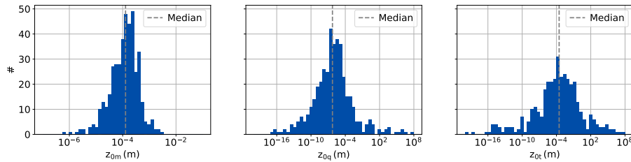
Figure A1. Histograms of the hourly roughness length values derived from the EC-IRGASON and PROMICE AWS observations.
