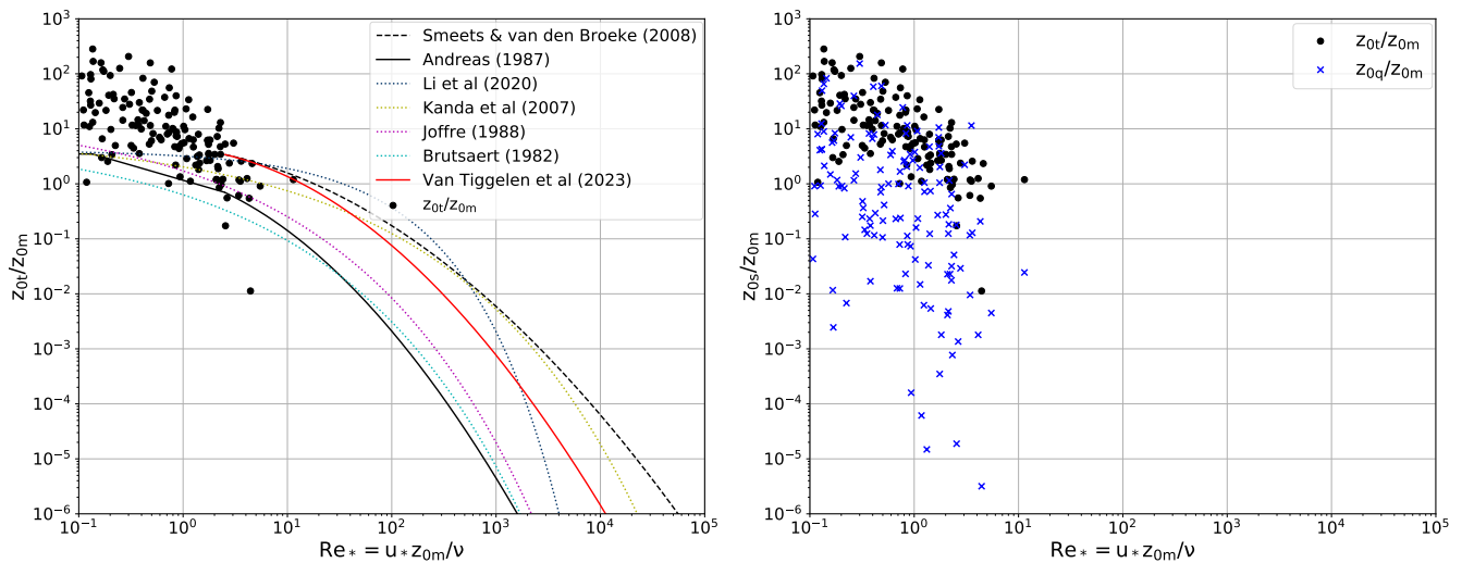
Figure A2. The hourly ratio of z_{0,t}/z_{0,m} from the EC-IRGASON and PROMICE AWS observations against the roughness Reynolds number Re_* = u_* z_{0,m}/\nu . Plotted together with (a) lines denoting the parameterisation from Smeets and Van den Broeke (2008b), Andreas (1987), Li et al. (2020), Kanda et al. (2007), Joffre (1988), Brutsaert (1982) and Van Tiggelen et al. (2023) and (b) the hourly z_{0,q}/z_{0,m} ratio from the EC-IRGASON and PROMICE AWS observations. The EC-IRGASON values are hourly averages of the 10-minute covariances.
