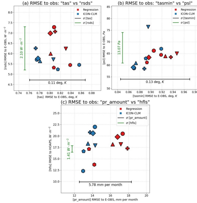
Figure 8. The monthly mean RMSEs (Eq. 1) to observations for ICON-CLM simulations (blue markers) and corresponding regression results (red markers) for all parameter setups from Latin Hypercube . Corresponding dynamical and linear setups are indicated by the same marker shape. The 2003-2008 monthly mean biases-RMSEs are shown for: (a) daily mean 2-meter temperature tas versus daily mean rsds , (b) daily minimum 2-meter temperature tasmin versus daily mean sea level pressure psl , (c) monthly total precipitation pr_amount versus daily mean latent heat flux hfls . The 2003-2008 mean internal variabilities of the model (Eq. 2) are shown as horizontal and vertical segments.
