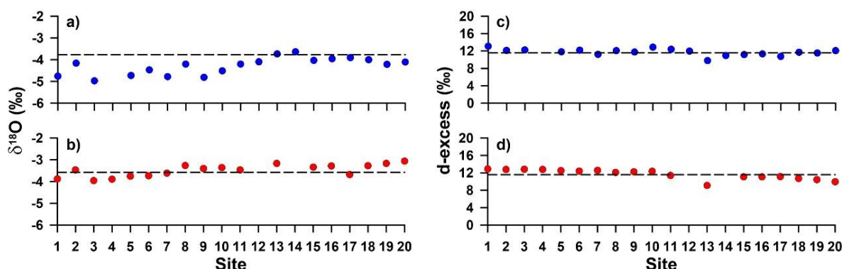
Figure 4: (a, b) Oxygen-18 ( \delta^{18}\text{O} ) isotopic ratios and (c, d) d -excess values in stream water samples collected at the 20 sampling sites within the Cube River catchment during the wettest (dark blue circles in a and c) and driest (red circles in b and d) sampling periods (i.e. M2 and M6 in Fig. 3). The dashed lines in a) and b) represent the average \delta^{18}\text{O} value (-3.7‰) and in c) and d) represent the average d -excess value (+11.6‰) of the samples collected at all monitoring sites during the six monitoring campaigns carried out in 2021 for reference, respectively. In the x-axis, the sampling sites are ordered according to the elevation of their outlets, generally corresponding to the sites with the smallest drainage areas to be located at the Cube River headwaters and the sites with the largest drainage areas downstream toward the catchment's outlet (Fig. 1a and Table 1).
