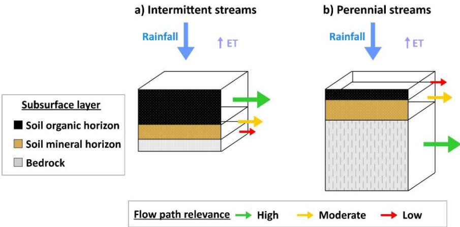
Figure 9: Conceptual model of subsurface water flow paths influencing streamflow generation in a) intermittent and b) perennial tropical streams under changing land use at the Cube River catchment, northern Ecuador. The white surface at the top of the boxes represents the surface at the ground level. The size of the coloured boxes representing the soil and bedrock subsurface layers indicates their relative capacity to store water below ground. The dashed vertical lines in the bedrock layer of subplot b) denote the high bedrock permeability of the underlying geology at subcatchments draining perennial streams, as opposed to the almost impermeable bedrock underlying intermittent subcatchments depicted in a). Overland flow has not been observed in intermittent or perennial streams during field sampling campaigns, and thus, such a streamflow generation mechanism is neglected in the conceptual diagrams. The size and colour of the horizontal arrows represent the relative relevance of various water flow paths influencing streamflow generation.
