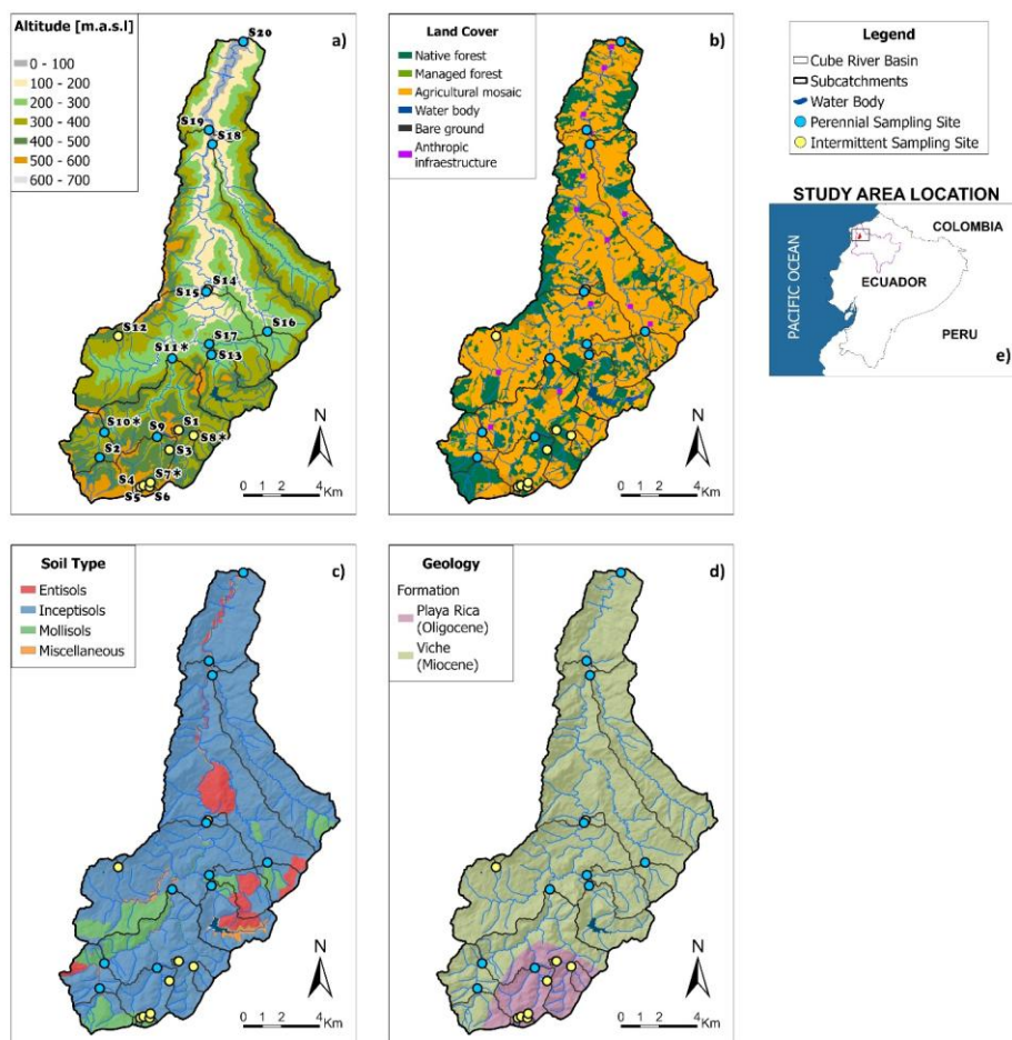
Figure 1: Cube River catchment (159 km 2 ) biophysical maps of: a) altitude, b) land cover, c) soil type, and d) geology. e) Location of the Cube River catchment (red area) in the lower part of the Esmeraldas River basin (purple line) in northwestern Ecuador. Maps a) to d) show the Cube River catchment drainage network and the intermittent (yellow circles) and perennial (blue circles) sampling sites at the outlet of 19 nested subcatchments (S1 to S19) and the outlet of the catchment (S20) where hydrologic, geochemical, and isotopic data were collected during six monitoring campaigns during the period January-December 2021. The * symbol next to the name of the sampling sites in a) denotes sites where water level data were continuously monitored during the study period.
