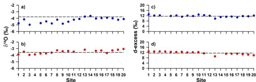
Figure 4: (a, b) Oxygen-18 ( \delta^{18}\text{O} ) isotopic ratios and (c, d) d -excess values in for stream water samples collected at the 20 sampling sites within the Cube River catchment during the wettest (dark blue circles in a and c) and driest (red circles in b and d) sampling periods (i.e. M2 and M6 in Fig. 3). The dashed lines in a) and b) represent the average \delta^{18}\text{O} value ( -3.7\text{‰} ) and in c) and d) represent the average d -excess value ( +11.6\text{‰} ) of the samples collected at all monitoring sites during the six monitoring campaigns carried out in 2021 for reference, respectively. In the x-axis, the sampling sites are ordered according to the elevation of their outlets, generally corresponding to the sites with the smallest drainage areas to be located at the Cube River headwaters and the sites with the largest drainage areas downstream toward the catchment's outlet (Fig. 1a and Table 1).
