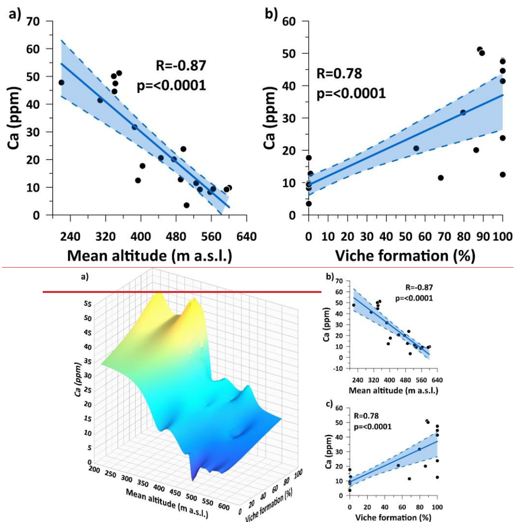
Figure 27: a) 3D surface plot showing the relation among mean altitude, the areal extent of the Viche formation, and Ca concentration for the 20 sampling sites monitored within the Cube River catchment during six monitoring campaigns carried out in 2021. Correlations b) between a) mean altitude and Ca concentration and c) between the areal extent of the Viche formation and Ca concentration. Note that the color scheme in a) is only used to visualize the interplay between the predictor variables (mean altitude and Viche formation) and the response variable Ca concentrations.
