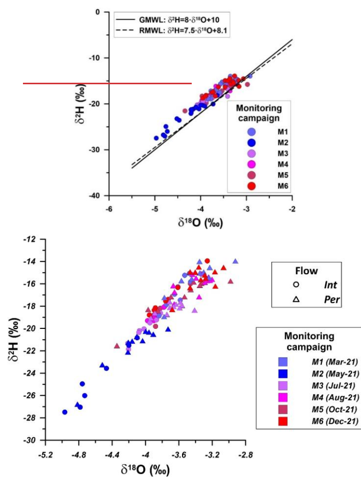
Figure 3: Relationship between oxygen-18 ( \delta^{18}\text{O} ) and hydrogen-2 ( \delta^2\text{H} ) isotopic ratios in stream water samples collected at the 20 sampling intermittent (circles) and perennial (triangles) sites within the Cube River catchment during six monitoring campaigns (M1-M6) carried out during the wet (M1 and M2), transition (M3) and dry (M4, M5, and M6) periods in 2021. The date of the sampling campaigns (mm-yy) is shown in parentheses in the legend. Monitoring campaigns M2 and M6 correspond to the wettest (dark blue circleless symbols) and driest (red circleless symbols) sampling periods, respectively. The Global Meteoric Water Line (GMWL) and a Regional Meteoric Water Line (RMWL) constructed using available data from two nearby stations of the Global Network of Isotopes in Precipitation (GNIP) database. Click or tap here to enter text. are also displayed for reference. Metadata, geographical information, isotopic data statistics, and source of the GNIP stations used in this analysis are presented in Table S1 as supplementary material.
