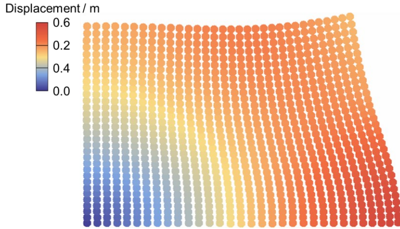
Figure 20. Displacement distribution at 0.5 s.
