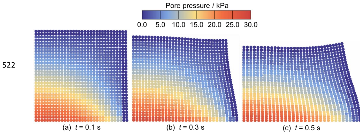
523 Figure 17. Pore pressures distribution at different times.
