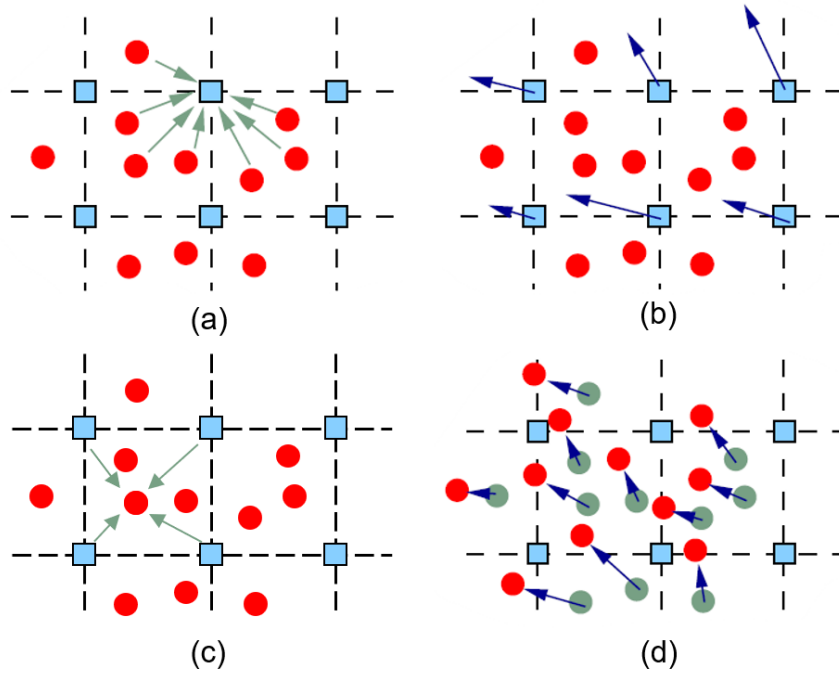
Figure 1. Standard algorithm of MPM: (a) interpolating information from particles to nodes; (b) solving governing equations on nodes; (c) interpolating information from nodes to particles; (d) update particles information.
