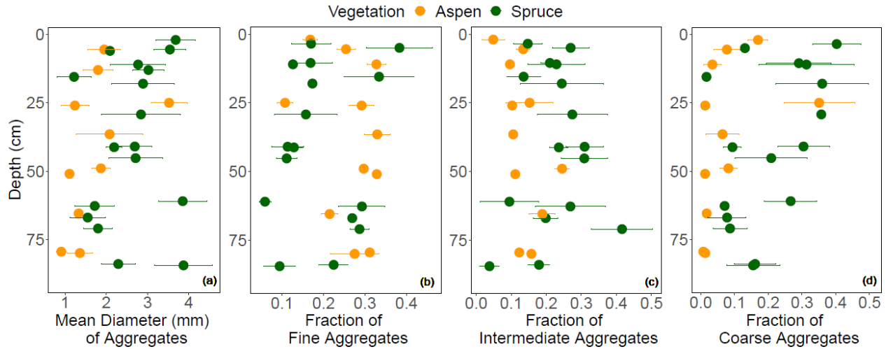
Figure 10: The geometric mean and standard deviation of (a) all aggregates, and fraction of (b) fine aggregates ( < 0.21 mm), (c) intermediate aggregates ( 0.21 - 4.76 mm), and (d) coarse aggregates ( > 4.76 mm). Colors are associated with vegetation, aspen (orange) and spruce (green).
