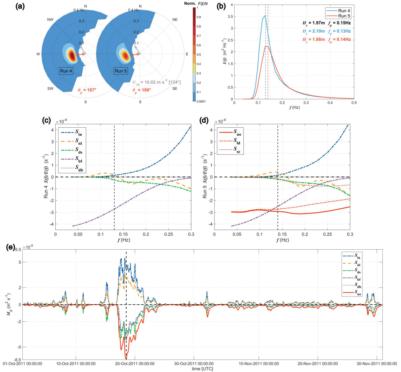
Figure 12: (a) Wave spectra F(f, \theta) at buoy 55032 at 1300 UTC 18 Oct 2011 from Run 4 (without S_{uo} ) and Run 5 (with S_{uo} ), respectively. The grey and red arrows denote wind and peak wave directions. (b) The corresponding 1D wave spectra E(f) with the respective wave height H_s and peak frequency f_p . Buoy observations are shown in black color. (c, d) The corresponding source terms, each normalized by the spectra from Run 4 (without S_{uo} ) and Run 5 (with S_{uo} ), respectively. In panel (d), the unresolved obstacle-related parameterization S_{uo} , together with the separate local dissipation ( S_{ld} ) and shadow effect ( S_{se} ), are shown as red lines. Evolution of the source term magnitude M_s at 55032 for the two-month period is shown in panel (e). Note that when
