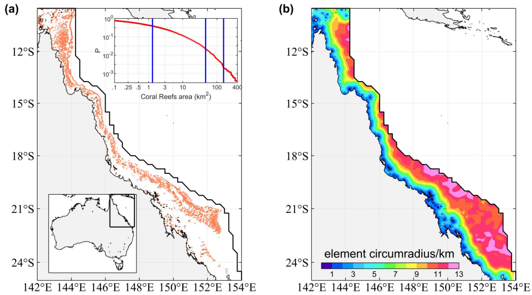
Figure 2: (a) The northeastern coast of Australia and the Great Barrier Reef (GBR; orange color) located inside our model domain (delimited by the black curve). The reef outlines (polygons) are from the multi-source global dataset of warm-water coral reefs compiled by UNEP-WCMC et al. (2010; version 4.1 with the highest resolution of 30 m). The inset displays the exceedance probability distribution of the area of individual reef polygons. The three blue vertical lines highlight the areas for characteristic equilateral triangular elements with a circumradius of 1, 6 and 11 km, respectively. (b) Same as Fig. 1b but for the mesh resolution zoomed in around the GBR.
