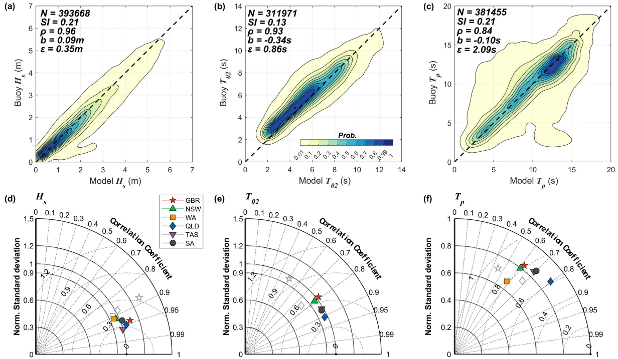
Figure 9: Comparison of the (a) significant wave height H_s , (b) mean period T_{02} and (c) peak period T_p between a total of 28 wave buoys and the WW3-ST6 simulation Run 5 (with S_{u0} ; Table 2). Taylor diagrams summarizing the comparison between Run 5 (colored, full markers) and buoys at different regions for (d) H_s , (e) mean period T_{02} and (f) peak period T_p . For comparison, the grey, empty markers illustrate the performance of Run 4 (without S_{u0} ) in the GBR (star), WA (square) and QLD (diamond) regions. Buoys are divided into groups according to Fig. 6.
