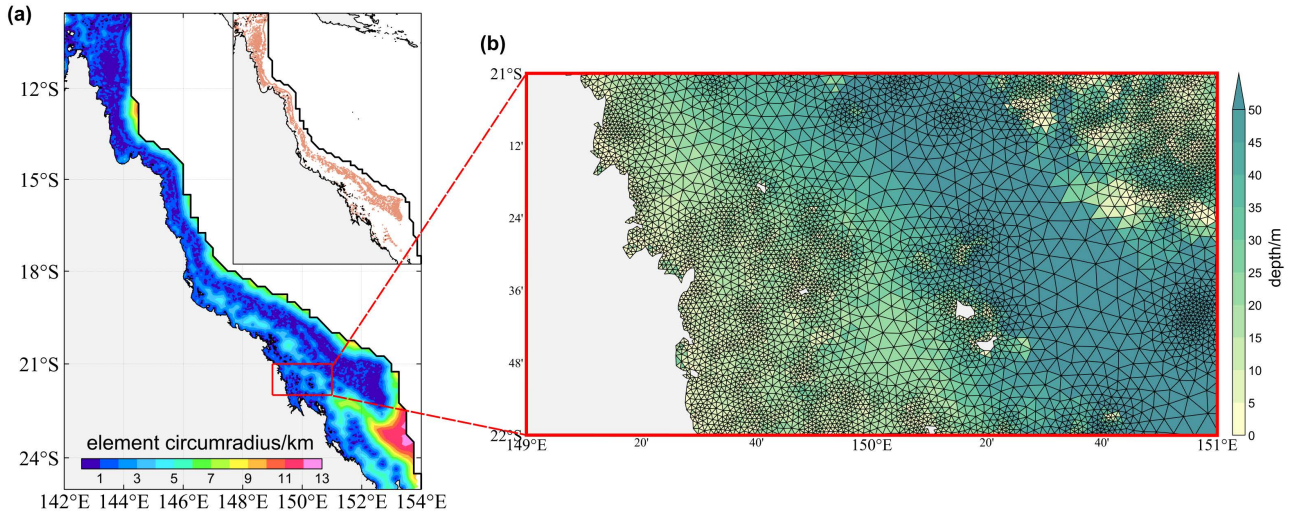
Figure 13: (a) The mesh resolution (in terms of the local element circumradius; unit: km) of the mesh version 2 (details in Table 1) zoomed in around the GBR. (b) The triangular grid (mesh v2) with varying resolutions zoomed in at a 1^\circ \times 2^\circ bin off the northeast coast of Australia.
