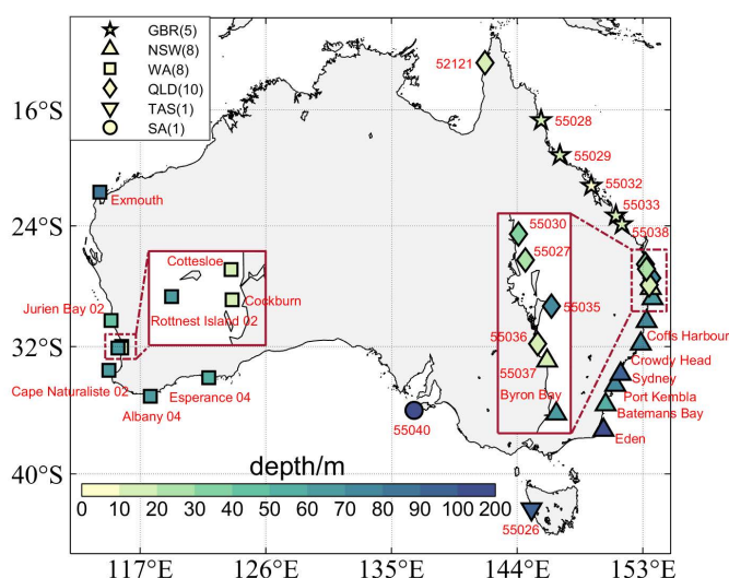
285 Figure 6: Locations and water depth of wave buoys sourced from the AODN used for validating wave simulations. For clarity, zoomed-in views of wave buoys near Perth and Brisbane are shown in the left and right insets, respectively. Buoys are grouped according to the Australian administrative divisions, including New South Wales (NSW), Western Australia (WA), Queensland (QLD), Tasmania (TAS), South Australia (SA). Note that the wave buoys in the GBR, although belonging to the QLD group, are highlighted separately with the star symbols.
