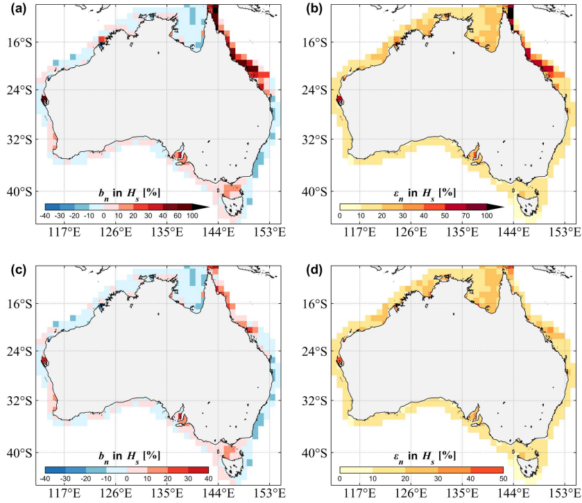
350 Figure 7: Error statistics of the significant wave height H_s gridded in 1^\circ \times 1^\circ bins for the WW3 (a, b) Run 4 (without the S_{u0} approach) and (c, d) Run 5 (with S_{u0} ) relative to the altimeter wave records: (a, c) the normalized bias b_n , (b, d) normalized RMSE \varepsilon_n . The ERA5 winds and ACCESS currents were adopted to force these two runs. The similar figure for the absolute bias b and RMSE \varepsilon can be found in the Supplements (Fig. S6).
