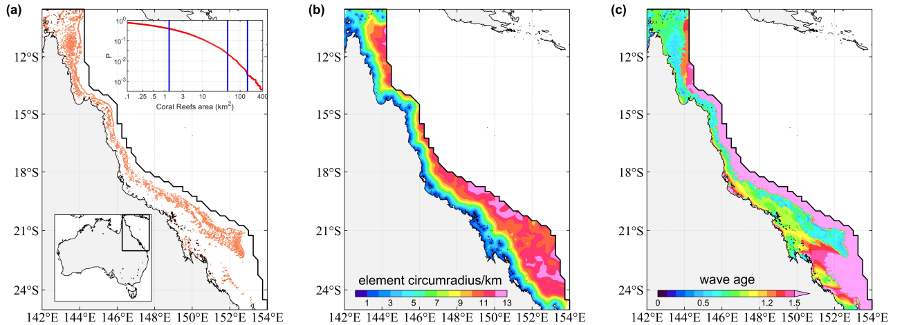
175 Figure 2: (a) The northeastern coast of Australia and the Great Barrier Reef (GBR; orange color) located inside our model domain (delimited by the black curve). The reef outlines (polygons) are from the multi-source global dataset of warm-water coral reefs compiled by UNEP-WCMC et al. (2010; version 4.1 with the highest resolution of 30 m). The inset displays the exceedance probability distribution of the area of individual reef polygons. The three blue vertical lines highlight the areas for characteristic equilateral triangular elements with a circumradius of 1, 6 and 11 km, respectively. (b) Same as Fig. 1b but for the mesh resolution zoomed in around the GBR. (c) Spatial distribution of wave age in the GBR based on the Run 7 simulation (see Table 2) for the year 2011.
