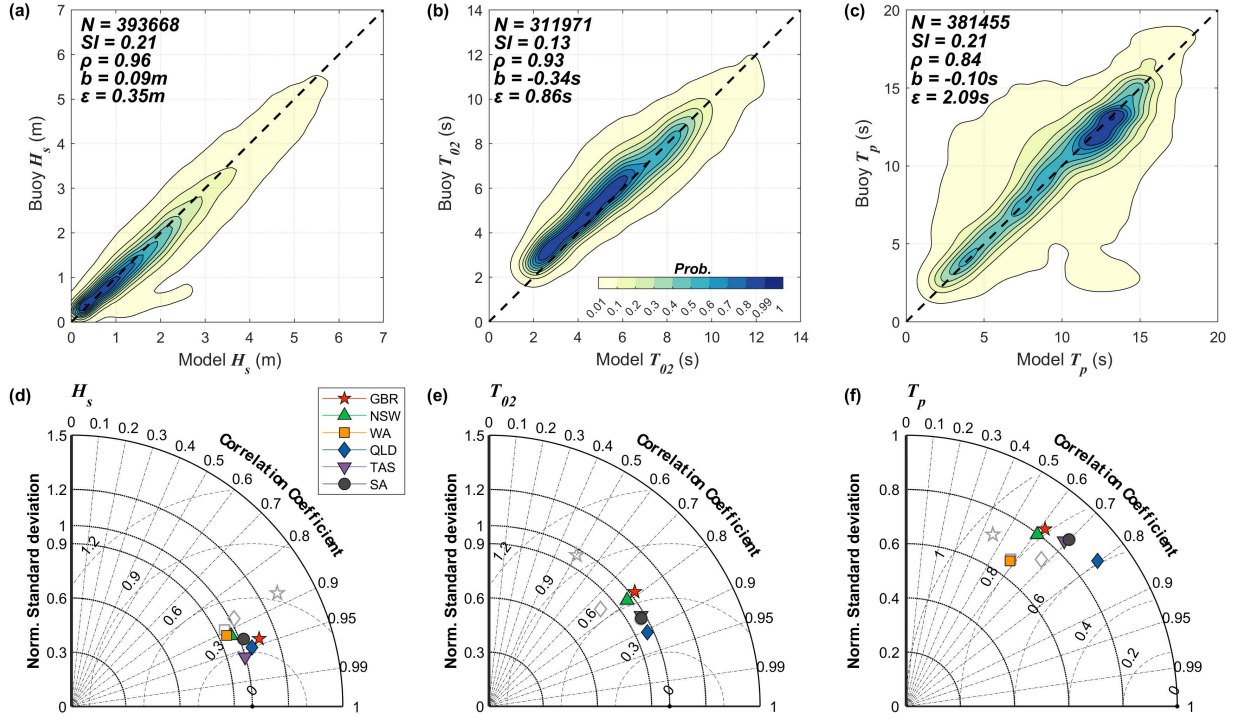
390 Figure 9: Comparison of the (a) significant wave height H_s , (b) mean period T_{02} and (c) peak period T_p between a total of 28 wave buoys and the WW3-ST6 simulation Run 5 (with S_{uo} ; Table 2). Taylor diagrams summarizing the comparison between Run 5 (colored, full markers) and buoys at different regions for (d) H_s , (e) mean period T_{02} and (f) peak period T_p . For comparison, the grey, empty markers illustrate the performance of Run 4 (without S_{uo} ) in the GBR (star), WA (square) and QLD (diamond) regions. Buoys are divided into groups according to Fig. 6.
