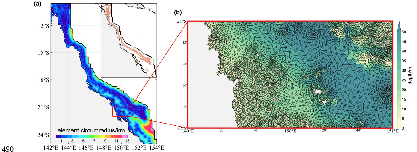
Figure 13: (a) The mesh resolution (in terms of the local element circumradius; unit: km) of the mesh version 2 (details in Table 1) zoomed in around the GBR. (b) The triangular grid (mesh v2) with varying resolutions zoomed in at a 1^\circ \times 2^\circ bin off the northeast coast of Australia.
