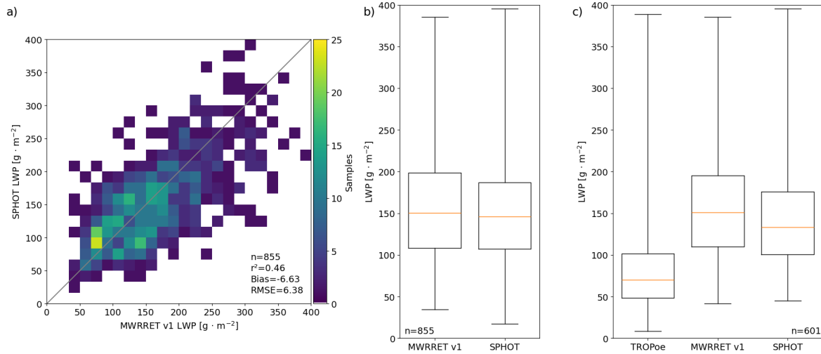
Figure 5: (a) Scatterplot of LWP retrievals and associated R^2 , Bias and RMSE [ \text{g m}^{-2} , bin size 16 \text{ g m}^{-2} ] from the SPHOT and MWRRET ("Version 1"). Box and whisker plots for LWP distribution quartiles and extremes, with distribution medians in yellow for (b) cumulative SPHOT and MWRRET datasets, and (c) datasets including TROPoe product availability.
