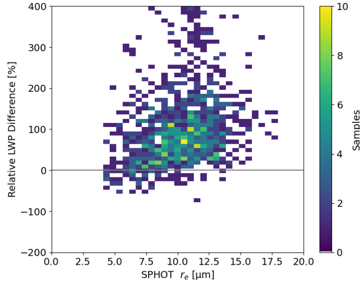
370 Figure 7: Scatterplot for the relative difference (TROPoe minus SPHOT retrieval divided by the TROPoe retrieval) in LWP estimates as a function of the associated SPHOT r_e retrieval estimate (bin size 0.5 \mu\text{m} and 10 \text{ g m}^{-2} ).
