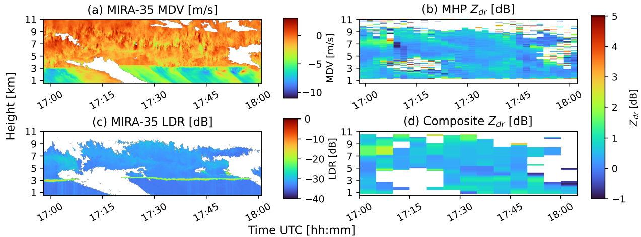
Figure 12. Measured mean Doppler velocity (a) and linear depolarisation ratio (c) of MIRA-35 in vertical profiles, differential reflectivity in extracted vertical profiles based on RHI scans of MHP (b) and differential reflectivity in a BA-CVP composite of ISN and MEM (d) for data collected on 08 July 2021 between 16:58 UTC and 18:01 UTC.
