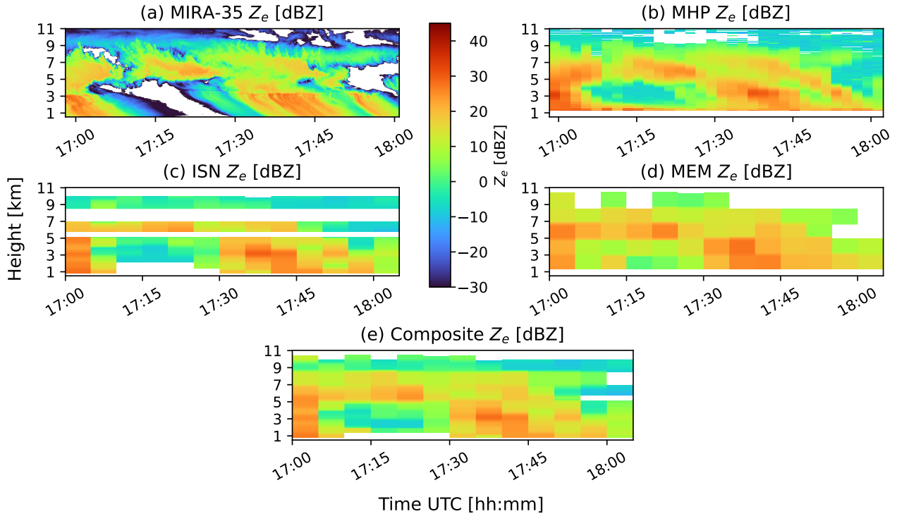
Figure 11. Measured radar reflectivity in vertical profiles of MIRA-35 (a), in extracted vertical profiles based on RHI scans of MHP (b), in BA-CVPs of ISN (c) and MEM (d) and as composite of ISN and MEM (e) collected on 08 July 2021 between 16:58 UTC and 18:01 UTC.
