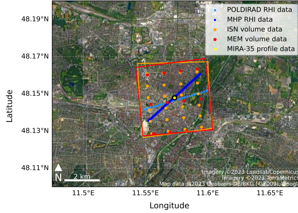
Figure 4. Map of the area of interest for this study. Shown is the metropolitan region of Munich as a zoom-in of the white rectangle in Fig. 3. The yellow dot marks the position of MIRA-35. Shown are the measurement points of the dedicated (blue colors) and operational radars (red and orange) within their respective segment of roughly 2 km x 2 km centered on MIRA-35 at the lowest elevation angle. The data of POLDIRAD is not directly above MIRA-35 with a very minor offset which is the result of the pointing error associated with the pointing accuracy of POLDIRAD. Imagery ©2023 Landsat/Copernicus, Imagery ©2023 TerraMetrics, Map data ©2023 Geobasis-DE/BKG (©2009), Google.
