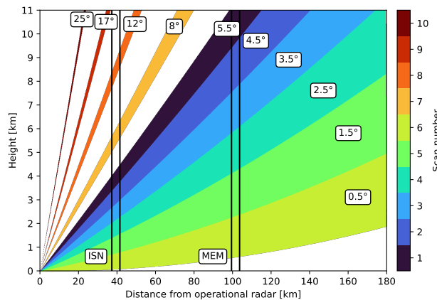
Figure 7. Scan strategy of the German operational radar network serviced by the DWD. Schematically shown are the ten PPI scans colored in order of execution with their respective elevation angles considering beam-broadening, earth curvature and refraction in earth's atmosphere. Black vertical lines mark the radial extent and position of the extracted BA-CVPS of ISN (at ca. 40 km) and MEM (at ca. 100 km) with regards to MIRA-35.
