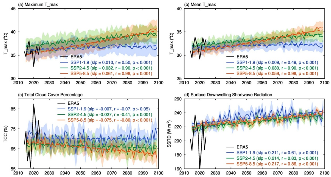
Figure 6 Trends of multi-model ensemble mean radiation conditions projected by the CMIP6 under three SSPs during 2015-2099. (a) The maximum daily T max , and (b) The mean daily T max in July, represent the extreme and mean status of high temperature, respectively. (c) TCC and (d) SSRD together reflect the solar radiation conditions for O 3 formation. The shading shows \pm 1.0 standard error, and the dash lines represent the linear trends of each variable under different SSPs. The black curve in each panel shows the real variation of each variable from the ERA5 reanalysis data during 2014-2024.
