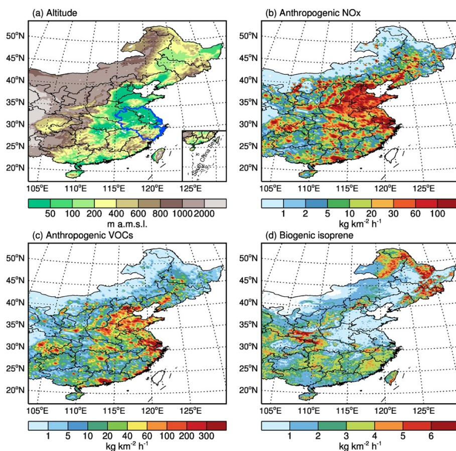
888 Figure 1 Location of the YRD, China and spatial distributions of emissions. (a) The 889 flat YRD is located in the eastern China, marked by the blue line. (b) Anthropogenic 890 NO x emission rate in July 2022 based on the MEIC emission inventory. (c) Same as (b), 891 but for anthropogenic non-methane VOCs. (b) and (c) represent human-induced 892 emissions of precursors for O 3 . (d) Biogenic isoprene emission rate is calculated by 893 MAGAN, representing biogenic VOCs emissions.
