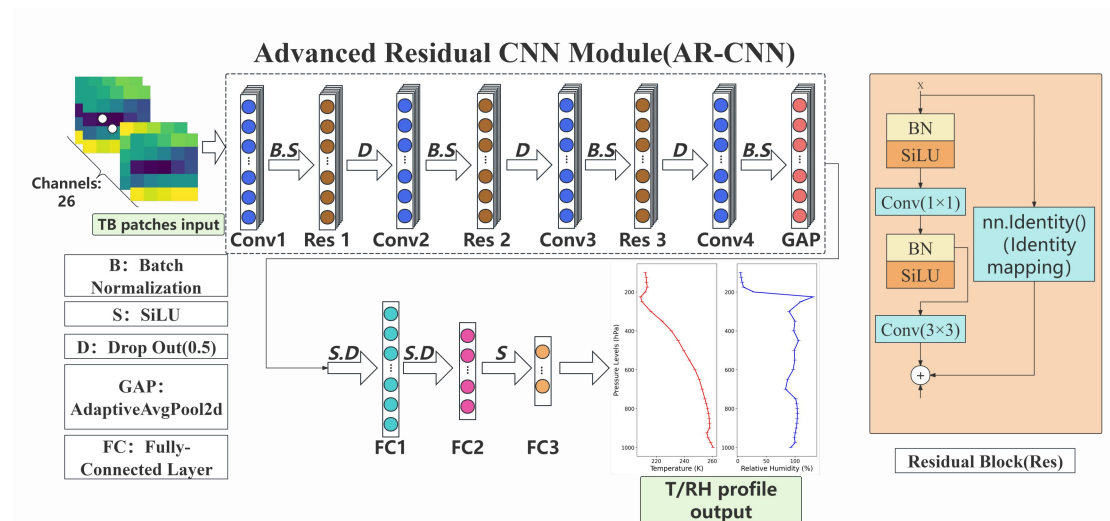
Figure 2: Network architecture for Advanced Residual CNN (AR-CNN)
