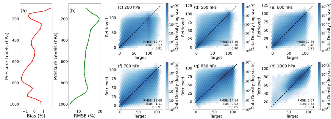
Figure 8: (a)-(b) Bias (%) and RMSE (%) of the retrieved RH profile; (c)-(h) Two-dimensional histograms of retrieved versus target RH at specific pressure levels. Color intensity indicates data density on a logarithmic scale, with darker colors representing higher data counts. The dashed black line ( y = x ) denotes the 1:1 reference for perfect agreement, and the Pearson correlation coefficient ( r ) quantifies the degree of linear consistency. (c) 200 hPa; (d) 500 hPa; (e) 600 hPa; (f) 700 hPa; (g) 850 hPa; (h) 1000 hPa.
