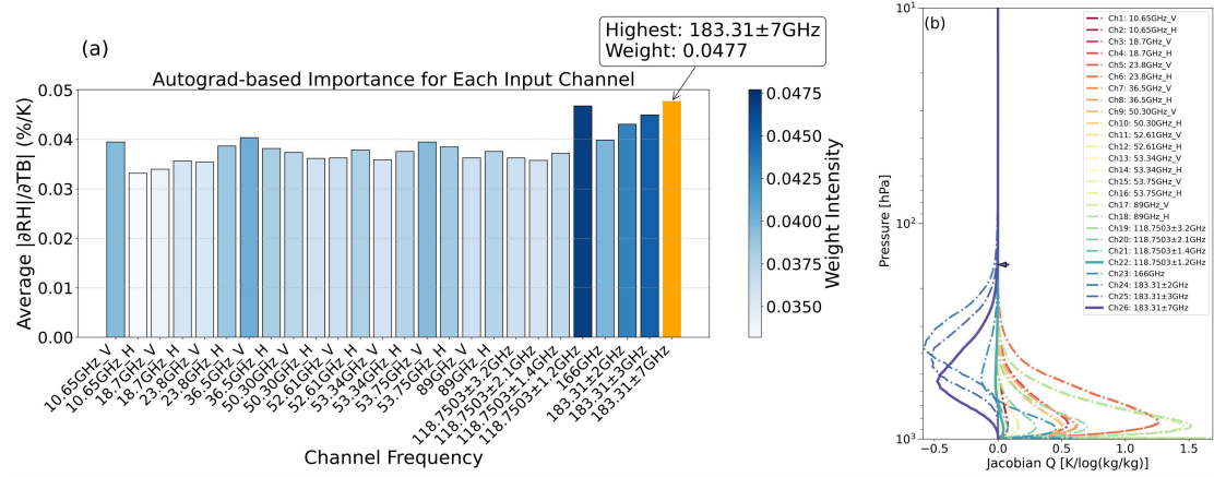
Figure 10: (a) Autograd-based sensitivity analysis of input channels for RH retrieval. The vertical axis represents the mean absolute normalized gradient ( |\partial RH/\partial TB| , % K -1 ); (b) Jacobian for relative humidity, obtained using the RTTOV model tailored for the MWRI-RM sensor. Solid lines denote Channel 22 (118.75±1.2 GHz) and 26 (183.31±7 GHz), while dash-dot lines represent other channels.
