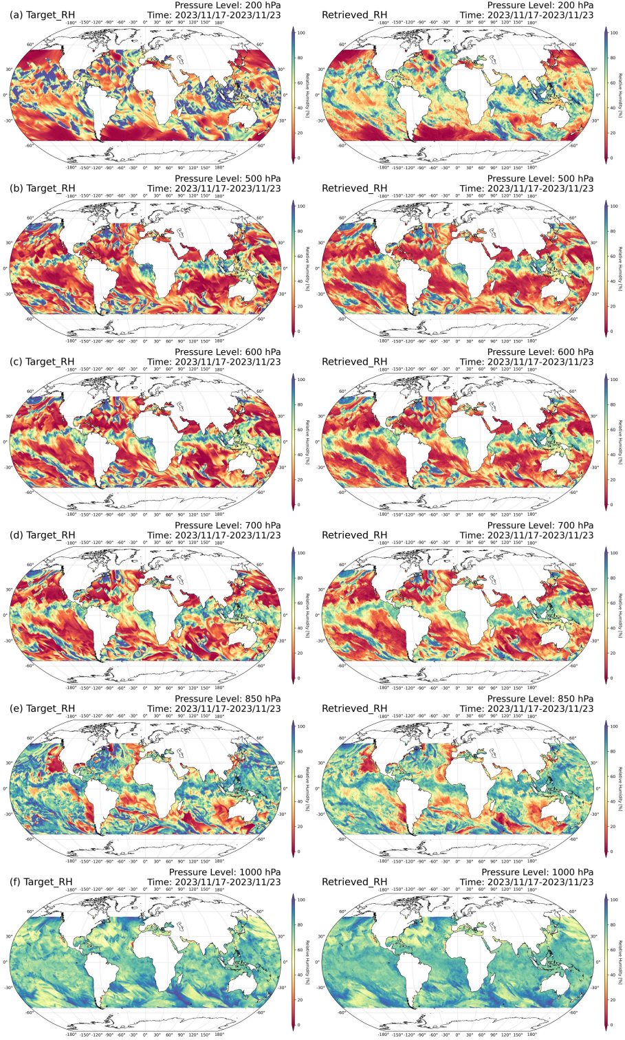
Fig. A2: Global Comparison Map of the Retrieved Relative Humidity at Specific Pressure Levels. (a)
