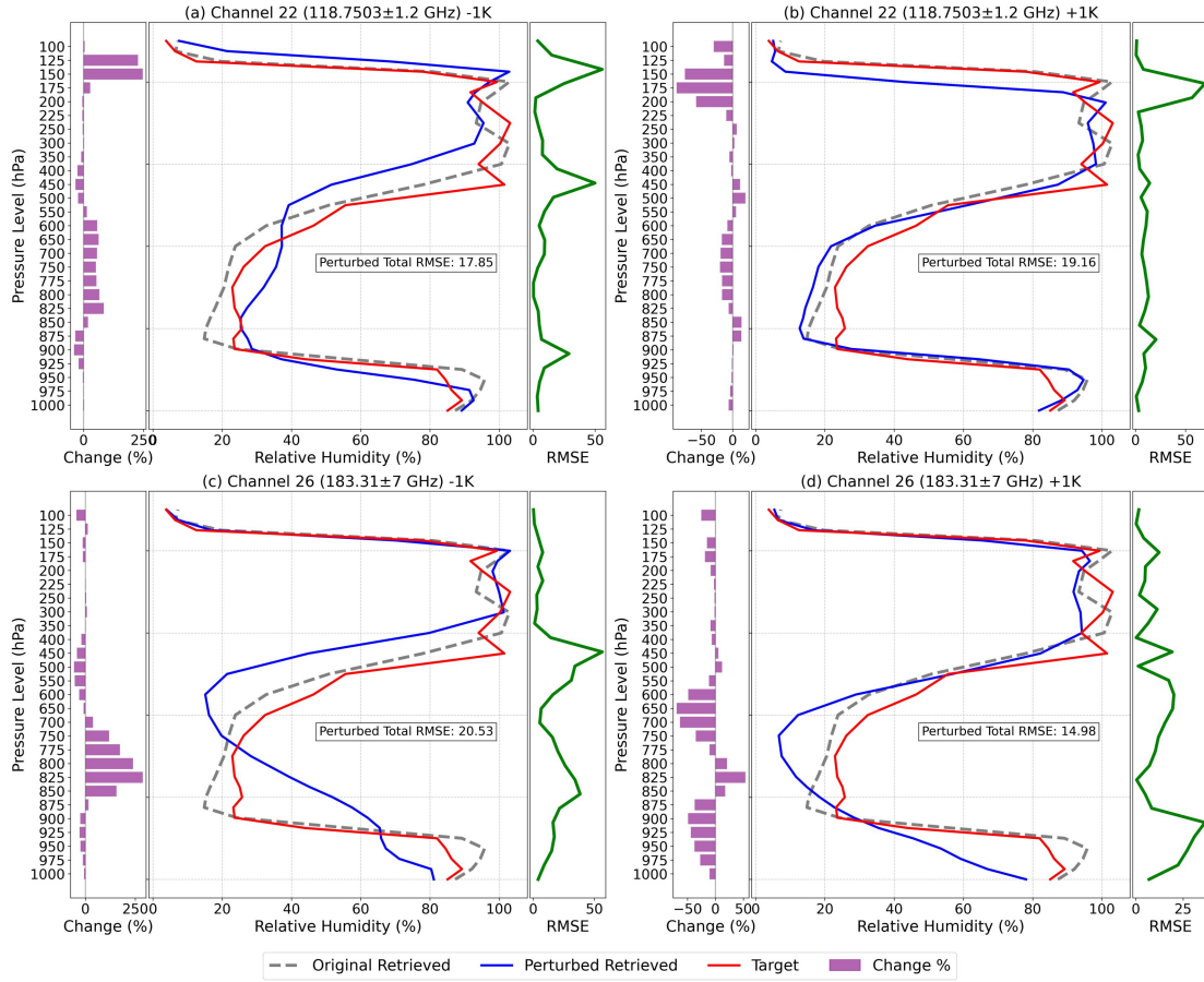
Figure 11: Single relative humidity profile perturbation experiment ( \pm 1\text{K} perturbations are introduced to the brightness temperatures of channels 22 and 26). Each subplot adopts a triple-axis composite layout: the left-hand purple bar chart reveals the vertical relative differences of the perturbed retrieval profile from the original profile (calculated as [(\text{perturbed} - \text{original})/\text{original}] \times 100\% ); the central area presents the relative humidity profiles comparison (gray dashed line denotes the original retrieval result, blue solid line represents the perturbed retrieval result, and red solid line is the target profile); the right-hand green curve signifies the vertical RMSE between the perturbed retrieval profile and the target profile.
