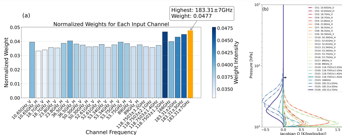
Figure 10: (a) Weighting map for RH profile retrieval channels; (b) Jacobian for relative humidity, obtained using the RTTOV model tailored for the MWRI-RM sensor. Solid lines denote Channel 22 (118.75±1.2 GHz) and 26 (183.31±7 GHz), while dash-dot lines represent other channels.
