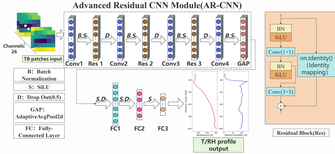
Figure 2: Network architecture for Advanced Residual CNN (AR-CNN)
