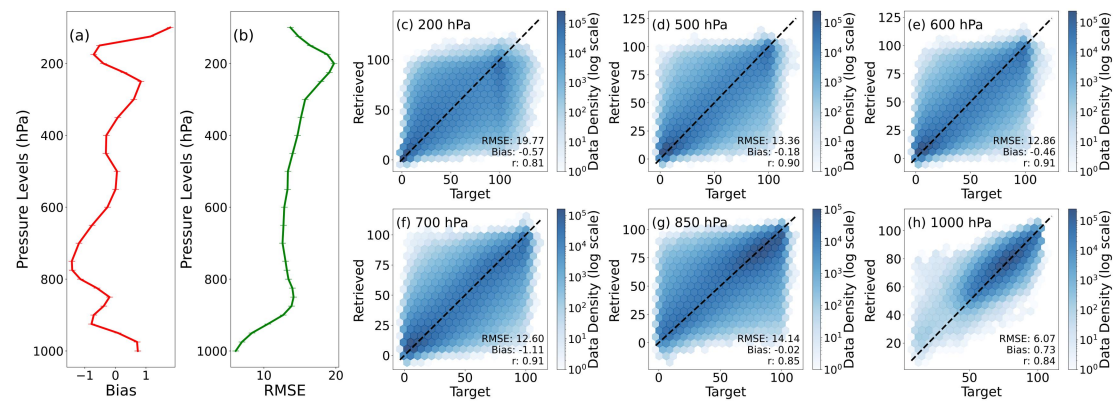
Figure 8: (a)-(b) Bias and RMSE of the retrieved RH profile; (c)-(h) Two-dimensional histogram of retrieved RH at specific pressure levels, where color intensity represents data point density (logarithmic binning). Darker colors indicate higher data counts in each bin, while lighter colors denote sparser distributions. A dashed black line ( y=x ) denotes the “1:1 consistency line” for perfect agreement between retrieved and target values. Pearson correlation coefficient ( r ) is shown for statistical assessment of linear agreement. (c) 200 hPa; (d) 500 hPa; (e) 600 hPa; (f) 700 hPa; (g) 850 hPa; (h) 1000 hPa.
