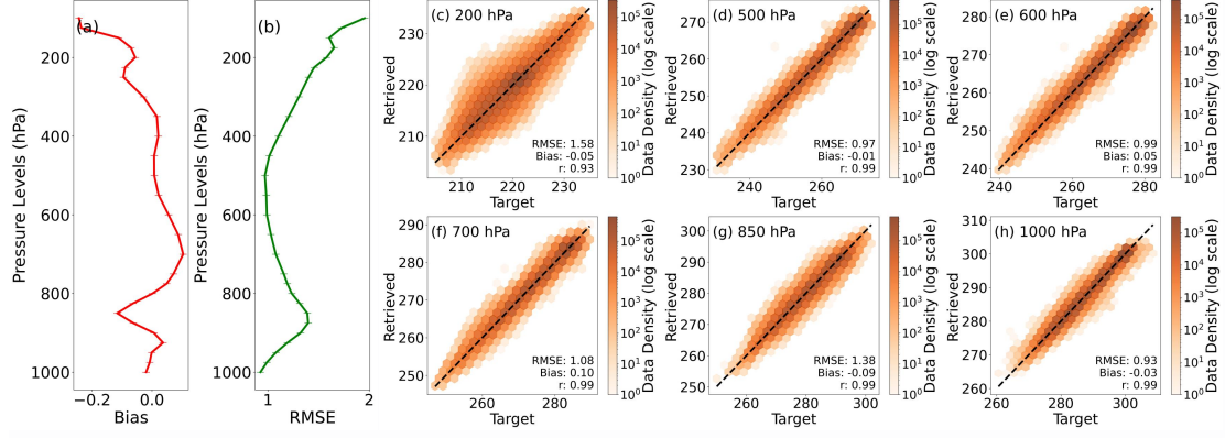
Figure 3: (a)-(b) Bias and RMSE of the retrieved temperature profile; (c)-(h) Two-dimensional histogram of retrieved temperature at specific pressure levels, where color intensity represents data point density (logarithmic binning). Darker colors indicate higher data counts in each bin, while lighter colors denote sparser distributions. A dashed black line ( y=x ) denotes the “1:1 consistency line” for perfect agreement between retrieved and target values. Pearson correlation coefficient ( r ) is shown for statistical assessment of linear agreement. (c) 200 hPa; (d) 500 hPa; (e) 600 hPa; (f) 700 hPa; (g) 850 hPa; (h) 1000 hPa.
