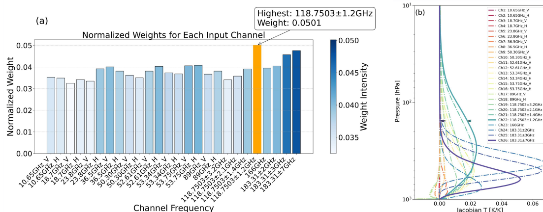
Figure 5: (a) Weighting map for temperature profile retrieval channels; (b) Jacobian for temperature, obtained using the RTTOV model tailored for the MWRI-RM sensor. Solid lines denote Channel 22 ( 118.75 \pm 1.2 GHz) and 26 ( 183.31 \pm 7 GHz), while dash-dot lines represent other channels.
