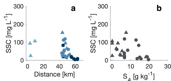
Figure 10. Suspended sediment concentration (SSC) versus distance from the glacier (a), and (b) the surface salinity. Data points with salinities in the intervals: <1 , 1-13 and >13 \text{ g kg}^{-1} are shown with colors, where lower salinity is shown in lighter blue and higher salinity in darker blue. Samples taken at the surface (triangles) and at 1 m depth (circles) are indicated. Note that no SSC samples were taken between 10 and 40 km from the ice margin.
