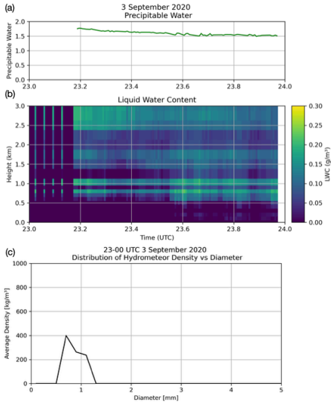
Figure 16: Additional observations of precipitable water and liquid water content from the MWR and hydrometeor size distribution from the PIP on 3 September 2020 (a) precipitable water content (b) liquid water content (c) distribution of hydrometeor density vs. diameter. Note the different y-axis scale in panel (c) compared to Fig. 12.
