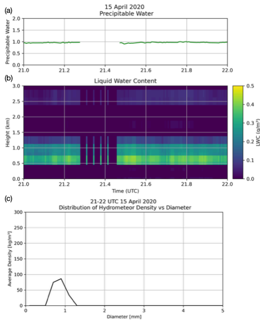
Figure 12: Additional observations of precipitable water and liquid water content from the MWR and hydrometeor size distribution from the PIP on 15 April 2020 (a) precipitable water content (b) liquid water content (c) distribution of hydrometeor density vs. diameter.
