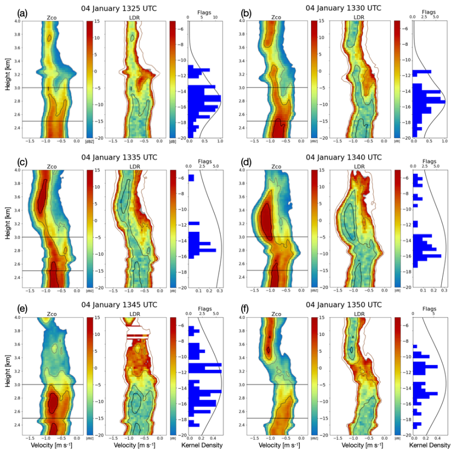
510 Figure 18: As in Figure 10, with spectrograms taken at 2.5 and 3.0 km, for 4 January 2022 at (a) 1325 UTC, (b) 1330 UTC, (c) 1335 UTC, (d) 1340 UTC, (e) 1345 UTC, (f) 1350 UTC.
