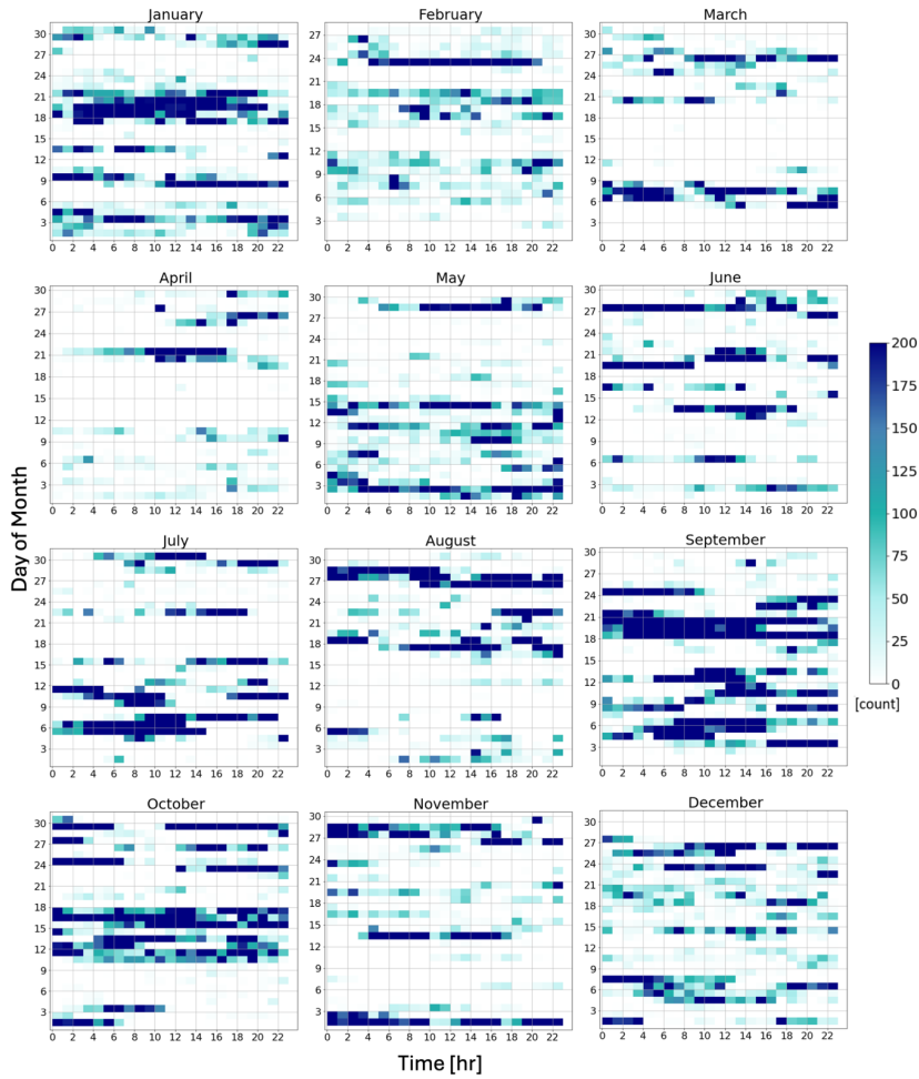
580 Figure A2: As in Figure 4, but for 2023. Results from July 2023 are displayed because vertically pointing moment data was available, but note that the spectra from this month was not available for verification.
