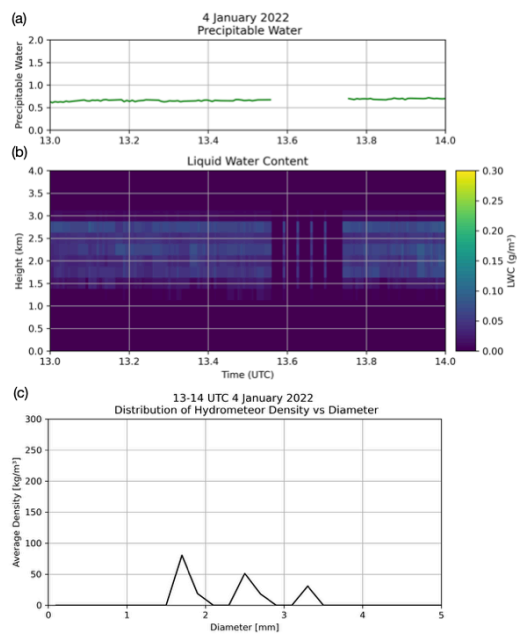
530 Figure 20: Additional observations of precipitable water and liquid water content from the MWR and hydrometeor size distribution from the PIP on 4 January 2022 (a) precipitable water content (b) liquid water content (c) distribution of hydrometeor density vs. diameter.
