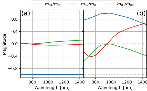
Figure 3. Non-ideal polarimetric response of ALI (Letros et al., 2024) is shown as normalized coefficients of the first row of the Muller matrix, which dictates the measured Stokes parameter I' . Plot (a) is the response of the LCR on state. Plot (b) is the response of the LCR off state. The coefficient of m_{01}/m_{00} shows the proportional transference of Q_{\text{atmo}} into I' . Likewise, m_{02}/m_{00} and m_{03}/m_{00} show the same for U_{\text{atmo}} and V_{\text{atmo}} respectively. An ideal ALI response would have m_{01}/m_{00} = -1 in the LCR on state, m_{01}/m_{00} = 1 in the LCR off state, as well as m_{02}/m_{00} = 0 and m_{03}/m_{00} = 0 for both cases - i.e. purely vertical linear polarization with the LCR on, and purely horizontal linear polarization with the LCR off.
