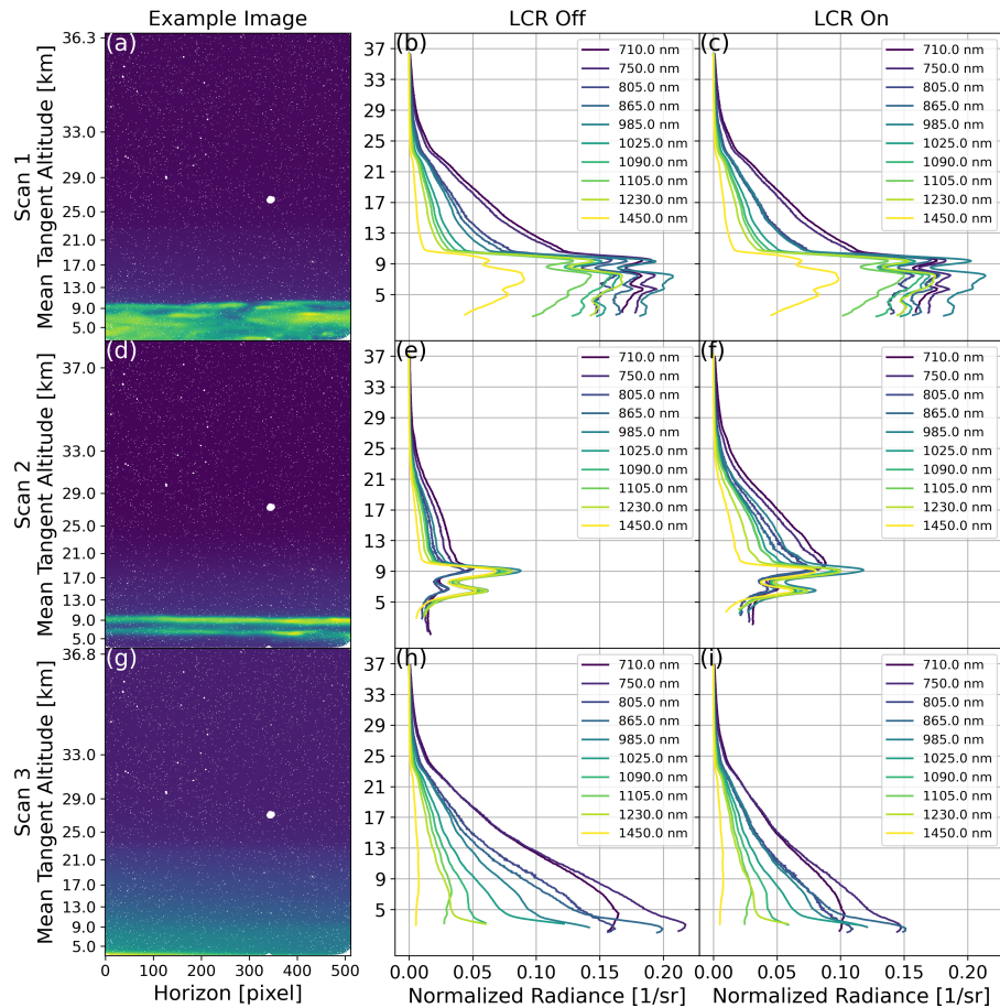
Figure 5. Observations of all three ALI scans used in the present work. Panels (a, b, c) are Scan 1 observations, (d, e, f) are Scan 2 observations, and (g, h, i) are Scan 3 observations. Panels (a, d, g) are example images from the three different scans taken at 1230 nm with the LCR off. Panels (b, e, h) are radiance profiles of different wavelengths with the LCR off (horizontally dominate polarization), and panels (c, f, i) are radiance profiles of different wavelengths with the LCR on (vertically dominate polarization).
