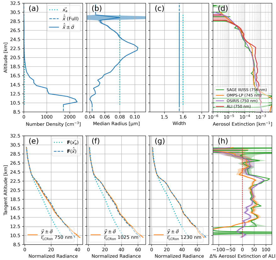
Figure 18. Aerosol retrieval of Scan 3 (horizontally dominate polarization). Descriptions of (a, b, c, d, e, f, g, h) same as Fig. 16.
