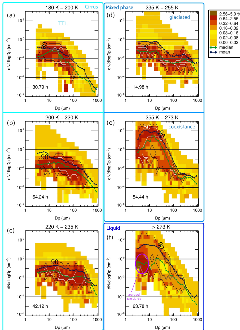
Figure 6. Heat maps of cloud particle size distributions (PSDs) in their respective temperature ranges; (a-c): cirrus clouds between 180-235 K ( \sim -90 to -38^{\circ}\text{C} ), (d-e): mixed-phase clouds between 235-273 K ( -38 to 0^{\circ}\text{C} ) and (f): liquid clouds for >273 K ( > 0^{\circ}\text{C} ). Mixed-phase and cirrus clouds are divided into sub-ranges, the coldest temperature range represent the tropical tropopause layer (TTL). Green/black lines: median/mean PSDs; solid black/white contour lines enclose regions containing 90/50% of the data points. The dataset contains 137.2 hours in ice clouds, 69.4 hours in mixed clouds and 63.8 hours in liquid clouds; the measurements hours in the temperature ranges are indicated in each panel.
