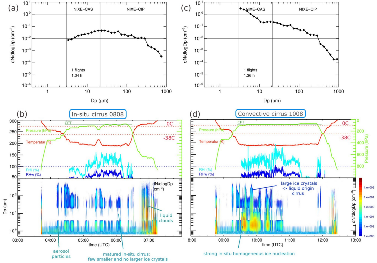
Figure 1. Cirrus PSDs: (a) and (c) mean PSDs, (b) and (d) PSDs along aircraft flights, for two flights during the StratoClim campaign in 2017 out of Nepal. ( D_p > 3 \mu\text{m} is D_{\text{ice}} ).
