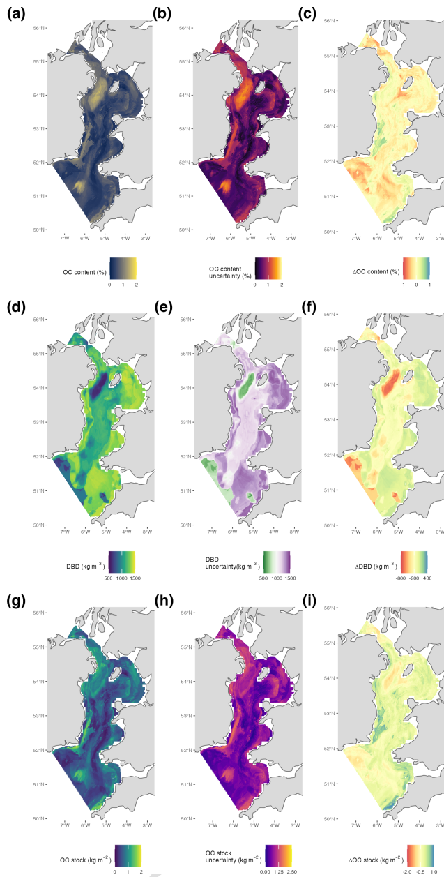
Figure 6. (a) Predicted organic carbon (OC) content using adjusted model inputs; (b) the associated uncertainty and (c) difference between not bias adjusted and bias adjusted predictions across the study area (difference = OC_{content,pre} - OC_{content,post} ); (d) Predicted dry bulk density (DBD) content using adjusted model inputs; (e) the associated uncertainty and (f) difference between DBD modelled from porosity and using an RF ( DBD_{adj} - DBD_{unadj} ); (g) Predicted organic carbon (OC) stock using adjusted model inputs; (h) the associated uncertainty and (i) difference between not bias adjusted and bias adjusted predictions across the study area (difference = OC_{stock,unadj} - OC_{stock,adj} ). Negative values in panels (c), (f), and (i) indicate where predictions with adjusted model inputs were higher than non-bias adjusted inputs.
