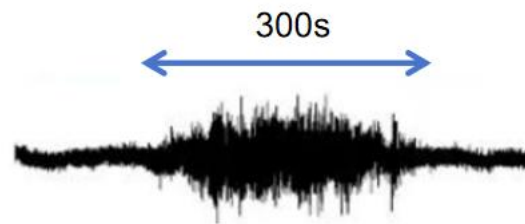
Figure 4: Seismic signal for 2018 Sedongpu detachment
