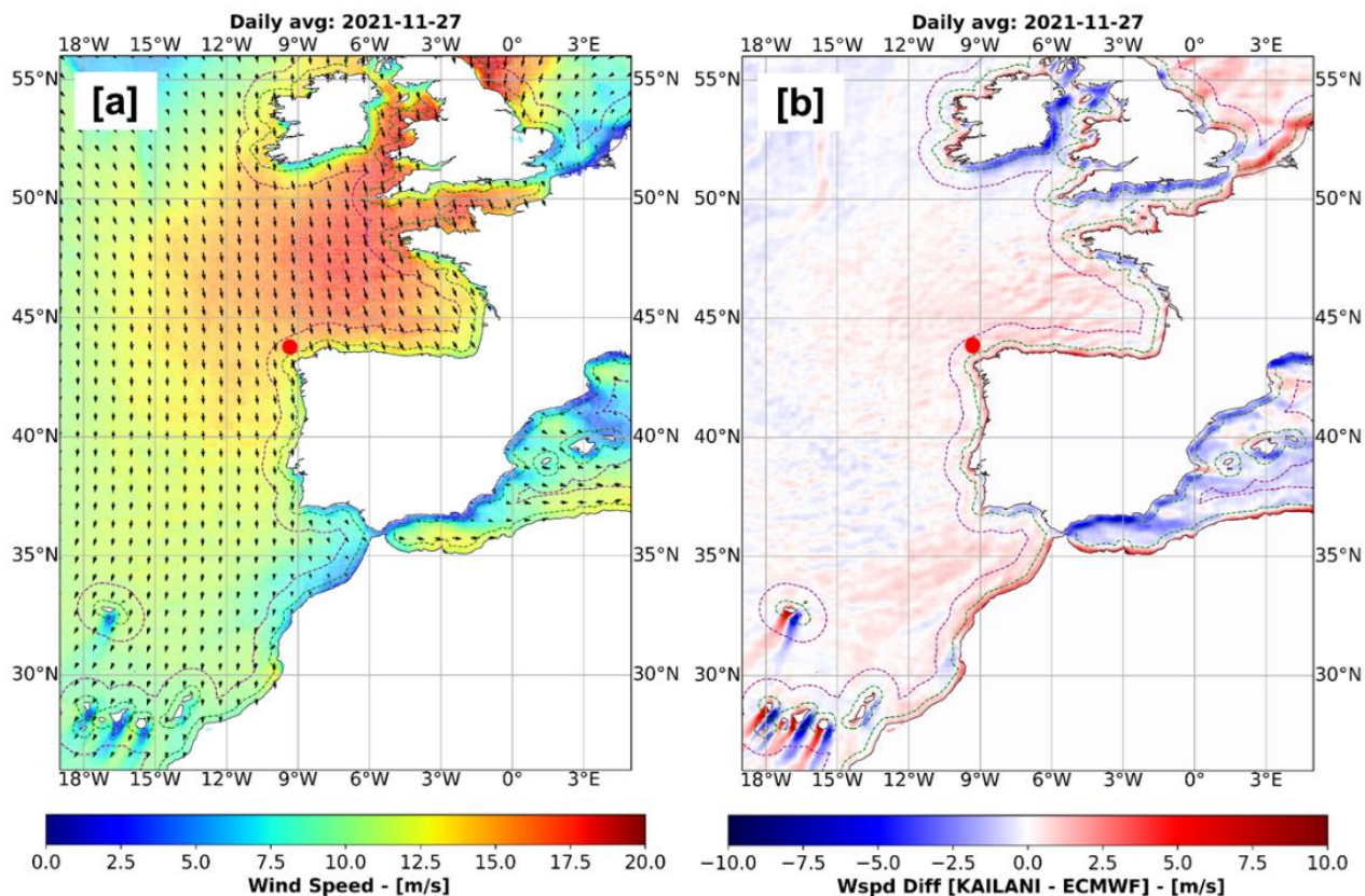
545 Figure 12: (Left) ANN-generated daily-averaged wind fields during the November 2021 event (storm peak, on 2021-11-27). The coloured areas the wind speed in m/s and the black arrows the wind vectors. (Right) Difference between KAILANI minus ECMWF-IFS daily-averaged wind speed. Units in m/s. White to red means that KAILANI predicts higher speeds than ECMWF-IFS; whilst white to blue refers that KAILANI predicts lower speeds. The red dot is the GAL-D buoy (see Fig. 13).
