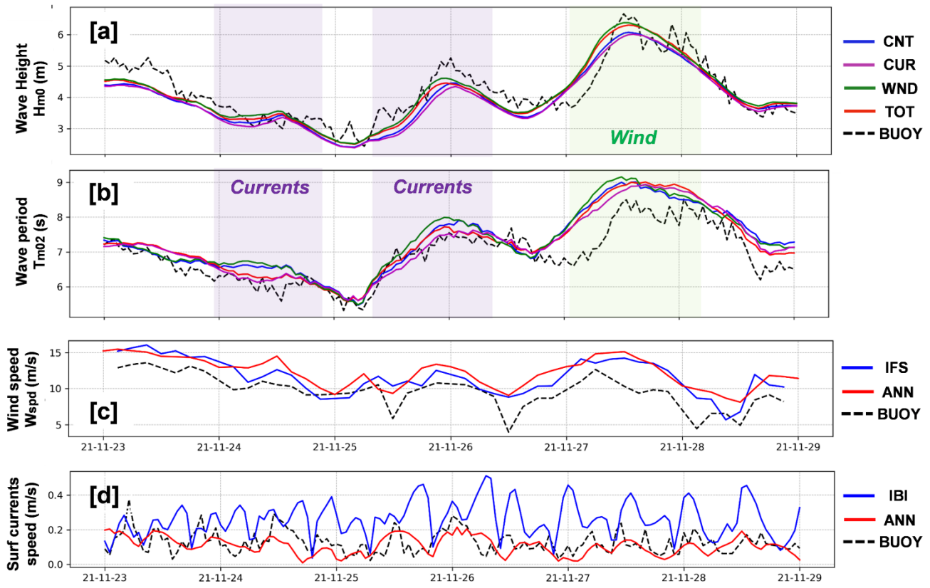
550 Figure 13: Time series of the performance of the wave parameters and their associated forcings at GAL (Villano Buoy) under the November 2021 event. [a] H_{m0} of the different experiments (see Table 2) vs the buoy. [b] Same as [a], but for the T_{m02} . The shaded time slices highlight good performance of the enhanced forcings, and the colour hints the main factor (be it wind [green] or currents [purple]). [c] Wind speed predicted by ECMWF-IFS (blue), the wind ANN (red) and the buoy measurements (dashed line). [d] Surface current speed predicted by IBI-PHY (blue), the currents ANN (red) and the buoy (dashed line).
