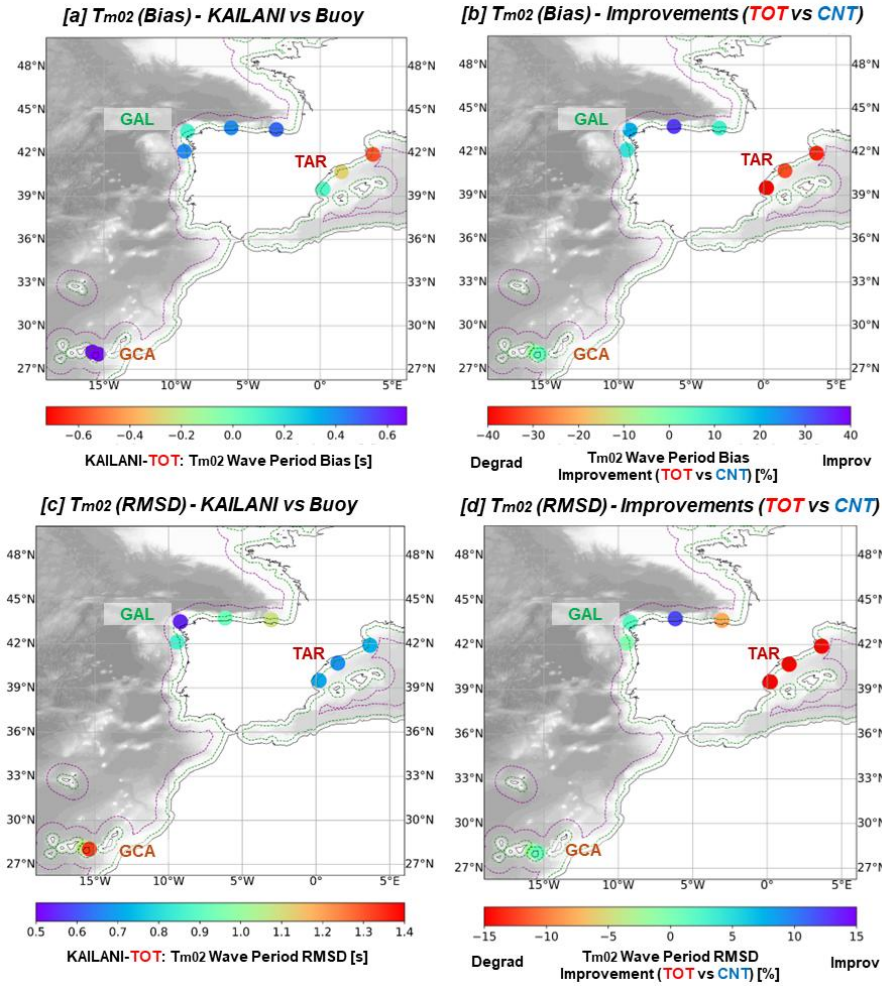
535 Figure 11: Integrated T m02 error metrics for the whole simulation period (2021/10 - 2022/01). Left panels [a,c] show the Bias and RMSD at the TOT experiment. Right panels [b,d] the % of improvement of the same metric from the left (TOT respect the control CNT test). “Improv” (green to purple) means improvement of the TOT respect CNT; whereas “Degrad” (green to red) means degradation of the prediction. Points closed to each pilot site buoy, are in-situ buoys.
