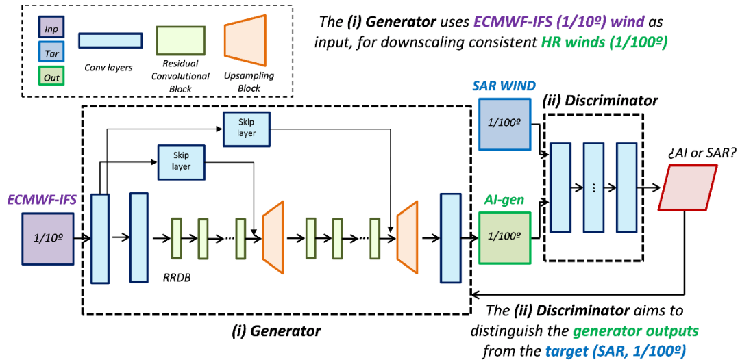
Figure 2: Generative Adversarial Network (GAN) for Wind Forecast that consists of two parts: (i) a Generator that uses ECMWF-IFS data (purple box) for building 1/100^\circ images (green box), trying to mimic SAR Wind data (blue box), and (ii) a Discriminator (that predict the likelihood that a given image is a true SAR Wind, or rather an AI-generated image).
