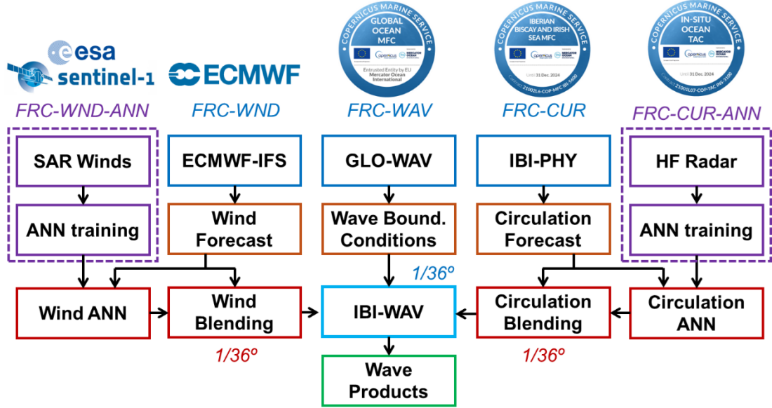
Figure 1: Flowchart of the proposed upgrades of the KAILANI project for the IBI-WAV operational chain. Note that ANNs training is conducted outside (and offline) the operational chains.
