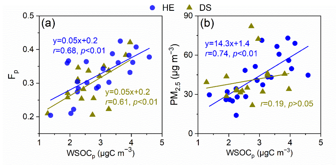
111 Figure S2. Linear regression analysis for WSOC p with (a) partitioning coefficient of 112 WSOCs ( F_p ) and (b) PM 2.5 during the haze event (HE) and dust storm (DS) event, 113 respectively
