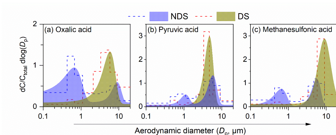
Figure S6. Size distribution of (a) oxalic acid, (b) pyruvic acid and (c) methanesulfonic acid during the non-dust storm (NDS) and dust storm (DS) events in Shanghai. The dashed lines and filled areas are the measured size distribution and fitting results, respectively. C_{total} is the sum of concentration on all the 9-stages.
