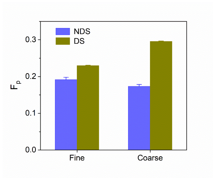
Figure S7. The partitioning coefficients ( F_p ) of WSOCs in the fine ( <2.1\mu\text{m} ) and coarse ( >2.1\mu\text{m} ) in the non-dust storm (NDS) and dust storm (DS) periods in Shanghai during spring of 2023.
