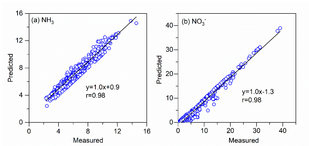
102 Figure S1. Comparison of measured ammonia and nitrate and predicted by ISORROPIA- 103 II model.
