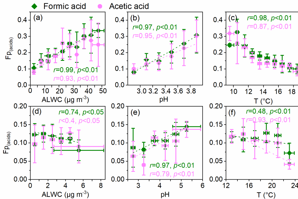
124 Figure S4. Factors affecting the gas-to-particle partitioning coefficients of formic and 125 acetic acids in (a-c) HE and (d-f) DS periods in spring 2023 in Shanghai.
