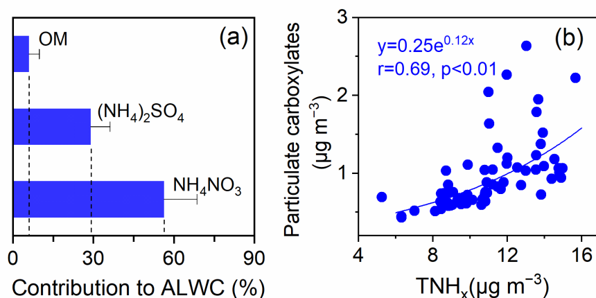
118 Figure S3. (a) Contributions of \text{NH}_4\text{NO}_3 , (\text{NH}_4)_2\text{SO}_4 and OM to ALWC in the haze 119 event (HE); (b) Particulate carboxylates as a function of \text{TNH}_x in the haze event (HE).
