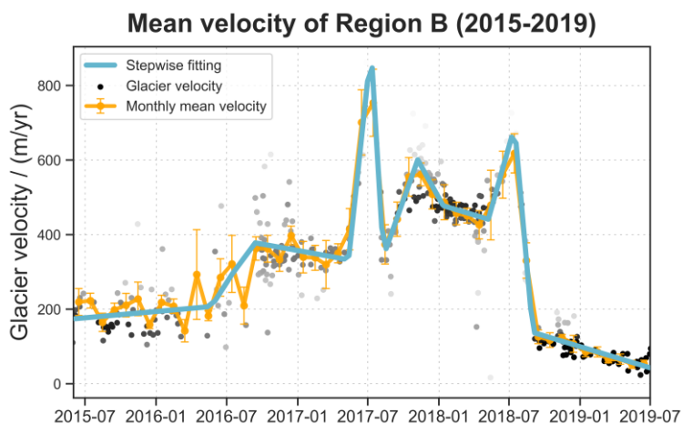
Figure 12: Glacier velocity time series for Regions B (2015 – 2019). The orange line represents monthly mean glacier velocity, while the cyan line denotes velocity change trends. Each grey dot corresponds to an individual velocity observation, with darker colours indicating more observations at that position.
