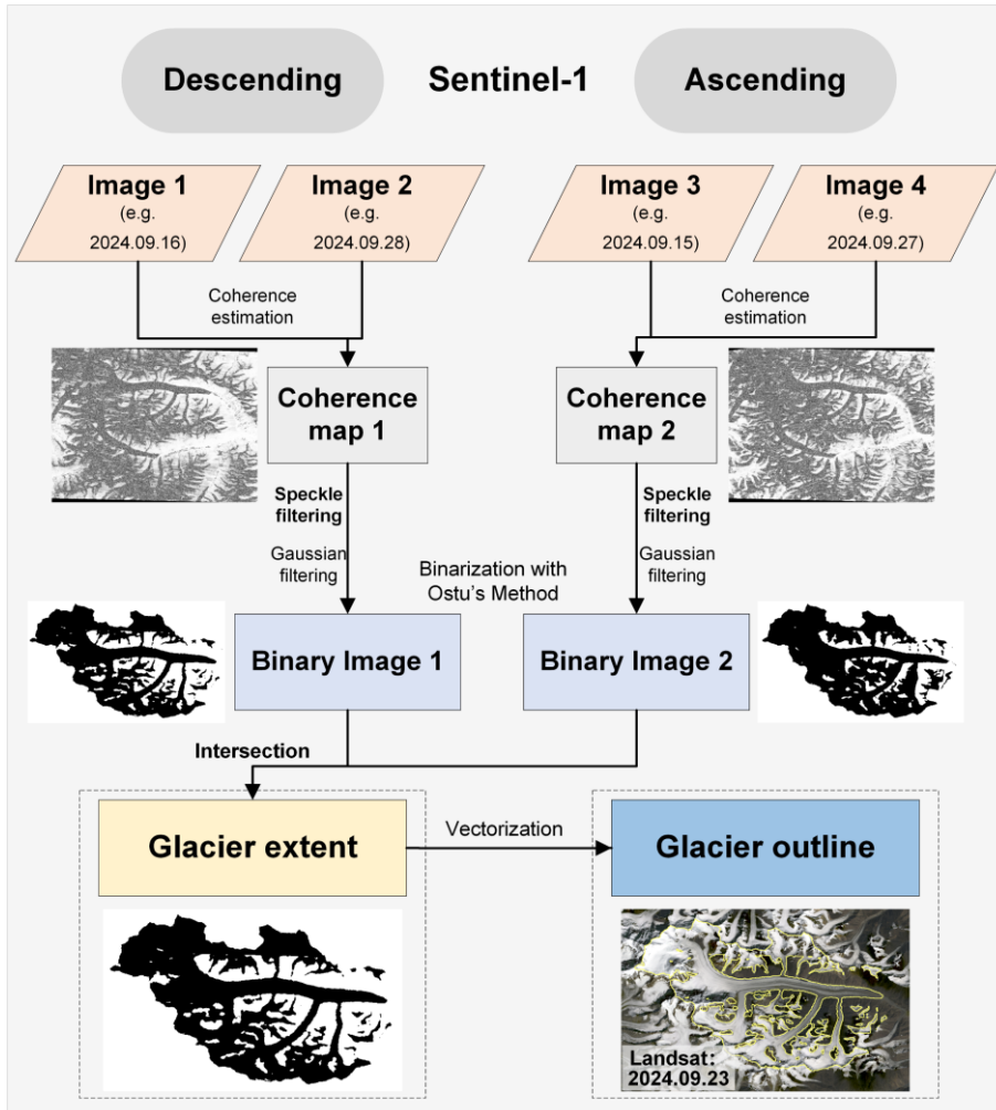
235 Figure 3: Flowchart for extracting glacier outlines using Sentinel-1 SLC images. The base map of the glacier outline is a Landsat 8 image acquired on September 23, 2024.
