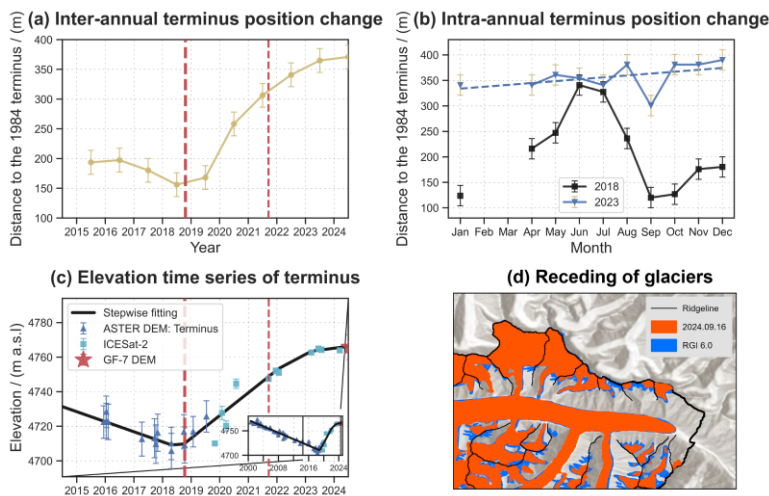
420 Figure 8: Terminus position and surface elevation changes over time. (a) Inter-annual terminus position changes derived from Sentinel-1 imagery; (b) Intra-annual terminus position variations derived from Sentinel-1 imagery; (c) Surface elevation time series at the glacier terminus, with the lower right subfigure displaying elevation changes from 2000 to 2024; (d) Glacier recession of NKG I, where blue represents the glacier extent derived from the RGI 6.0 inventory (August 2, 2002) and red depicts its configuration as of September 16, 2024. 425 For panels (a) and (b), since the glacier length in 1984 was shorter than in all subsequent years after 2000, the glacier termini extracted from Sentinel-1 images (2015–2024) are all ahead of the 1984 terminus. Therefore, an increase in distance from the 1984 terminus indicates glacier advance, while a decrease in distance indicates glacier retreat. The base map in panel (d) is derived from ESRI World Hillshade (Credit: ESRI, NASA, NGA, USGS).
