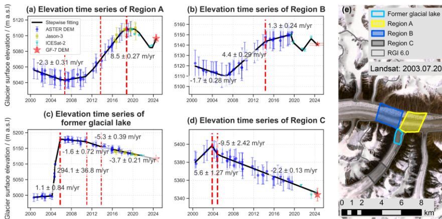
380 Figure 6: Glacier surface elevation time series of Regions A, B, C, and the former glacial lake from 2000 to 2024. (a)–(d) Black lines indicate elevation change trends, with each dot representing an individual elevation observation. Vertical red lines mark transition points in elevation change patterns. (e) Locations of Regions A, B, C, and the former glacial lake. The base map in panel (e) is a Landsat 7 image acquired on July 20, 2003.
