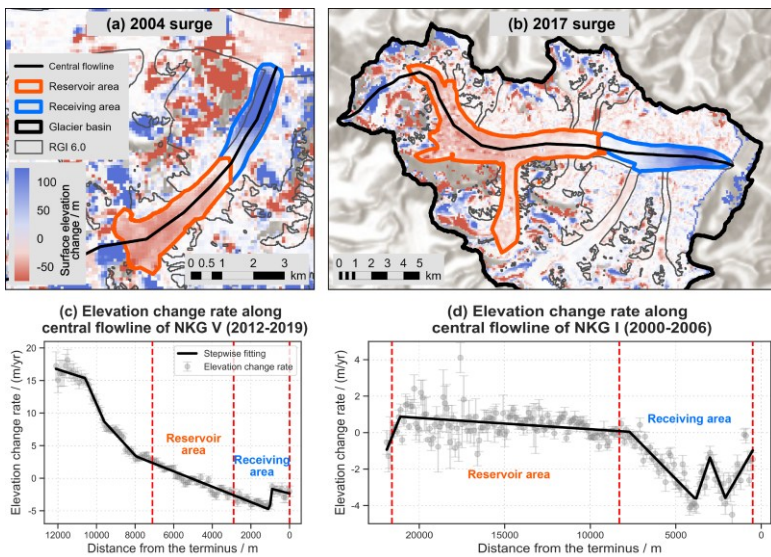
505 Figure 11: Glacier elevation changes during surges and elevation change rates along central flowlines during stable periods. (a) Elevation changes of NKG V between 2002 and 2006; (b) Elevation changes of NKG I between 2015 and 2019; (c) Elevation change rates along the central flowline of NKG V during the period (2012–2019); (d) Elevation change rates along the central flowline of NKG I during the period (2000–2006). The areas between the vertical dashed lines in (c) and (d) correspond to the reservoir and receiving areas shown in (a) and (b). The base map in panel (b) is derived from ESRI World Hillshade (Credit: ESRI, NASA, NGA, USGS).
