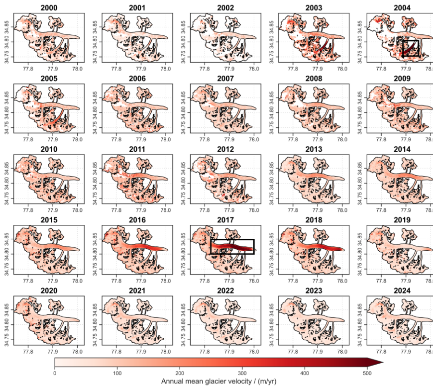
Figure 4: Annual mean velocities of NKG I from 2000 to 2024. Darker colours indicate higher velocities. The two black rectangles highlight the extents of the identified glacier surges, showing where velocities increased by 20-fold (2004) and 5-fold (2017) of magnitude over quiescent rates ( \sim 50 m/yr in 2023). Glacier outlines are derived from RGI 6.0, with NKG V manually connected to NKG I.
