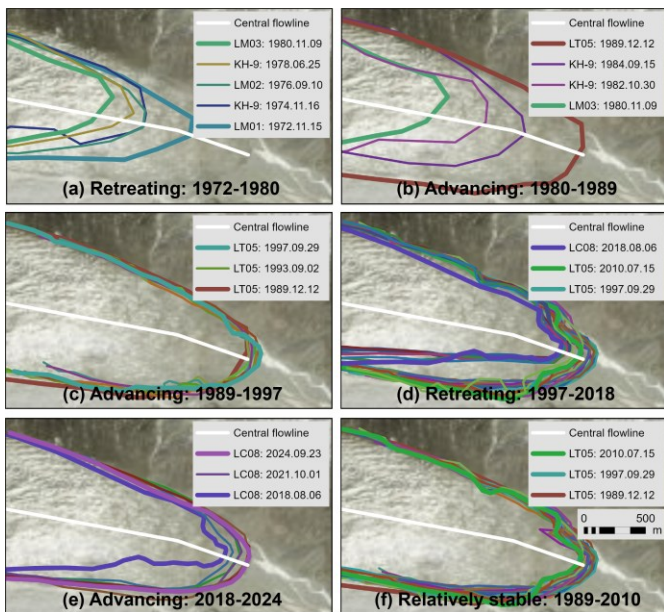
450 Figure 9: Temporal evolution of the NKG I terminus position from 1972 to 2024. (a) Terminus retreat from 1972 to 1980; (b) Rapid terminus advance between 1980 and 1989; (c) Slow terminus advance from 1989 to 1997; (d) Terminus retreat from 1997 to 2018; (e) Terminus advance from 2018 to 2024; and (f) Period of relative terminus stability between 1989 and 2010. Coloured lines represent terminus positions and morphological changes at different time steps. The base maps in panels (a)–(f) are derived from ESRI World Imagery and 455 Hillshade (Credits: ESRI, NASA, NGA, USGS, Maxar).
