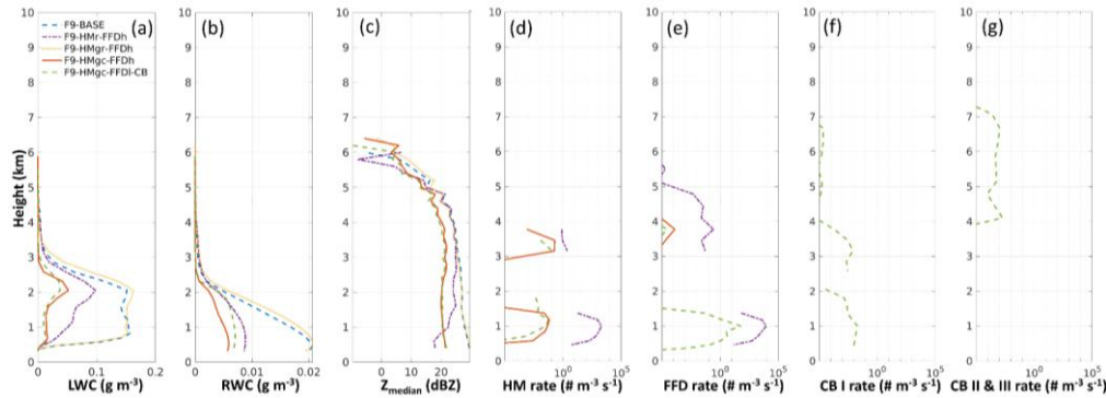
Figure 6. Profiles from the baseline and SIP simulations on 2019-02-07. (a): mean LWC, (b): mean RWC, (c): median radar reflectivity ( Z_{\text{median}} ), (d): mean Hallett-Mossop rate, (e): mean Fragmentation of Freezing Drop rate, (f): ice-ice collisional
