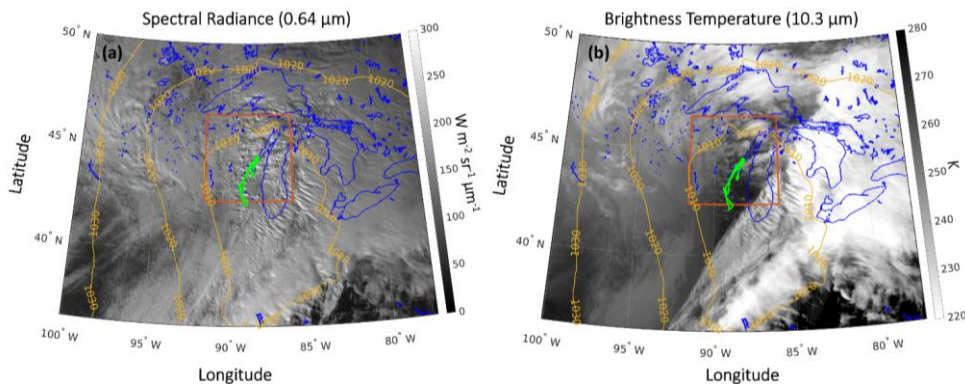
Figure 2. (a) GOES-16 spectral radiance at 0.64 \mu\text{m} (Channel 2). (b) GOES-16 brightness temperature at 10.3 \mu\text{m} (Channel 13). Both images are from 20:30 UTC on 9 February 2019. Blue lines denote coastlines and lakes; the red rectangle indicates the inner-most simulation domain (with a 0.25 km grid spacing) for Flight 9; yellow lines show the sea level pressure isobar at 18:00 UTC from the operational regional analysis used at ECCC; green lines: aircraft flight track. (Only data from the flight segments in the northern portion of the track were used in this study).
