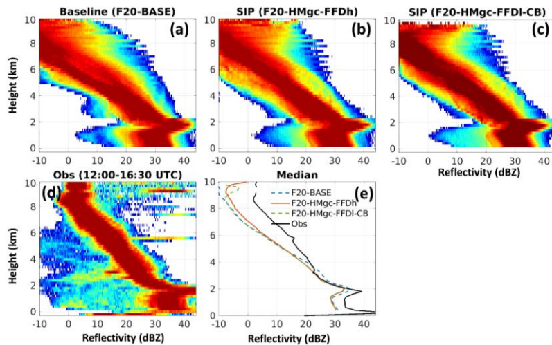
Figure 19. Similar to Figure 9 but for ICICLE Flight 20. The simulation data at 14:30 UTC on 2019-02-23 are used. The observation data from Flight 20 between 12:00 and 16:30 UTC are used.
