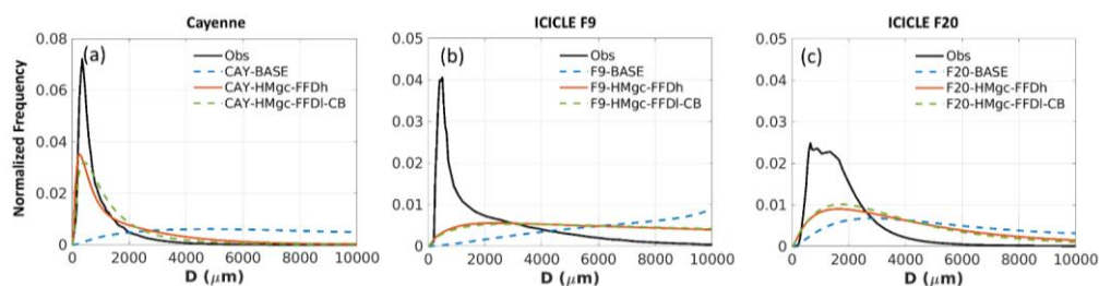
Figure 22. Ice particle mass distribution for HAIC-HIWC 2015 campaign near French Guiana (a), ICICLE Flight 9 (b), Flight 20 (c) for the temperature between -15^{\circ}\text{C} and -5^{\circ}\text{C} . Blue dashed lines: baseline simulation (BASE). Red lines: SIP (HMgc-FFDh) simulation. Green dashed lines: SIP (HMgc-FFDI-CB). Black lines: observation.
