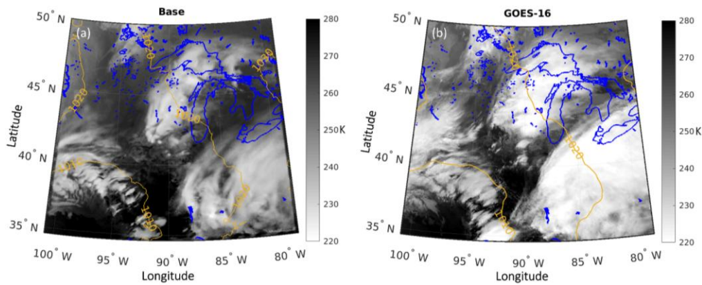
Figure 14. Similar to Figure 4 but for ICICLE Flight 20 on 23 February 2019 at 14:30 UTC. The yellow lines in panel b indicate the sea-level pressure from ECCC's operation regional prediction at 14:30 UTC initiated at 12:00 UTC.
