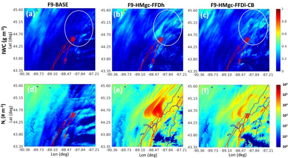
Figure 10. Averaged values between altitude of 0.5 and 3.8 km for Flight 9. (a), (b), (c): IWC; (d), (e), (f): N_i . First column for F9-BASE, middle column for F9-HMgc-FFD, third column for F9-HMgc-FFDI-CB. Red line: flight track.
