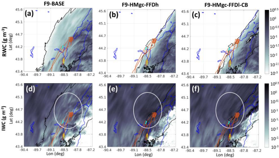
Figure 11. RWC (a, b, c) and IWC (d, e, f) near the surface for F9-BASE (a, d), F9-HMgc-FFDh (b, e) and F9-HMgc-FFDI-CB (c, f) simulations at 20:30 UTC on 2019-02-07. Black contour: region of freezing rain ( RWC > 0.01 \text{ g m}^{-3} and T < 0^\circ\text{C} in the lowest model layer at \sim 20 \text{ m} above surface). Red lines: Flight 9 aircraft track. Yellow lines: part of flight track below 800 m of altitude observing both supercooled liquid and ice near 20:12 UTC. Turquoise lines: part of flight track below 800 m of altitude observing only ice near 20:47 UTC.
