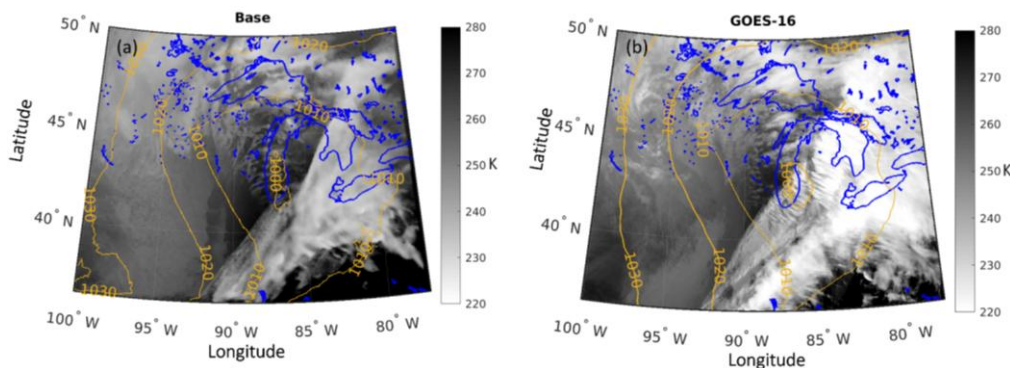
Figure 4. (a) Brightness temperature at 10.3 \mu\text{m} simulated using RTTOV (Saunders et al., 2018) with the BASE simulation at 2.5 km resolution for 20:30 UTC on 9 February 2019. (b) Observed brightness temperature from GOES-16 for 20:30 UTC on 9 February 2019. Blue lines indicate lake boundaries, while yellow lines represent sea-level isobars: from the F9-BASE simulation at 20:30 UTC in panel (a) and from ECCC's regional prediction model at 20:30 UTC initiated at 18:00 UTC in panel (b).
