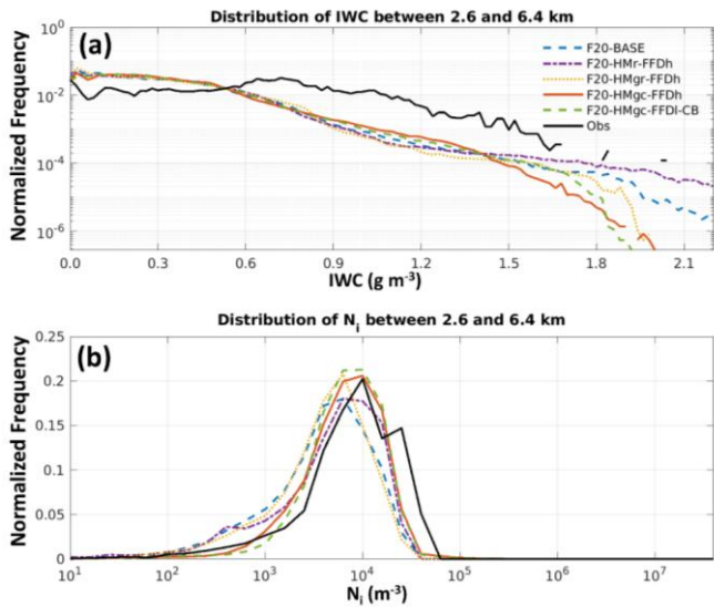
530 Figure 17. Same as Figure 7 but for simulations at 14:30 UTC on 2019-02-23 and observation data from ICICLE Flight 20 between 12:30 and 16:00 UTC. The altitude range is between 2.6 and 6.4 km.
