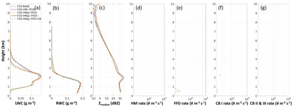
Figure 16. Same as Figure 6 but for ICICLE Flight 20 on 2019-02-23. The profiles are calculated based on simulation data at 510 min (14:30 UTC).
