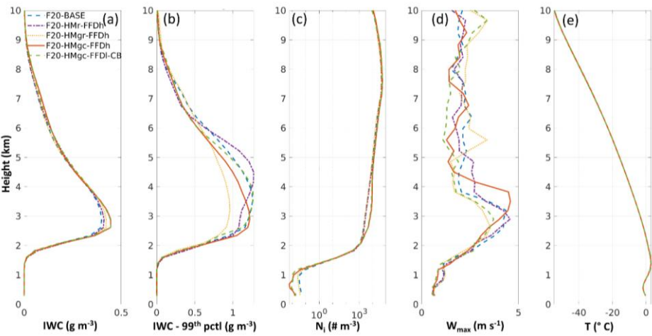
Figure 15. Same as Figure 5 but for ICICLE Flight 20 on 2019-02-23. The profiles are calculated based on simulation data at 510 min (14:30 UTC).
