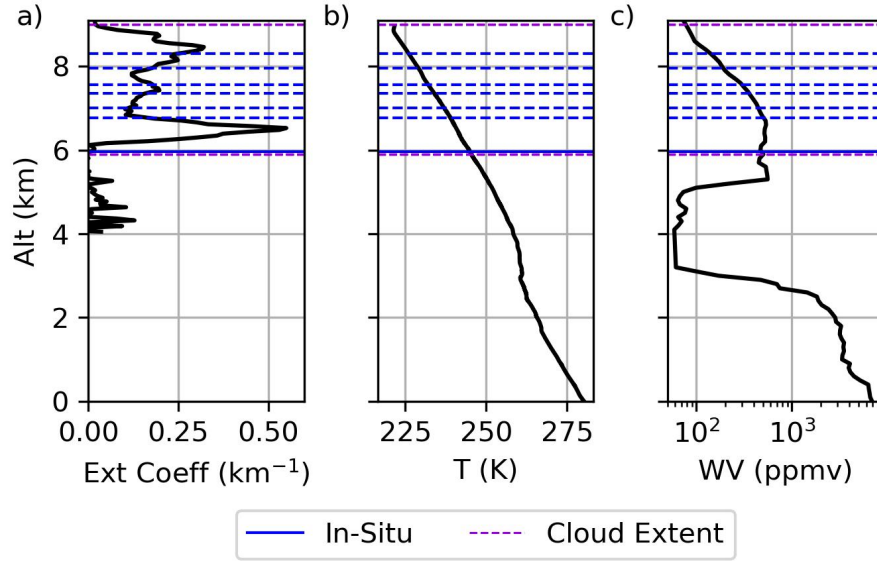
Figure 2. (a) The lidar-derived extinction coefficient of the cloud measured at 09:48:35 UTC. The (b) temperature and (c) water vapour profiles measured by dropsonde 1 at 09:47:48 UTC. The edges of the cloud extent are marked in purple, and the altitudes at which in-situ measurements of cloud habit and PSDs have been characterised are shown in blue.
