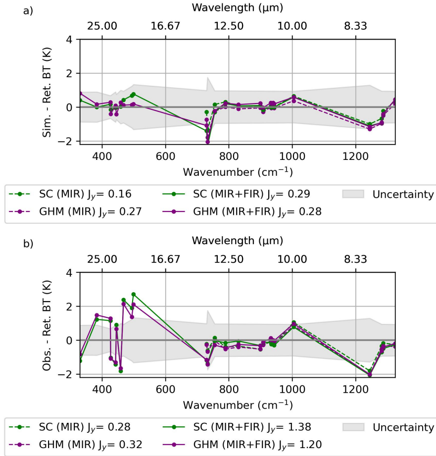
Figure 8. The BT residuals and J_y in the cloud-sensitive channels using the (dashed) mid-infrared (MIR) only and (solid) mid- and far-infrared (MIR+FIR) on the FORUM-aircraft (a) simulation and (b) observation. The residuals within the MIR are partially obscured by the combined MIR+FIR retrieval. The retrievals using the SC and GHM models are shown in green and purple, respectively. The square-root-diagonal of S_y is shaded in grey as the uncertainty.
