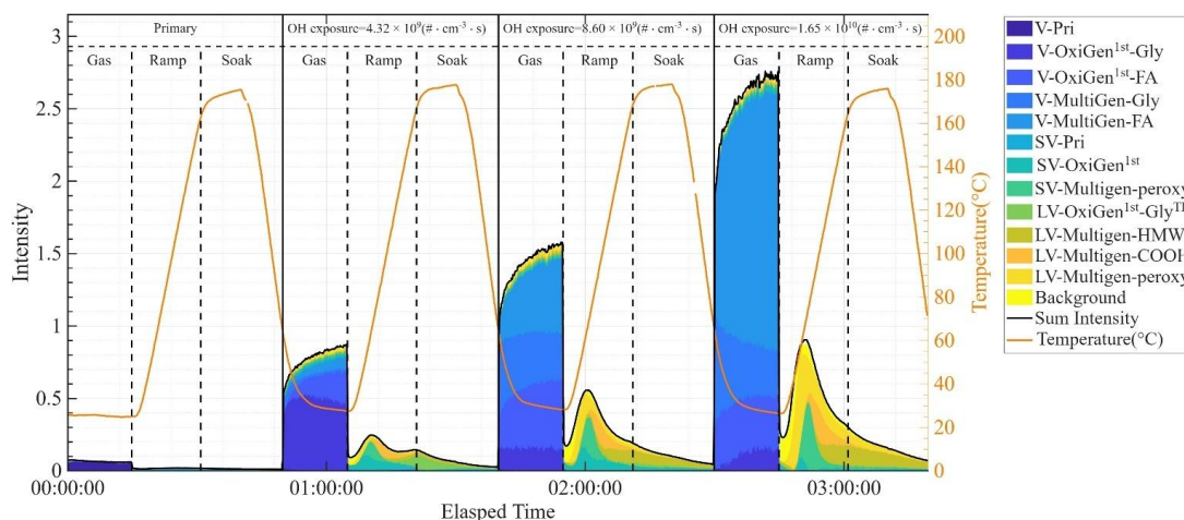
Figure 3 Factor time series of ME-2 PMF classification result with strengthen of OH exposure. Y-axis Intensity represents the sum of CIMS organic signal normalized to iodide ion other than formic acid.
