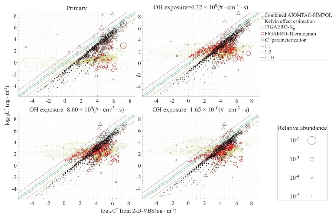
475 Figure 5 The characteristic effective saturated concentration C^* of FIGAERO-CIMS detected species utilizing different estimation methods with enhancement of OH exposure. Markers show combined AIOMFAC-SIMPOL vapor-pressure and activity coefficient estimation methods accounting for kelvin effect (triangle), K_p from FIGAERO measurements (yellow circle), T_{\max} from FIGAERO thermograms (red circle), C^* parametrization(West et al., 2023) (reverse triangle). Lines shows 1:1,1:2 and 1:10 position. Marker size represents relative abundance of species.
