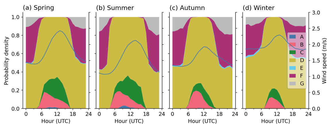
Figure 16. Seasonal mean diurnal cycle of the probability distribution of atmospheric stability and of the wind speed averaged over all sites. Atmospheric stability ranges from very unstable (A) to very stable (G), with D representing neutral conditions.
