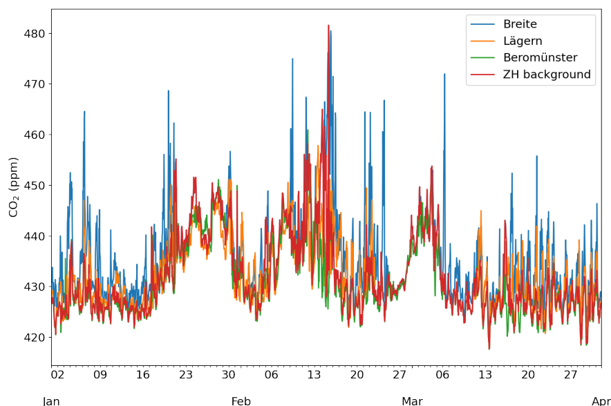
Figure 10. Time series of CO 2 concentrations at the three background sites Beromünster, Lägern and Breite-Birchwil and the constructed Zurich background time series for the first three months of 2023.
