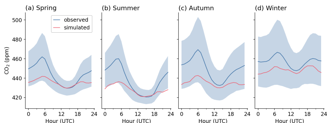
Figure 15. Seasonal mean diurnal cycle of \text{CO}_2 averaged over all mid-cost stations excluding the sites zjho, zsch, zhrgn, reck, hard2. The blue shaded area denotes the standard deviation of the hourly values.
