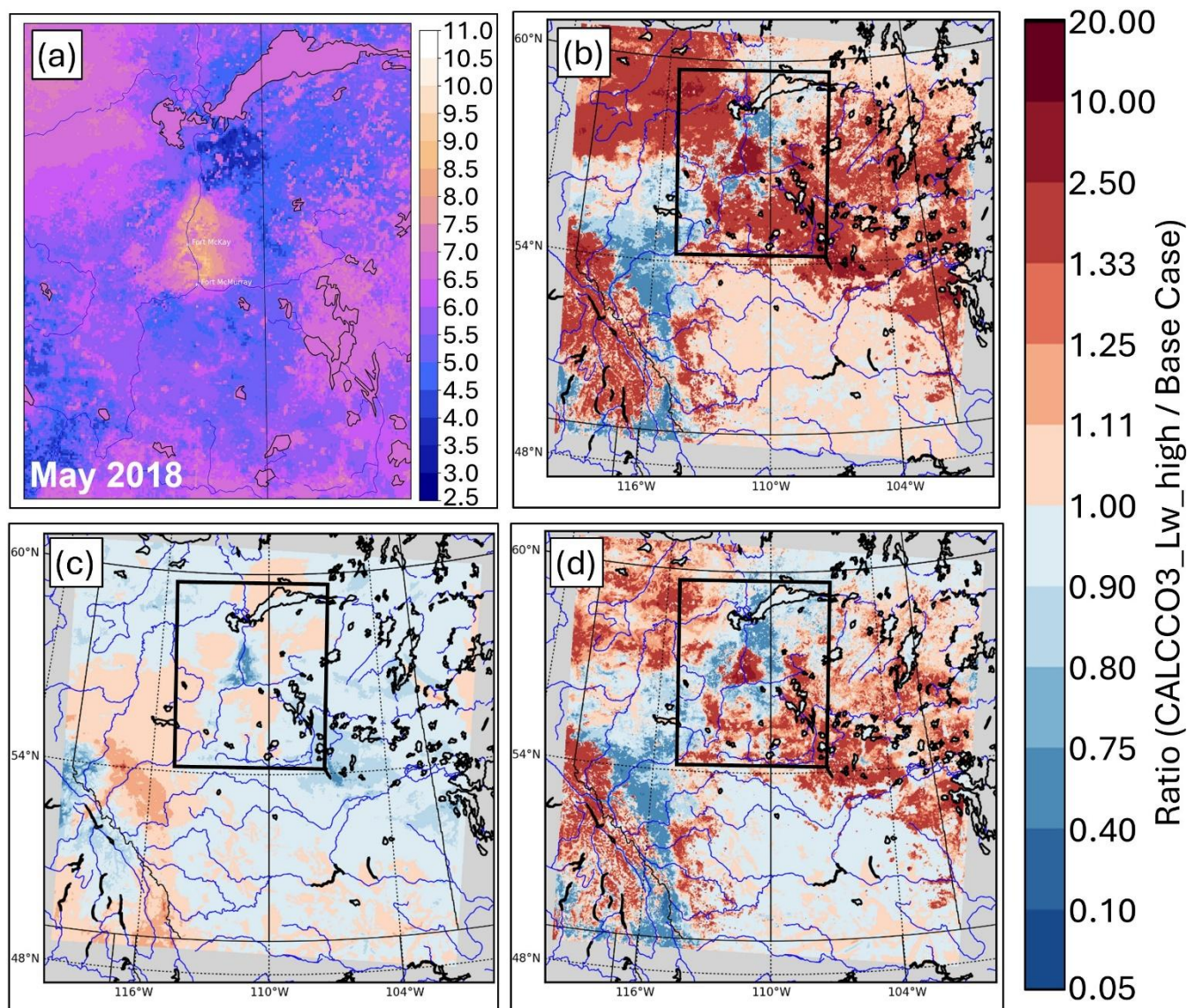
660 Figure 6: Average impact of surface foliage pH. May, 2018. (a): AOSR average surface foliage pH calculated using CALCCO3_Lw_high. (b,c,d) Ratios (CALCCO3_Lw_high: Base Case) of (b) \cdot V_{dSO_2} , (c) SO 2 concentration at the surface, (d) Monthly SO 2 deposition flux at the surface. Inset box in panels (b,c,d) shows the AOSR, displayed as a “zoom” in panel (a). Supplemental Fig. S3 shows the Base Case and CALCCO3_Lw_high values corresponding to panels (b,c,d).
