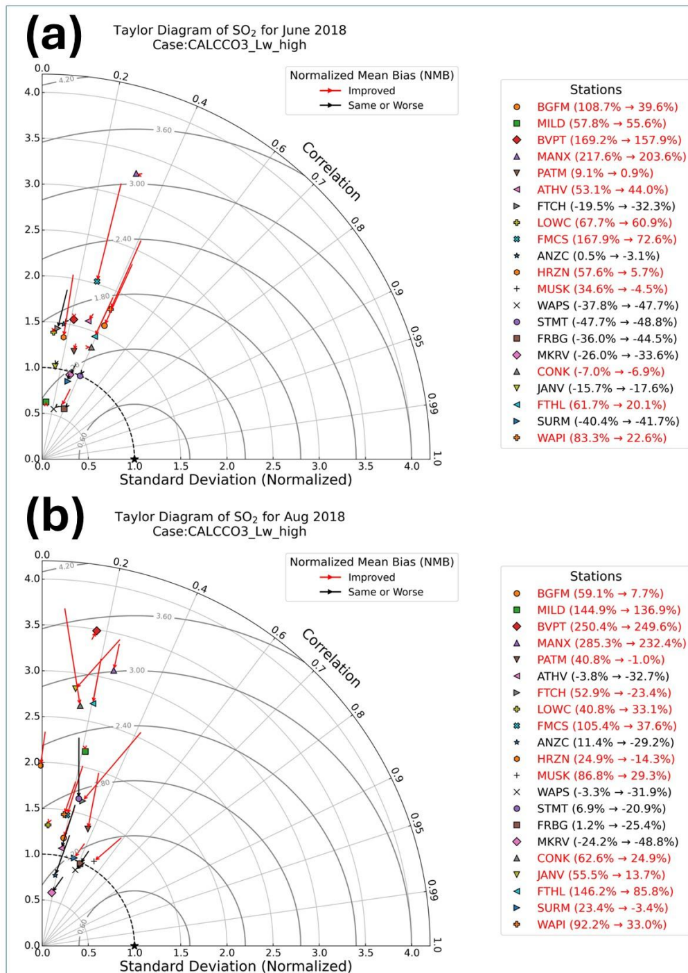
Figure 11: Taylor Diagram of SO 2 for (a) June 2018, (b) Aug 2018 (see Fig. S10 for May and July). The equations used to compute these metrics are provided in Table S3. In each panel, the “star” symbol on x-axis marks the reference point for a perfect model, corresponding to a correlation = 1.0, a CRMS = 1.0 and a normalized standard deviation = 1.0. Arrows illustrate changes in model performance from the Base Case (arrow start) to CALCCO3_Lw_high (arrow end). A trajectory that moves closer to the reference point indicates improved agreement with observations (red arrows). The CRMS is proportional to the distance from the star; concentric circles centred on the star represent contours of constant CRMS. The standard deviation is measured radially from the origin. The different WBEA stations are denoted by different symbols, with each arrow pointing from the Base Case to CALCCO3_Lw_high locations of station performance on the diagram. Red (black) arrows denote an improvement (deterioration or no change) in the normalized mean bias error (NMB) for CALCCO3_Lw_high compared to the Base Case. The value of the NMB for each station is shown in the legend after the station name as (Base Case → CALCCO3_Lw_high), with red text likewise representing improvements in the NMB when using CALCCO3_Lw_high compared to the Base Case. The azimuthal distance represents the correlation (i.e., r ) starting from 0.0 and increasing clockwise to 1.0. The radial distance from the origin gives the normalized standard deviation of the model at the station. Each station standard deviation has been normalized by the observed standard deviation at that station. Thus, the observed standard deviation is always at (1.0, 1.0) represented by the star on each plot. May and July Taylor diagrams are given in the Supplement, Fig. S10.
