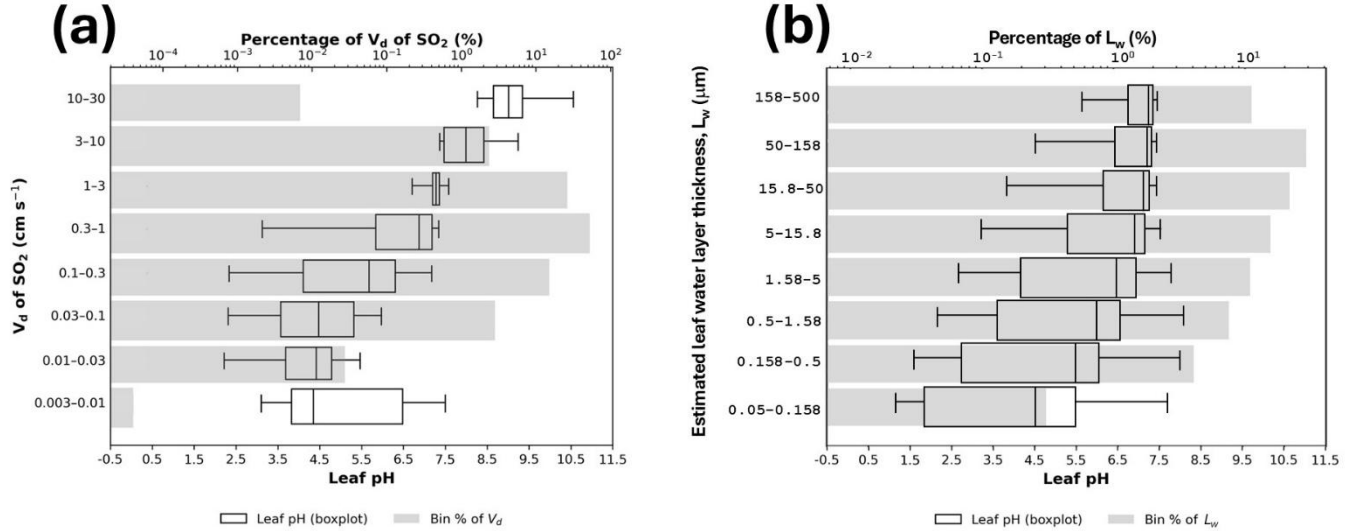
Figure 5: (a): The deposition velocity of \text{SO}_2 ( V_{d\text{SO}_2} , \text{cm s}^{-1} ) as a function of foliage (leaf) pH; data are from May 2018. V_{d\text{SO}_2} has been separated into 8 discrete bins, and the corresponding box plots give the range of leaf pH (lower x-axis) within each bin. The whiskers, box boundaries, central vertical line, etc. from left to right for each box are the 5 th percentile, 25 th percentile, median, 75 th percentile, and 95 th percentile, respectively. This format for box plots is applied henceforth. Each box is superimposed over a shaded bar that gives the percentage of V_{d\text{SO}_2} in the corresponding bin (upper x-axis). (b): The foliage (leaf) pH as a function of the estimated leaf water layer thickness ( L_w , \mu\text{m} ). L_w has been separated into 12 discrete bins, and the corresponding box plot gives the range of leaf pH in the corresponding bin. The shaded bars give the percentage of L_w in each bin (right y-axis).
