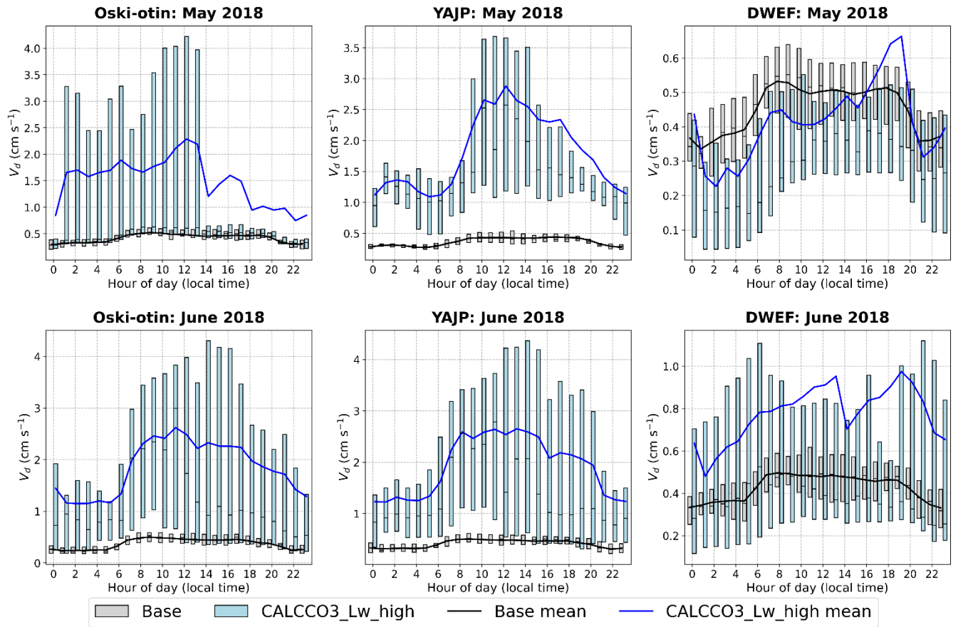
Figure 9: The diurnal cycle of model-predicted V_{dSO_2} at (a, d) Oski-otin, (b, e) the York Athabasca Jack Pine (YAJP) Tower, (c, f) a downwind evergreen forest (DWEF). The first row (a, b, c) shows the predicted V_{dSO_2} for May 2018 while the second row (d, e, f) shows June 2018. The box plot formatting in Fig. 9 is consistent with Fig. 5 and solid lines indicate the mean V_{dSO_2} in each hourly bin.
