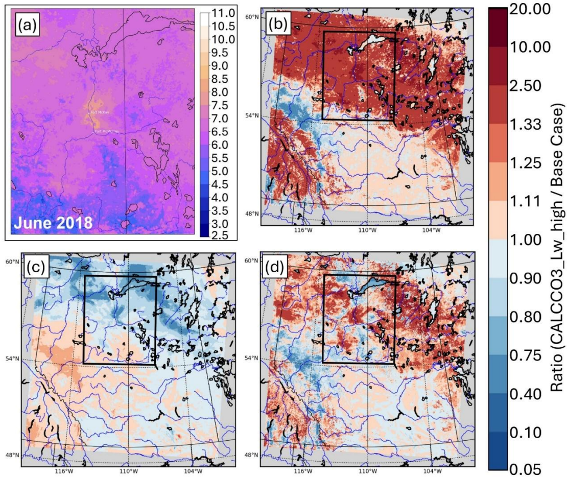
Figure 7: Average impact of surface foliage pH. June, 2018. Panels as in Fig. 6. Supplemental Fig. S4 shows the Base Case and CALCCO3_Lw_high values corresponding to panels (b,c,d).
