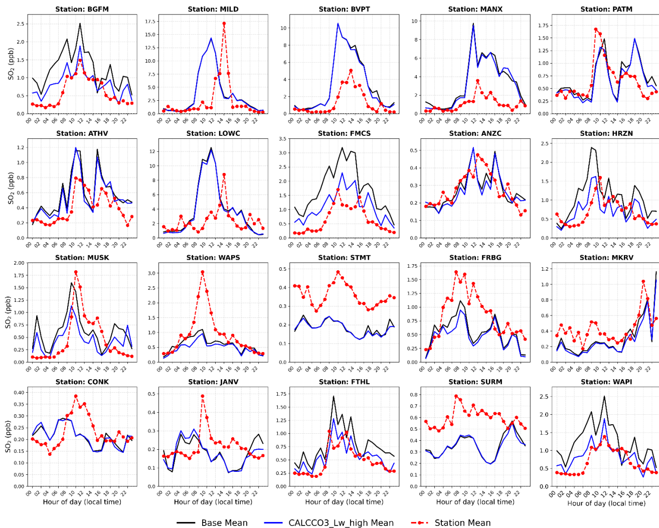
795 Figure 10: The mean diurnal cycle of \text{SO}_2 measured at WBEA continuous monitoring stations (red dashed line) given in local time. The data are for the month of June 2018. Also shown are the model predicted mean \text{SO}_2 surface concentrations at the same location. The black line is the Base Case, while the blue line is CALCCO3_Lw_high. Note that due to plotting limitations the WBEA station 'FTCH' is not included in the figure. Identical plots for May, July and August 2018 are provided in the supplemental material (Fig. S5, S6, S7, respectively).
