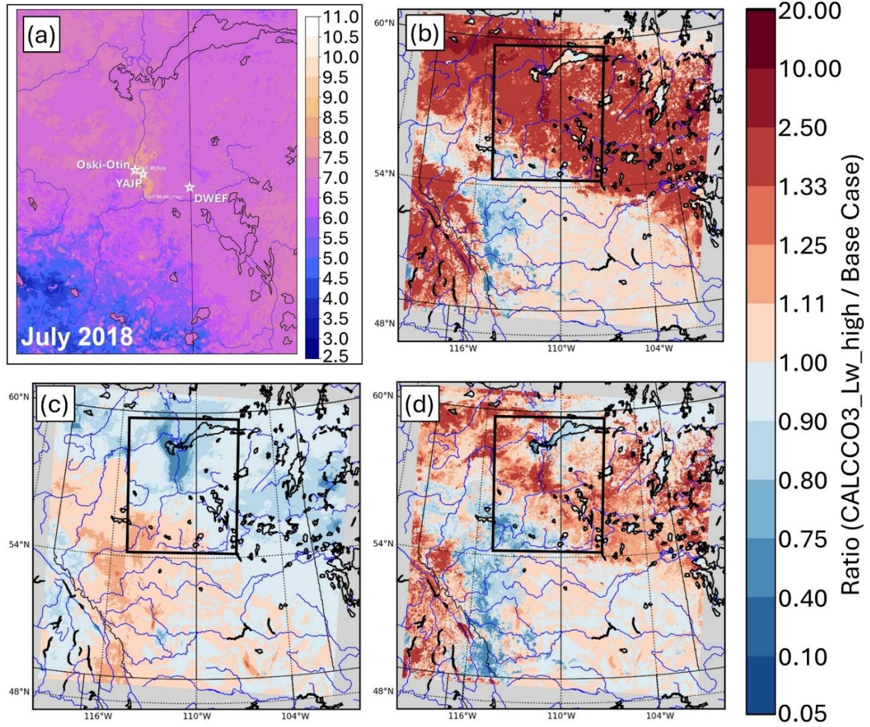
700 Figure 8: Average impact of surface foliage pH. July, 2018. Panels as in Fig. 6. Supplemental Fig. S5 shows the Base Case and CALCCO3_Lw_high values corresponding to panels (b,c,d). The locations of Oski-otin, YAJP and DWEF (stars) are provided for reference to Fig. 9.
