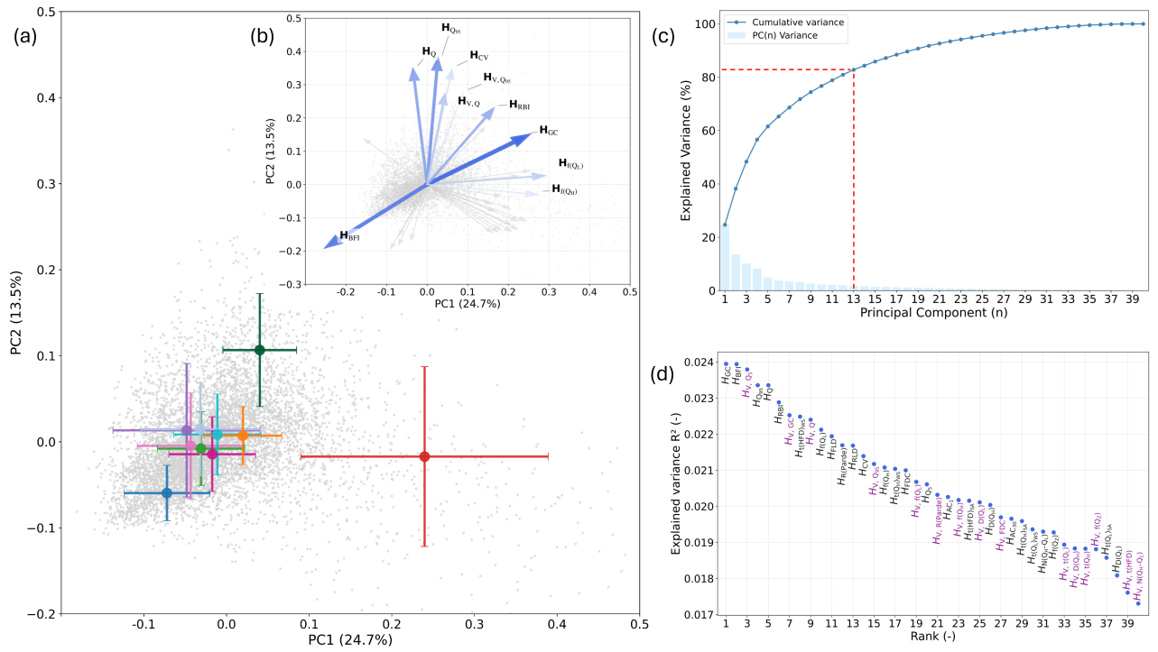
Figure 3. Principal component analysis (PCA) of the 40 hydrological signatures across the HRTs. (a) explained variance of PC1 (24.7%) and PC2 (13.5%) for each catchment (grey), with HRT means and standard deviations shown in their respective colour. (b) loadings of the hydrological signatures, shown for PC1 and PC2. Arrow thickness and colour intensity reflect each signature's ranked explained variance based on the first 13 PCs (see panel d), accounting for just above 80% of the cumulative explained variance. Thicker and more intense coloured arrows indicate more informative signatures. (c) cumulative explained variance across all principal components. The explained variance of the first 13 PCs is highlighted by the red dashed lines. (d) ranked explained variance of the first 13 PCs, which together account for approximately 80% of the total variance. Signatures related to variance are highlighted in purple.
