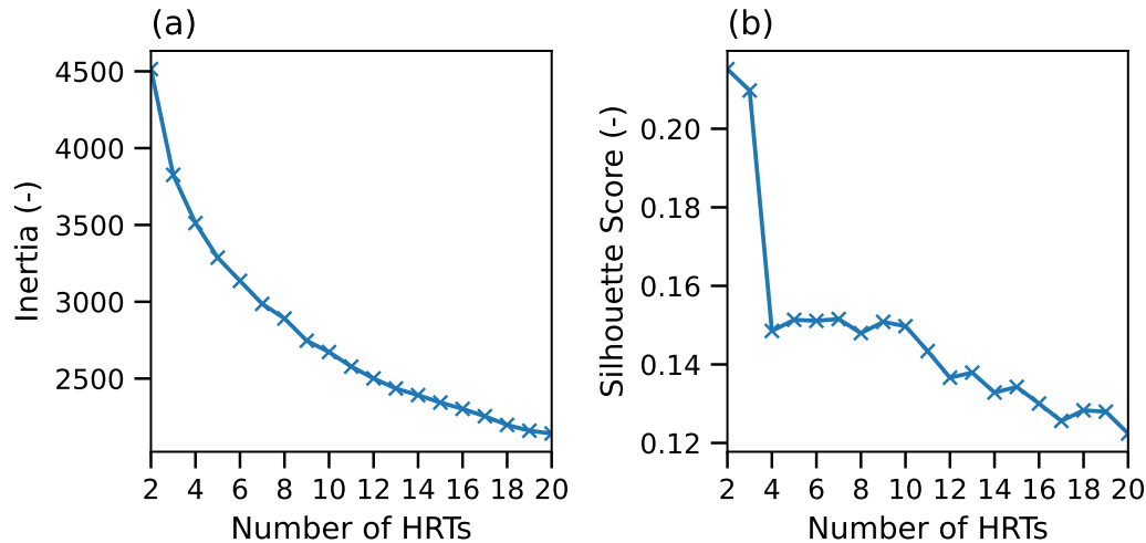
Figure 2. Assessment of cluster robustness using k-means clustering. (a) Elbow Method results for k = 2-20 HRTs, used to evaluate the optimal number of hydrological response types. (b) Silhouette Scores for the same range of HRTs, providing an additional metric of cluster cohesion and separation.
