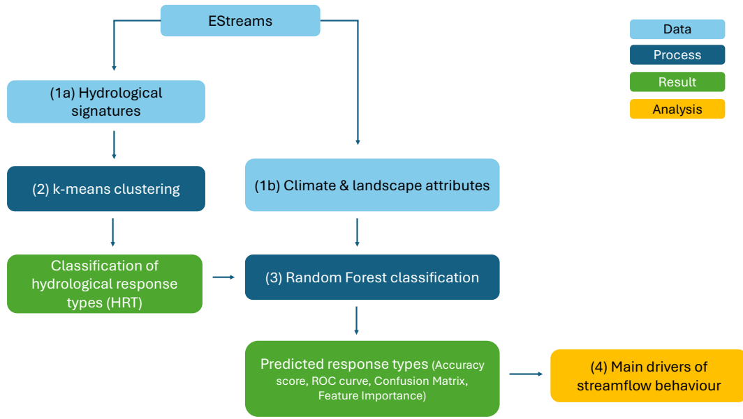
Figure 1. Workflow of the study. Streamflow time series and catchment attributes (1) were used to classify hydrological response types (HRT) to the individual catchments via k-means clustering (2) and predict HRT membership using a Random Forest classification model (3). The importance of individual attributes was quantified from the Random Forest classification model to identify the dominant controls on HRT membership and thus the main drivers of the hydrological response (4).
