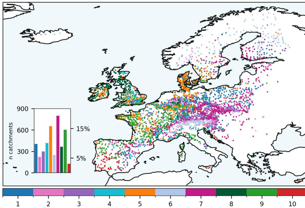
Figure C1. Classification of 4137 non-nested catchments into 10 HRT based on 40 hydrological signatures. The HRTs are ordered by increasing slope of the flow duration curves.
