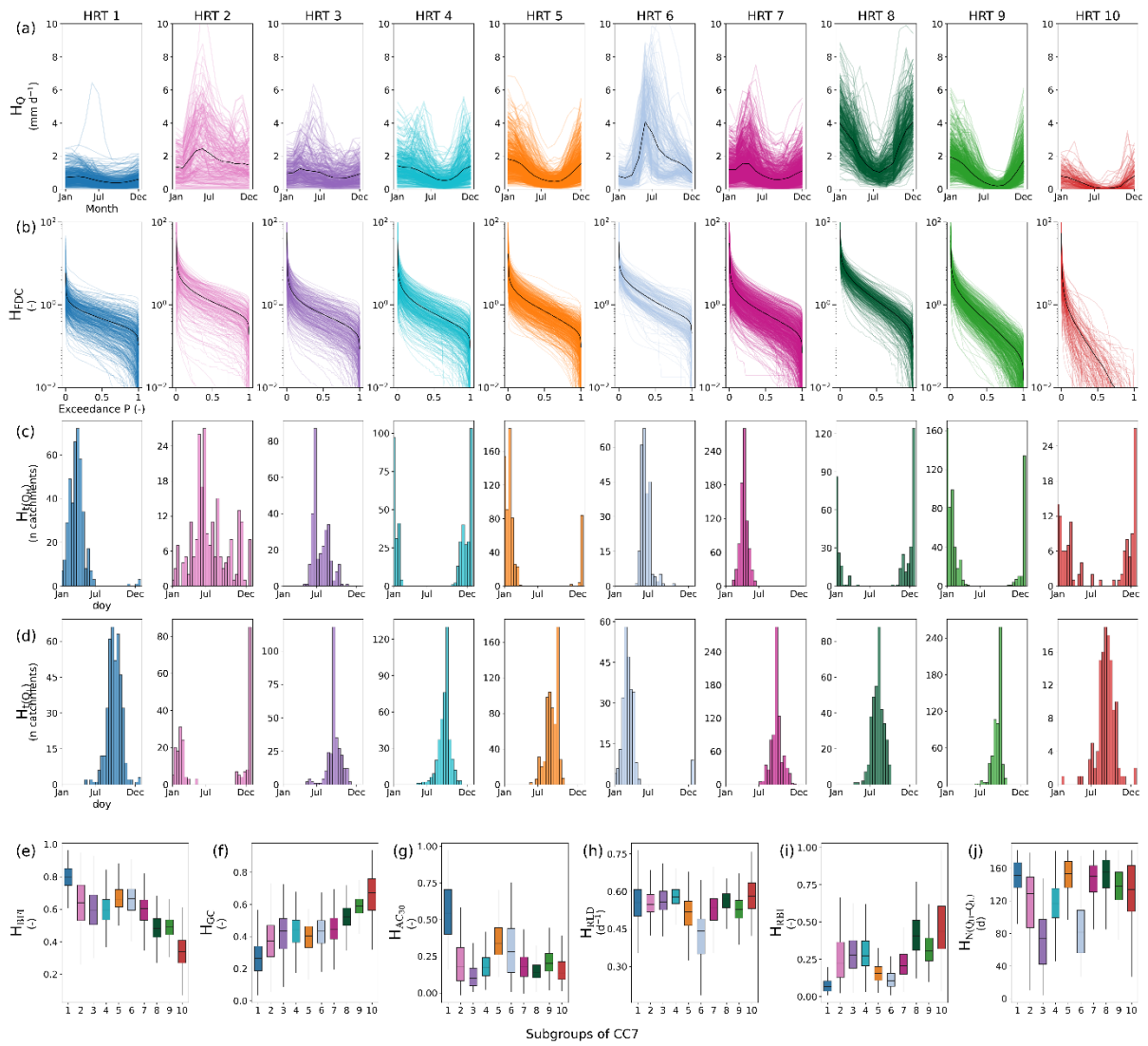
Figure C2. Visualization of 10 out of the 40 hydrological signatures across hydrological response types (HRTs) for the analysis of non-nested catchments.
