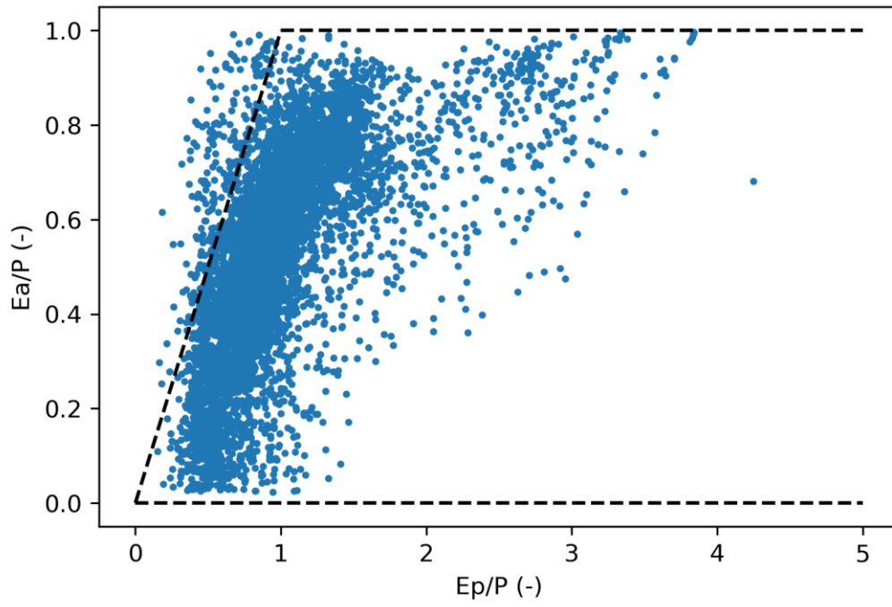
Figure C3. The 7175 catchments used in the analysis plotted in the Budyko framework.
