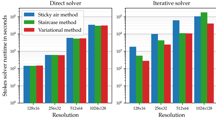
Figure 17. Performance across all resolutions is consistent between discretisation methods when using a direct solver (typical for 2D models). However, with an iterative multigrid solver, significant performance gains are observed when using the variational method.
