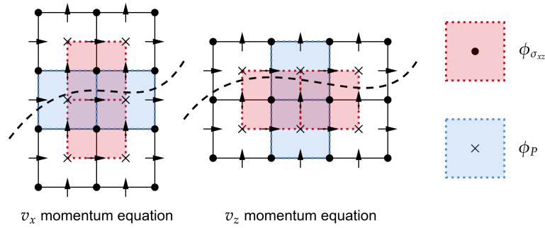
Figure 4. In 2D, the v_x and v_z momentum equations are solved only if at least one of the pictured volume fractions surrounding the velocity point is nonzero.
