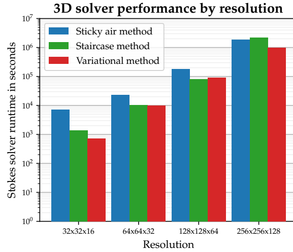
Figure 18. 3D scaling tests, conducted using an iterative multigrid solver on a constant-viscosity Cartesian box domain at various resolutions, demonstrate that the variational method consistently outperforms the sticky air method. The staircase method shows variable performance results.
