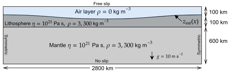
Figure 11. 2D surface relaxation benchmark based on Case 1 presented by Crameri et al. (2012). An initially non-flat surface in a three-layer model relaxes until equilibrium is reached after approximately 100 ky.
