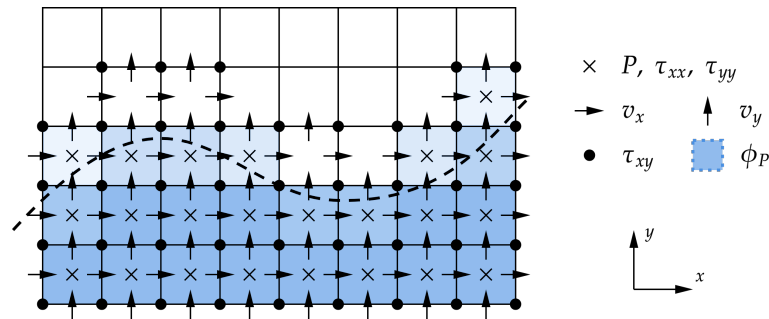
Figure 5. The discretised Stokes equations on a simplified domain using the variational method. Cell-centred volume fractions \phi_P dictate where the continuity equation is solved; cells with zero volume fraction (white) are excluded.
