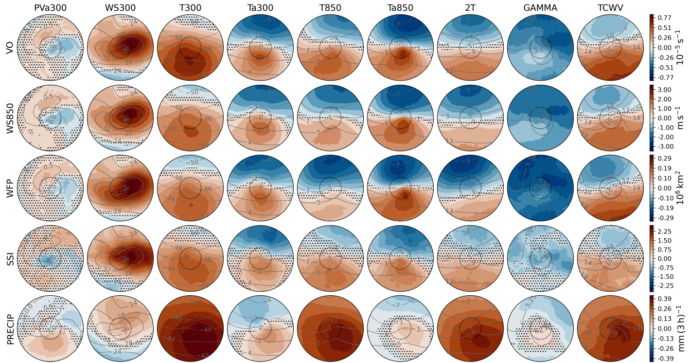
Figure 3. Sensitivity signal of each combination for all ETCs (shading) and the composite field of precursors at genesis (contours). Intensity measures stay constant along rows and precursors stay constant along columns. There is one colourbar per intensity measure, i.e. per row. The hatched areas indicate statistically nonsignificant values and the dashed black circle denotes a radius of 6° geodesic. The radius of the whole circle is 18° geodesic. Units of precursors are PVU ( 10^{-6} \text{ K m}^2 \text{ kg}^{-1} \text{ s}^{-1} ) for PVa300, \text{m s}^{-1} for WS300, ^{\circ}\text{C} for T300, Ta300, T850, Ta850, and 2T, ^{\circ}\text{C km}^{-1} for GAMMA, and \text{kg m}^{-2} for TCWV.
