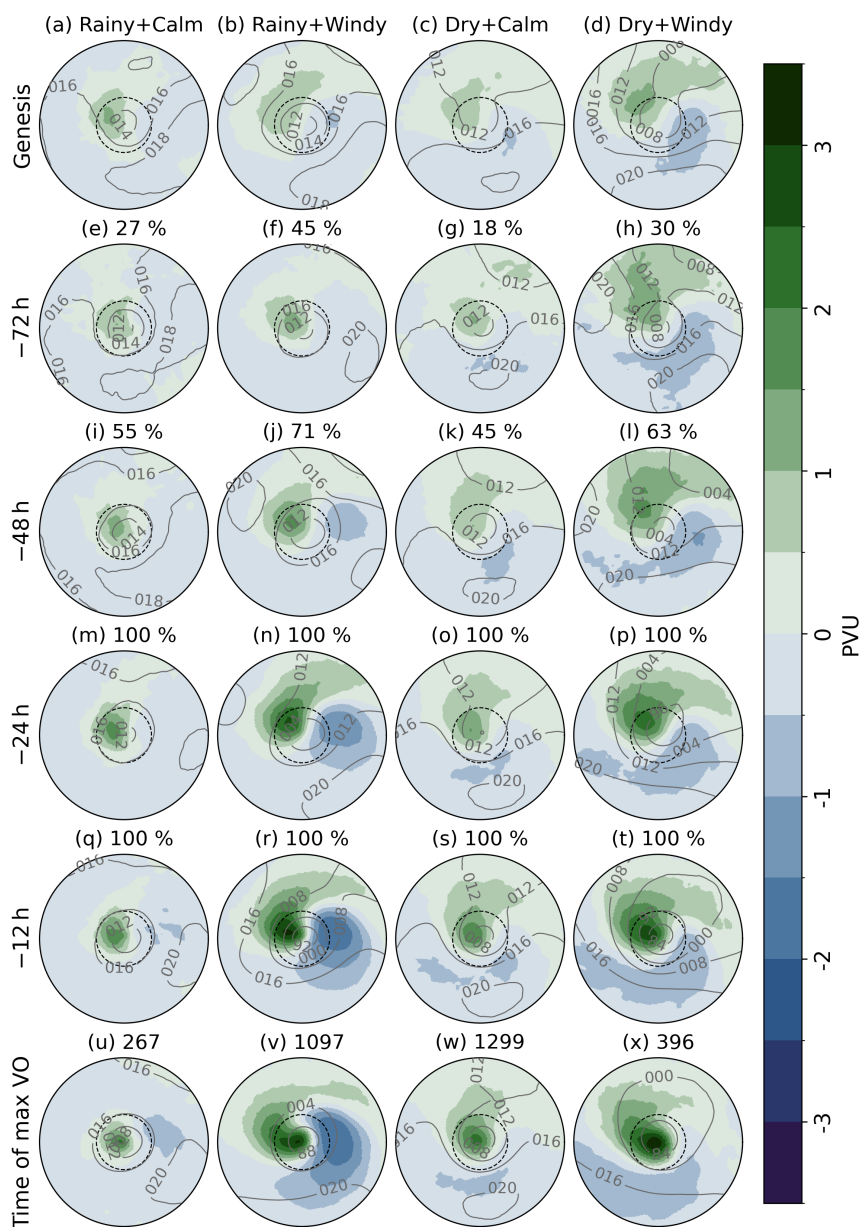
Figure 8. As in Fig. 7, with the shading showing PVa300.
