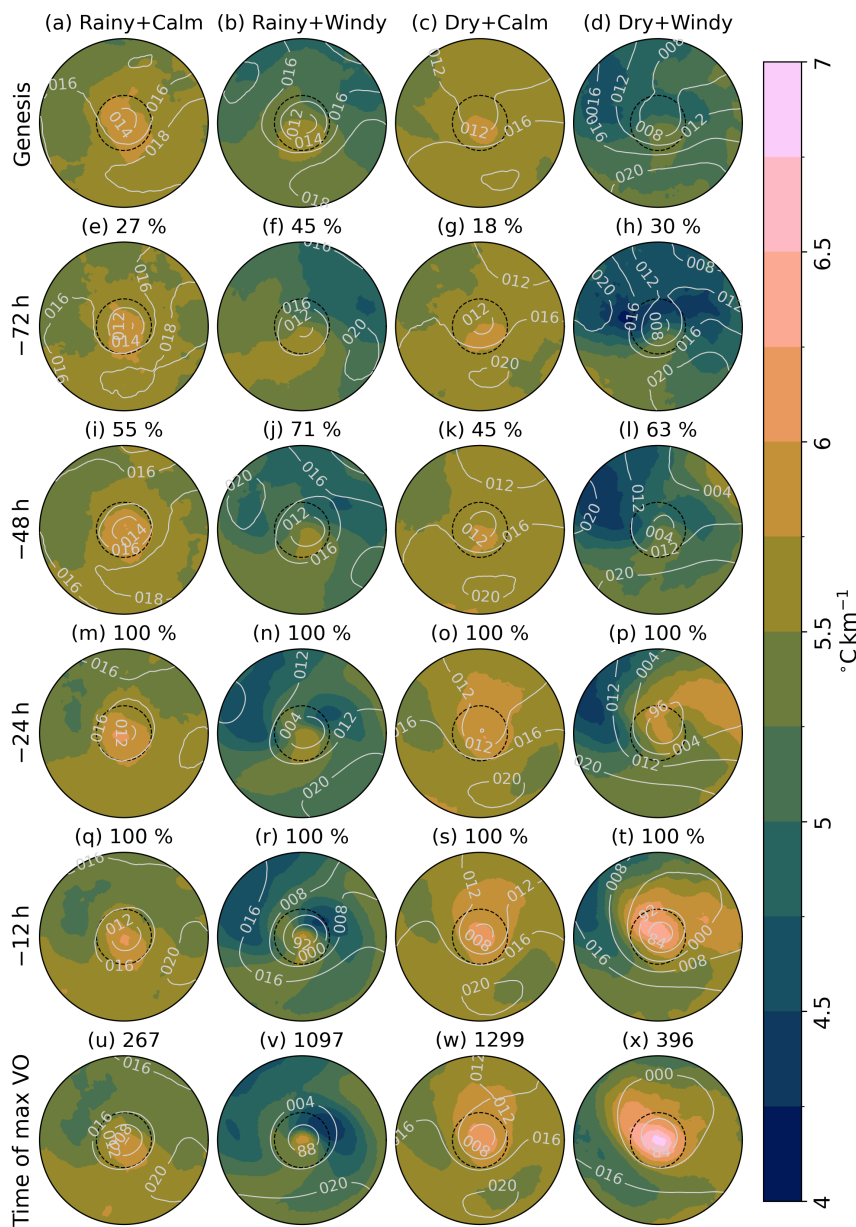
Figure 11. As in Fig. 7, with the shading showing GAMMA, defined as -\frac{[T(850 \text{ hPa}) - T(500 \text{ hPa})]}{[Z(850 \text{ hPa}) - Z(500 \text{ hPa})]} , where T is temperature and Z geopotential height.
