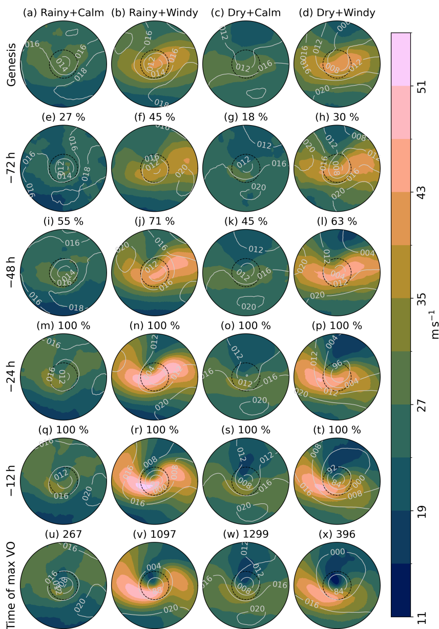
Figure 7. Composite evolution of WS300 (colours) in the four intensity groups. MSLP composite is shown in the contours in hPa with the leading number (1 or 9) omitted. The dashed black circle denotes a radius of 6° geodesic and the radius of the whole circle is 18° geodesic. The numbers on top of panels in the last row indicate the total size of the group. Percentages on other rows indicate the proportion available to sample of these sizes. Genesis time includes full sample, the same as the time of maximum VO.
