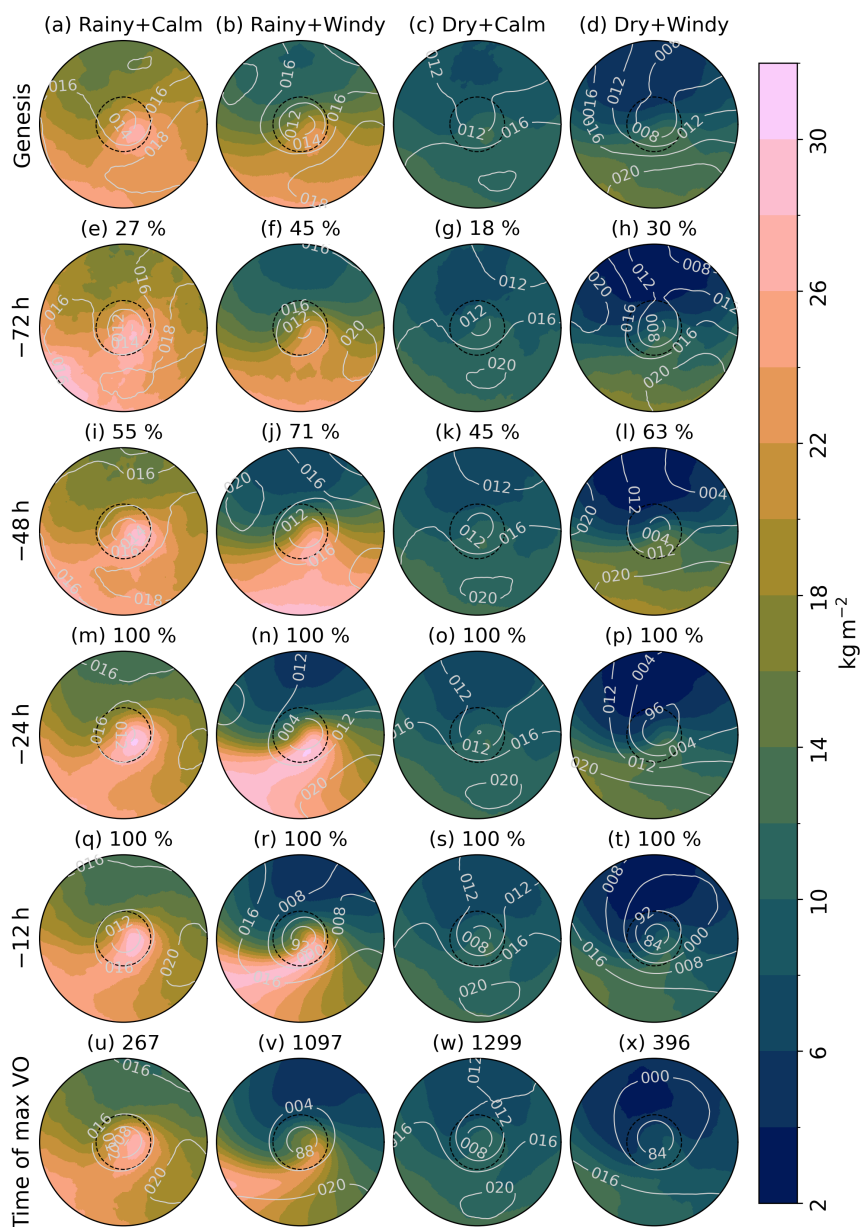
Figure 10. As in Fig. 7, with the shading showing TCWV.
