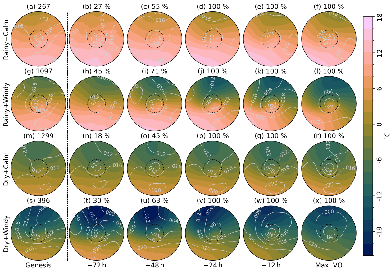
Figure 9. As in Fig. 7, with the shading showing T850.
