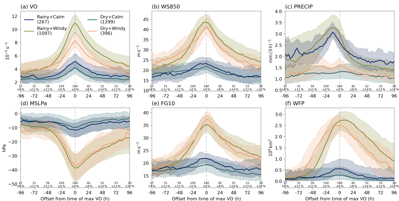
Figure 6. Average evolution of six selected intensity measures in the four intensity groups relative to the time of maximum VO. The solid line shows the median value and the shading contains values in the two middle quartiles. Percentages on the x-axis show the mean and standard deviation of proportion of tracks sampled in the groups for a given time step. The complete group sizes are shown in parentheses in the legend in panel (a). Median times of maximum VO in the groups are shown in Fig. S13.
