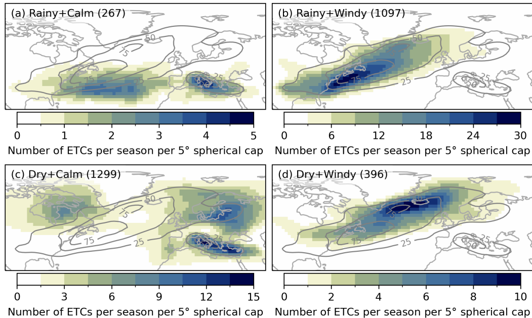
Figure 2. Track densities of the four intensity groups. The value indicates the number of ETCs occurring within a spherical cap with a radius of 5° geodesic per season (six months). The contours show the track density distribution of the full dataset (7361 ETCs) in the same unit. Total number of ETC tracks in each group is shown in the parentheses. Note the different values in the colourbars.
