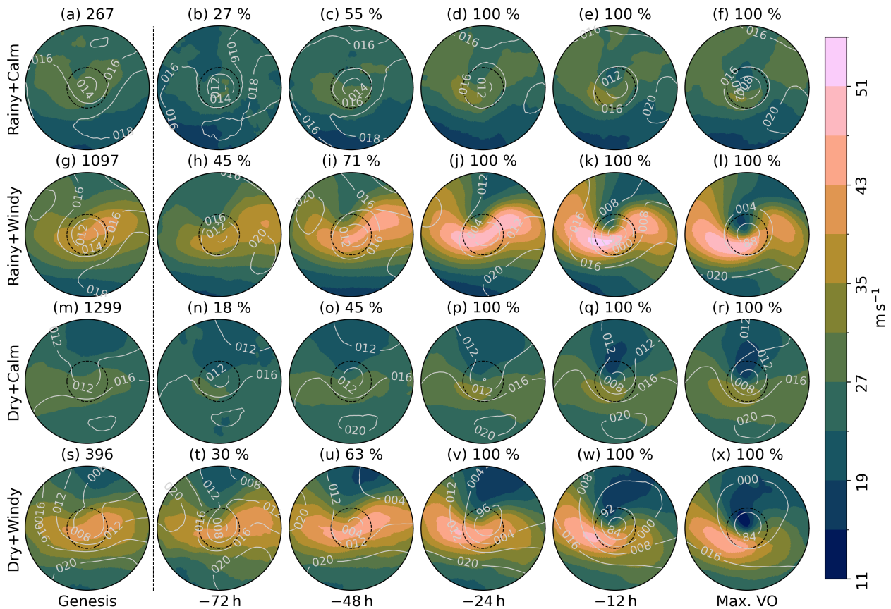
Figure 7. Composite evolution of WS300 (colour shading) in the four intensity groups (rows). MSLP composite is shown in the contours in hPa with the leading number-digit (1 or 9) omitted. The dashed black circle denotes a radius of 6^\circ geodesic and the radius of the whole circle is 18^\circ geodesic. The numbers on top of panels in the last row-first column indicate the total size of the each group. Percentages-The percentages on top of other rows-panels indicate the proportion available to sample of from these sizes -Genesis at a given time includes full sample, relative to the same-as-the-time of maximum VO (columns).
