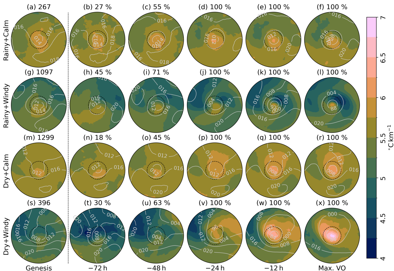
Figure 11. As in Fig. 7, with the shading showing GAMMA, defined as -\frac{T(850 \text{ hPa}) - T(500 \text{ hPa})}{Z(850 \text{ hPa}) - Z(500 \text{ hPa})} , where T is temperature and Z geopotential height.
