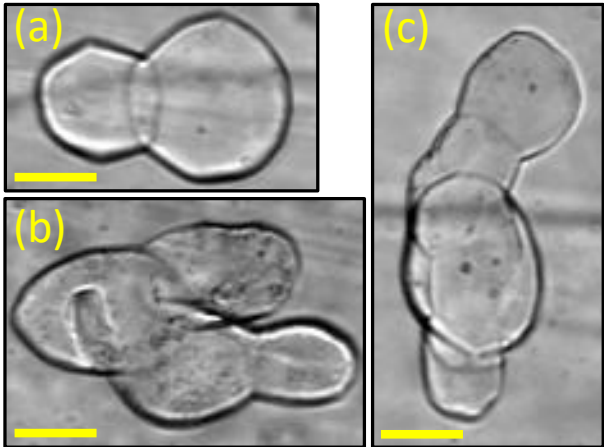
Figure 9. Example of clustered air hydrates in the sample from 2405 m depth. Scale bars correspond to 100 \mu\text{m} . a) represents a "simple" clustered air hydrate, b) and c) represent "multi" clustered air hydrates. The equivalent-circle diameter for a), b) and c) is 257, 299 and 296 \mu\text{m} , respectively, which is about two times the samples' \bar{D} (137 \mu\text{m} ).
