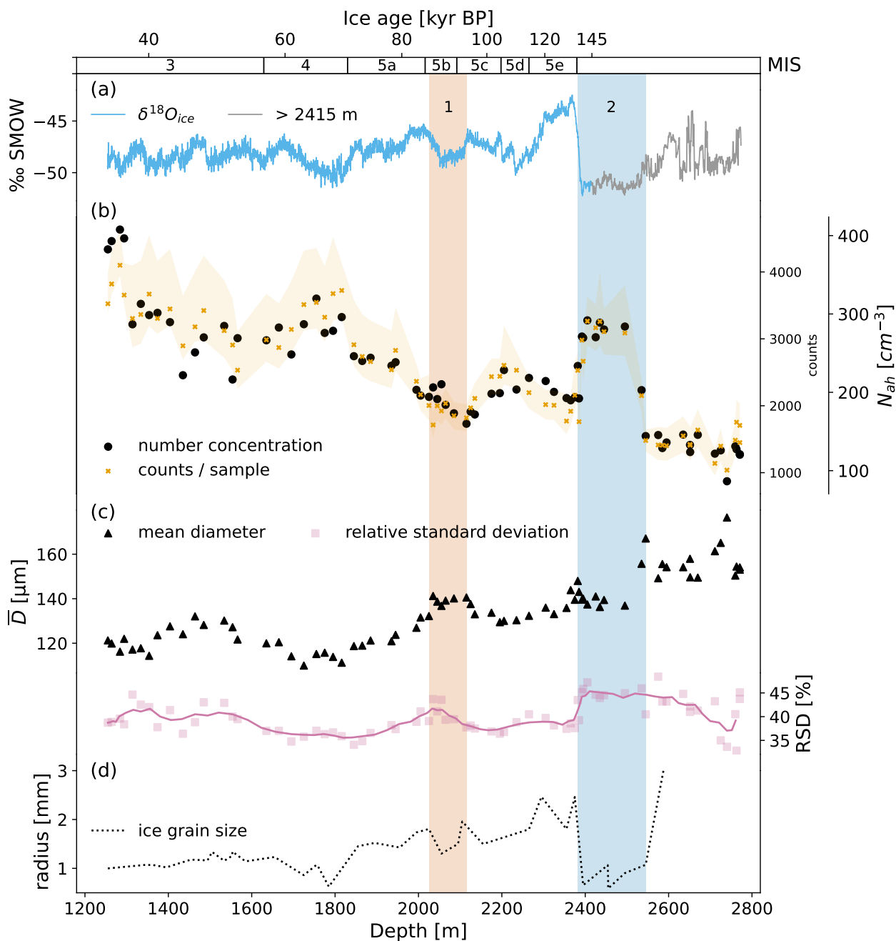
Figure 5. Air hydrate depth profiles of the EDML ice core. a) Paleo-climatic information as \delta^{18}\text{O}_{\text{ice}} values (EPICA Community Members, 2010; Meyer et al.), b) air hydrate number concentration ( N_{ah} ), c) mean diameter ( \bar{D} ) and relative standard deviation (RSD) and d) ice grain size (Weikusat et al., 2009). The ice age at the top of the figure corresponds to the AICC 2023 for EDML (Bouchet et al., 2023). The MIS boundaries are defined by Lisiecki and Raymo (2005), the MIS 5 substage boundaries are from Otvos (2015). Error-band for b) is explained in section 2.4.
