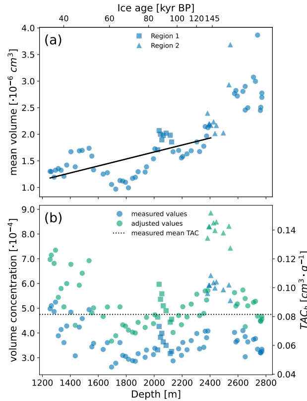
Figure 6. a) Air hydrate mean volume. The solid line represents the calculated growth rate for the dated part of the EDML ice core (1255 - 2415 m; Ruth et al., 2007). b) Blue markers: air hydrate volume concentration and total air content calculated from theoretical air content of air hydrates. Green markers: adjusted values to match the measured mean TAC for EDML (dotted line at 0.0815 cm 3 g -1 ; Ruth et al., 2004). Square markers correspond to samples from 2025 - 2115 m depth (region 1 in Figs. 5,7). Triangular markers correspond to samples from 2382 - 2545 m depth (region 2 in Figs. 5,7). The ice age at the top of the figure corresponds to the AICC 2023 for EDML (Bouchet et al., 2023).
