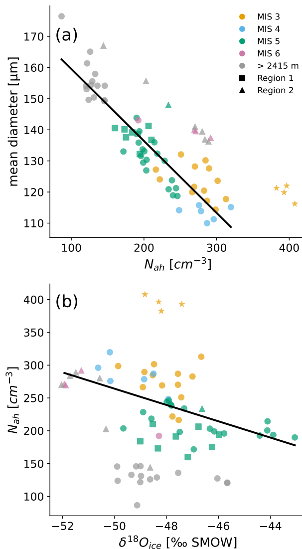
Figure 8. a) N_{ah} plotted against \bar{D} . The linear correlation and the Pearson Correlation Coefficient are calculated without considering data from 1255 - 1294 m and region 2 ( R = -0.92 , p < 0.001 ). b) \delta^{18}O_{ice} plotted against N_{ah} . The linear correlation and the Pearson Correlation Coefficient are calculated without considering samples from 1255 - 1294 m and deeper than 2415 m ( R = -0.57 , p < 0.001 ). Square markers correspond to samples from 2025 - 2115 m depth (region 1 in Fig. 5,7). Triangular markers correspond to samples from 2382 - 2545 m depth (region 2 in Fig. 5,7).
