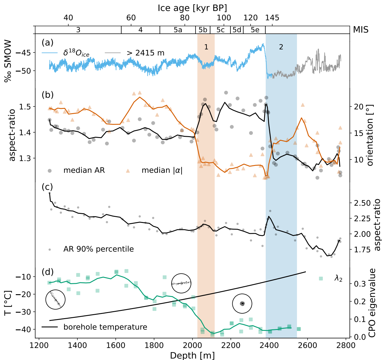
Figure 7. Shape characteristics of air hydrates in the EDML ice core. a) Paleo-climatic information as \delta^{18}O_{ice} values (EPICA Community Members, 2010; Meyer et al.), b) air hydrate median AR and median of the absolute orientations ( |\alpha| ), c) 90% percentile of air hydrate AR and d) measured borehole temperature (Weikusat et al., 2017) and the second eigenvalue of the orientation tensor of the ice crystals c-axis distribution measured on vertical sections (Weikusat et al., 2013). Schematic stereographic projections are added to display the respective changes in ice CPO. The ice age at the top of the figure corresponds to the AICC 2023 for EDML (Bouchet et al., 2023). The MIS boundaries are defined by Lisiecki and Raymo (2005), the MIS 5 substage boundaries are from Otvos (2015).
