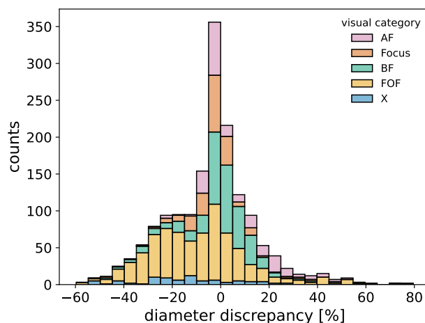
Figure 3. Stacked distribution of diameter discrepancy for each air hydrate in the eight GT- compared to the corresponding segmented image. The different colors and abbreviations correspond to the different visual categories in Table 1. The mean value and standard deviation are -4% and \pm 18\% , respectively.
