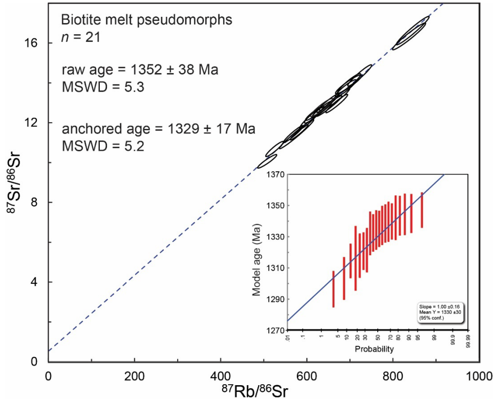
325 Figure 9. Rb-Sr data for biotite that occurs as melt-film pseudomorphs in Tasiyak Gneiss at the contact with the MLP. This textural variety of biotite is characterized by a narrow range of ^{87}\text{Rb}/^{86}\text{Sr} . The inset linearized probability curve was generated with model ages calculated at initial ^{87}\text{Sr}/^{86}\text{Sr} = 0.73 .
