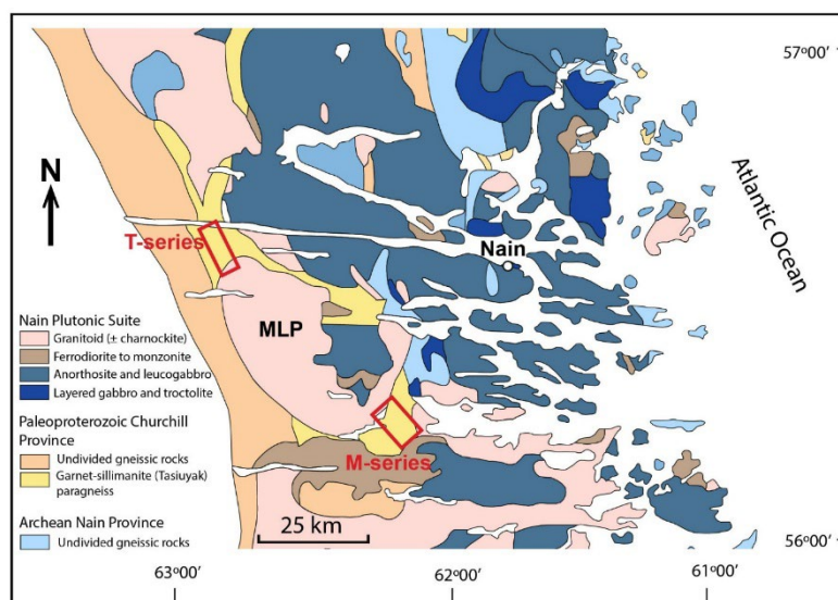
Figure 1. Location of the Makhavinekh Lake Pluton (MLP), host Tasiuyak paragneiss, and the surrounding Nain Plutonic Suite intrusions in the vicinity of Nain, coastal Labrador. Samples for this study were selected from two previously described transects from the northern (T-series samples) and southeast (M-series samples) contact zones of the MLP. Modified from Lightfoot et al (2012).
