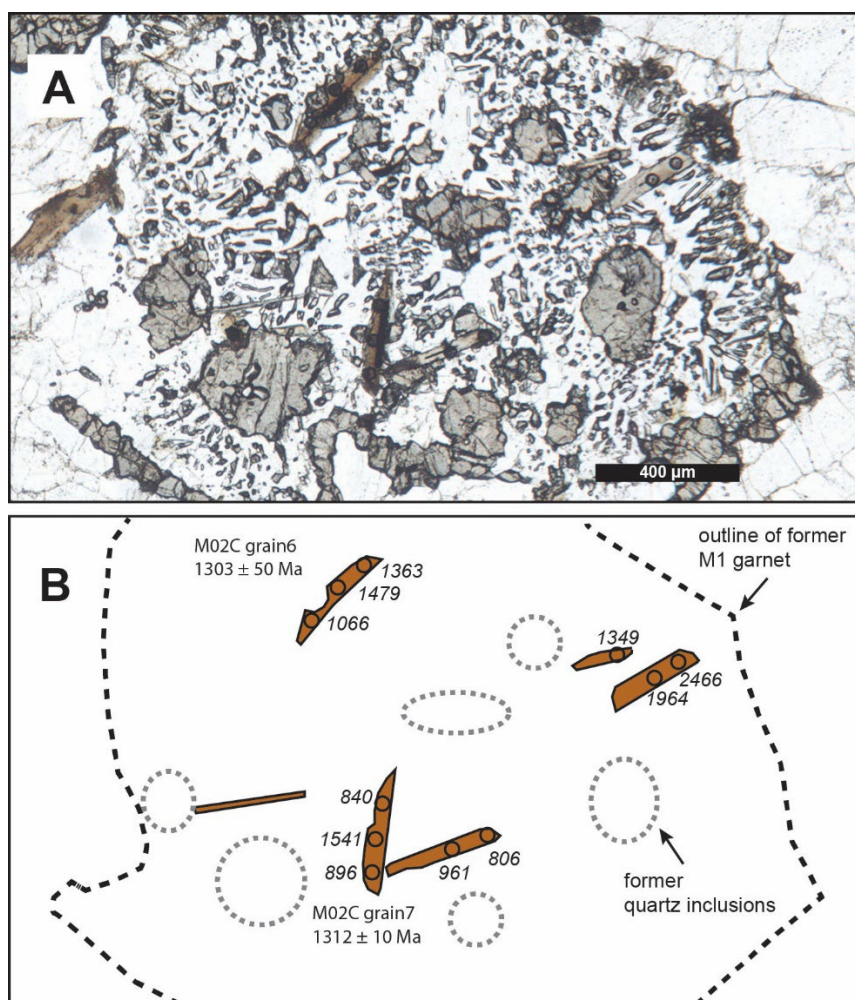
Figure 7. Detail of biotite neoblasts in inner aureole sample M02C-10. A) Plane light photomicrograph showing the locations of 26\mu\text{m} diameter laser craters distributed across individual grains. B) Line drawing illustrating biotite neoblasts and associated ^{87}\text{Rb}/^{86}\text{Sr} at the laser sample locations shown by black circles. Anchored three-point isochron ages are shown for two grains.
