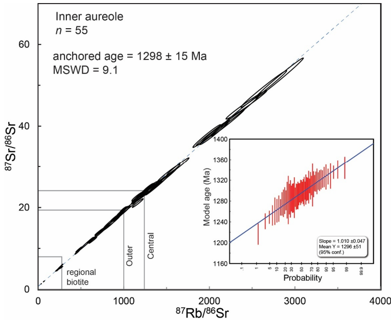
Figure 76. Rb-Sr data for neoblastic biotite grains in textural equilibrium with Opx + Crd corona in the inner aureole. Boxes show range of isotope ratios encountered in armoured regional biotite , the outer aureole and the central aureoles . The raw regression overlaps the known crystallization age of the MLP as well as the initial Sr recorded in plagioclase . Regression age and intercepts for data with model ages above or below 1322 Ma (anchored at f_{Sr} = 0.73 ) are also shown. Inset linearized probably plot for model ages ( 1\sigma error bars excluded for clarity ) reveals a gently curving array with a slope of unity within uncertainty . One anomalously young point was rejected for calculation purposes.
