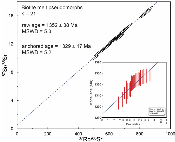
Figure 98. Rb-Sr data for biotite that occurs as melt-film pseudomorphs in Tasiyuak Gneiss at the contact with the MLP. This textural variety of biotite is characterized by a narrow range of ^{87}\text{Rb}/^{86}\text{Sr} . Dotted ellipses were rejected from the regression calculation (see text for details). The inset linearized probability curve was generated with model ages calculated at initial ^{87}\text{Sr}/^{86}\text{Sr} = 0.73 .
