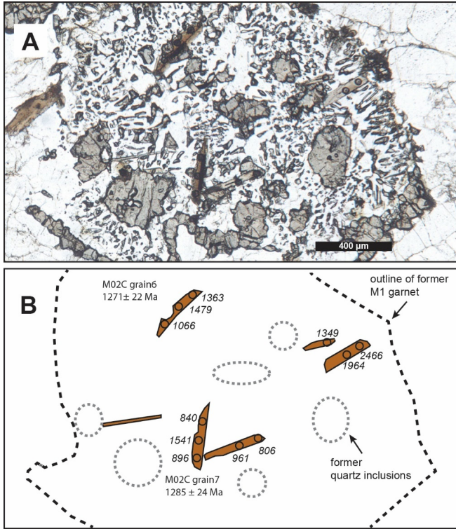
345 Figure 87. Detail of biotite neoblcasts in inner aureole sample M02C-10. A) Plane light photomicrograph showing the locations of 26 μm diameter laser craters distributed across individual grains. B) Line drawing illustrating biotite neoblcasts and associated ^{87}\text{Rb}/^{86}\text{Sr} at the laser sample locations shown by black circles. Anchored three-point isochron ages are shown for two grains.
