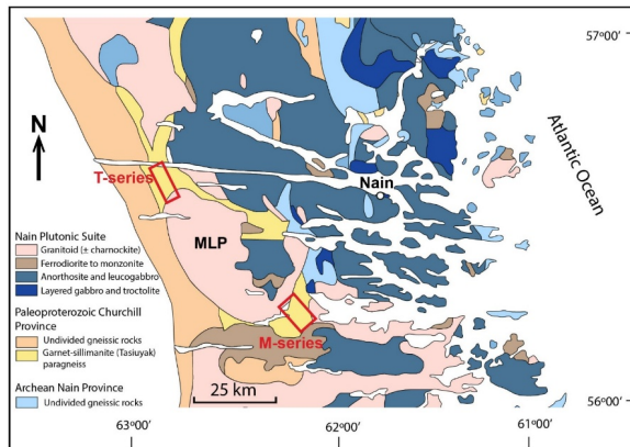
85 Figure 1. Location of the Makhavinekh Lake Pluton (MLP), host Tasiuyak paragneiss, and the surrounding Nain Plutonic Suite intrusions in the vicinity of Nain, coastal Labrador. Samples for this study were selected from two previously described transects from the northern (T-series samples) and southeast (M-series samples) contact zones of the MLP. Modified from Lightfoot et al (2012).
