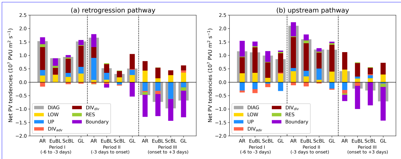
Figure 7. Net effect of amplitude evolution (grey bar) and contributing processes (coloured bars, see legend) for three different time periods (I, II and III; see x-axis for exact time lag information) and the four blocked regimes, split up into the onset PVAs - following the (a) retrogression and (b) upstream pathway.
