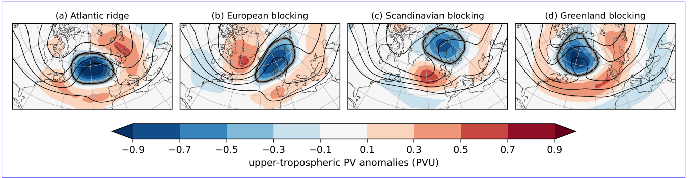
Figure 2. Composites of vertically-averaged PV anomalies between 500–150 hPa (shading) and vertically-averaged PV for all time steps attributed to each of the four blocked regime types (contours, in PVU, from 1.5 to 3.5 PVU in steps of 0.5 PVU). The thick black contour illustrates the regime mask for the respective regime type, defined by the -0.3 PVU contour.
