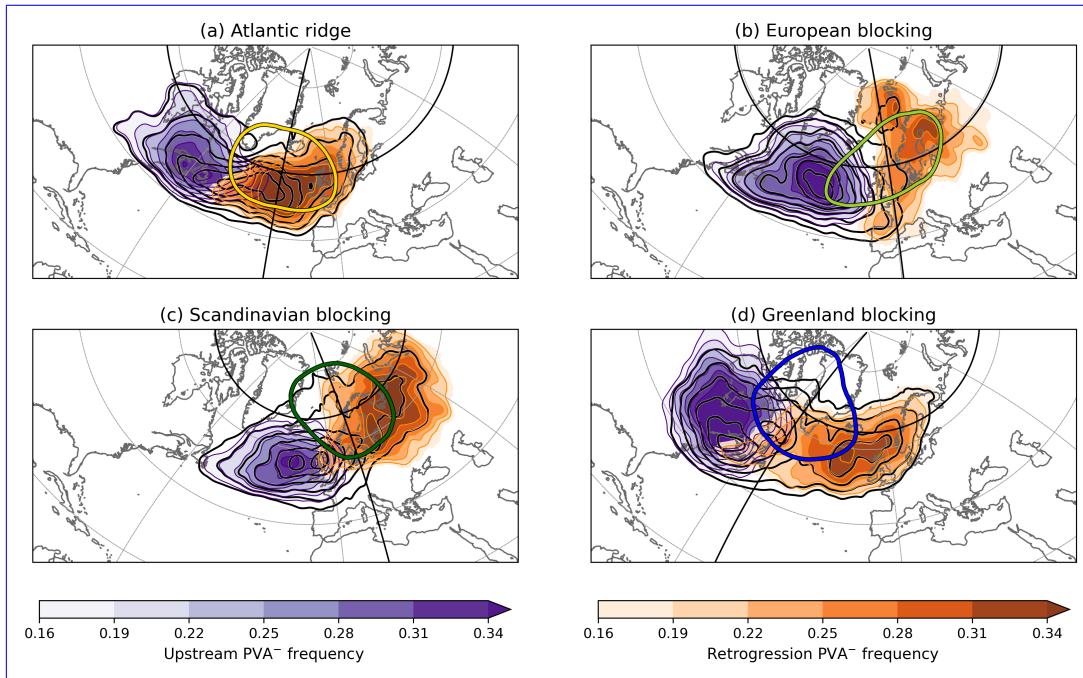
Figure 4. Mean composites (shading) of onset PVA^- frequency for the two different pathways (orange colours for retrogression pathway, violet colours for upstream pathway) at t = -72 h before blocked regime onset for the four blocked regimes. The shading represents the onset PVA^- frequency within each respective pathway subset. The data is smoothed by taking into account the time steps \pm 6 hours around t = -72 h and using a Gaussian filter with \sigma = 2 . Grey-Black contours show the total onset PVA^- frequency, independent of pathway (0.1 to 0.4 in increments of 0.03). Coloured closed contours mark the regime masks (same as in Figure 2). Dashed-Solid black vertical and horizontal lines indicate the centre of mass position of the regime mask, which is used to separate the two pathways.
