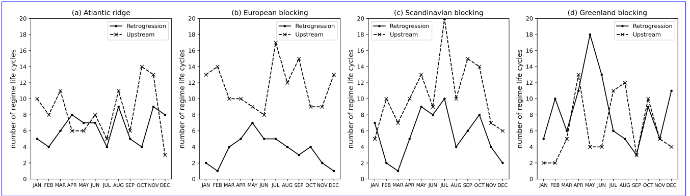
Figure 3. Monthly distribution of the absolute number of regime life cycles for the two identified pathways for each of the four blocked regimes. The retrogression pathway is shown with a solid line, and the upstream pathway with a dashed line.
