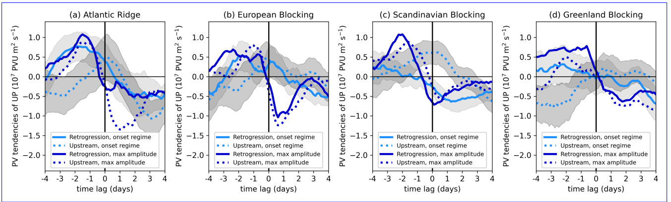
Figure 10. Temporal evolution of the upper-tropospheric PV tendency contribution to the amplitude change of onset PVAs - relative to the regime onset (light blue) and relative to the maximum in PVA - amplitude (dark blue) for the retrogression pathway (solid) and the upstream pathway (dotted). The x-axis shows the time lag around regime onset for the light blue lines and the time lag relative to the maximum amplitude of onset PVAs - for the dark blue lines. Grey shading displays \pm 1 standard deviations around the mean for the onset-centred perspective (light blue lines). The lines were smoothed using a 24 h moving window ( \pm 12 h).
