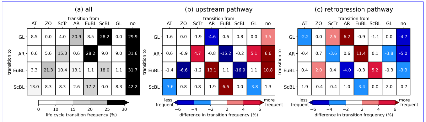
Figure 5. (a) Life cycle transition frequency (%) for all transitions into the blocked regimes (y-axis) from one of the seven regimes or the no regime (x-axis). Each row represents a blocked regime, and each column shows the share of cases (%) with the respective preceding regime. (b) Differences in transitions transition frequency for the life cycles linked to the upstream pathway in comparison compared to all life cycles, independent of pathway. (c) Differences in transitions frequency Same as panel b, but for the life cycles linked to the retrogression pathway in comparison to all.
