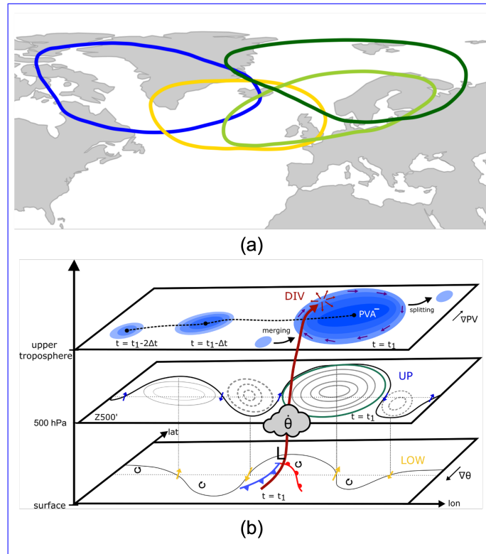
Figure 1. (a) Subregions for blocking in the North Atlantic–European sector obtained from a weather regime perspective. The solid, closed contour lines mark the areas of the anticyclonic PV anomaly associated with the blocked regime patterns: Atlantic Ridge (gold), European Blocking (yellow-green), Scandinavian Blocking (dark green), and Greenland Blocking (blue). (b) Schematic of the quasi-Lagrangian potential vorticity framework (Hauser et al., 2023, 2024b). Upper-troposphere level: Exemplary track (black dashed) of negative PV anomalies (blue shading, PVA^- ), including splitting and merging of existing anomalies; impact of divergent outflow near the tropopause (DIV, dark-red arrows); and wind fields induced by upper-tropospheric PV anomalies (dark-blue arrows). 500 hPa level: absolute geopotential height ( Z500 ; black), Z500 anomalies ( Z500' ; grey; solid for positive, dashed for negative), contour of the anticyclonic anomaly as in panel (a) (green), and wind fields linked to barotropic phase-propagation tendencies (UP, blue arrows). Surface: temperature wave (solid black line), influence of wind fields linked to low-level PV anomalies on higher levels (LOW, gold arrows), symbolic low-pressure system (L) with cold (blue) and warm (red) fronts, and a warm-conveyor-belt airstream (dark-red arrow) with diabatic heating in the mid-troposphere (grey cloud).
