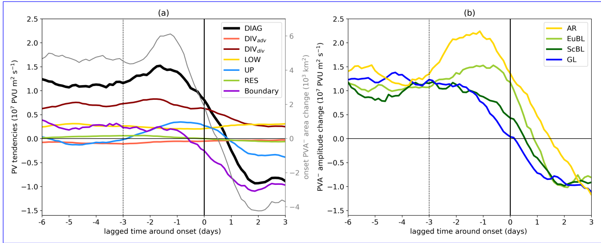
Figure 6. (a) Composite of amplitude-modifying contributions (left y-axis) to the diagnosed amplitude change of onset PVAs - (DIAG, black) for all blocked regime life cycles independent of type, following Equation 2: advection part of the divergent outflow term ( DIV_{adv} , -\mathbf{v}_{div} \cdot \nabla q_0 , light red), divergence part of the divergent outflow term ( DIV_{div} , q'(\nabla \cdot \mathbf{v}_{div}) , dark red), baroclinic interaction (LOW, -\mathbf{v}_{up} \cdot \nabla q_0 , gold), upper-tropospheric wave dynamics (UP, -\mathbf{v}_{up} \cdot \nabla q_0 , blue), the residual PV tendency term (RES, -\mathbf{v}_{res} \cdot \nabla q_0 , yellow green) and the boundary term (Boundary, dark violet). The sign of the PV tendencies is defined such that positive (negative) values always indicate amplification (weakening) of the PVAs - . The grey line shows the mean change in onset PVA - area (right y-axis). (b) Mean diagnosed amplitude change of onset PVAs - around blocked regime onset for the four blocked regimes separately. Note that all curves are smoothed by taking into account the time steps +/- 12 h.
