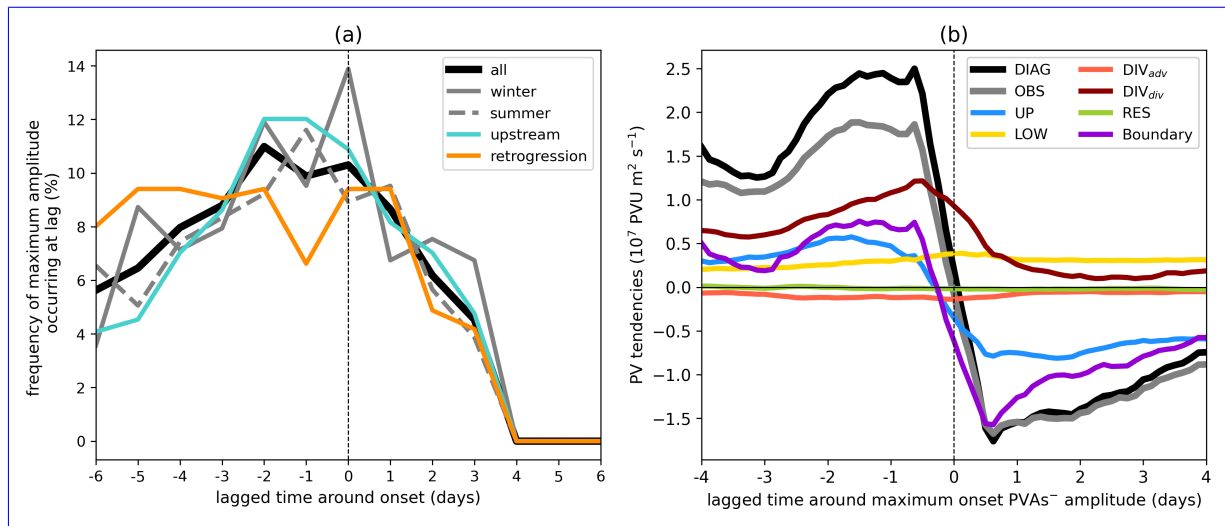
Figure 9. (a) Timing of maximum amplitude for onset PVAs - within the period -6 to +6 days around onset for all year-round regime life cycles (black), only for those in extended winter (NDJFM, solid grey) and extended summer (MJJAS, dashed grey), for all following the upstream pathway (turquoise) and the retrogression pathway (orange). (b) Mean of integrated PV tendencies over the onset PVAs - centred on the timing of their maximum amplitude (see panel a) and for all blocked regime life cycles. The lines have been smoothed by performing a centred 24 h running-mean.
