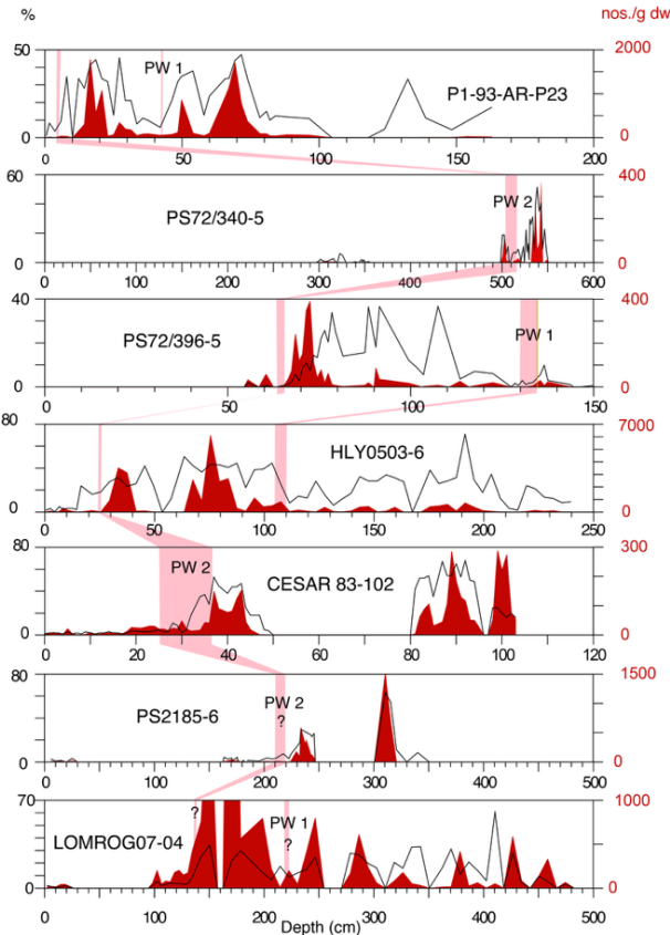
Figure 11: Stratigraphic occurrence of B. arctica across the Arctic Ocean. Core locations are shown in Figure 1. Absolute abundances (>63µm) of cores P1-93-AR-P23, HLY0503-6, and LOMROG07-04 are from Lazar and Polyak (2016), and CESAR83-102 from Scott et al. (1989). The depth intervals of the pink-white layers are from Cronin et al. (2014) and Scott et al. (1989). %: relative abundances; nos./g dw: absolute abundances. Absolute abundances in core CESAR83-102 are numbers/10ccm wet sample (Scott et al., 1989).
