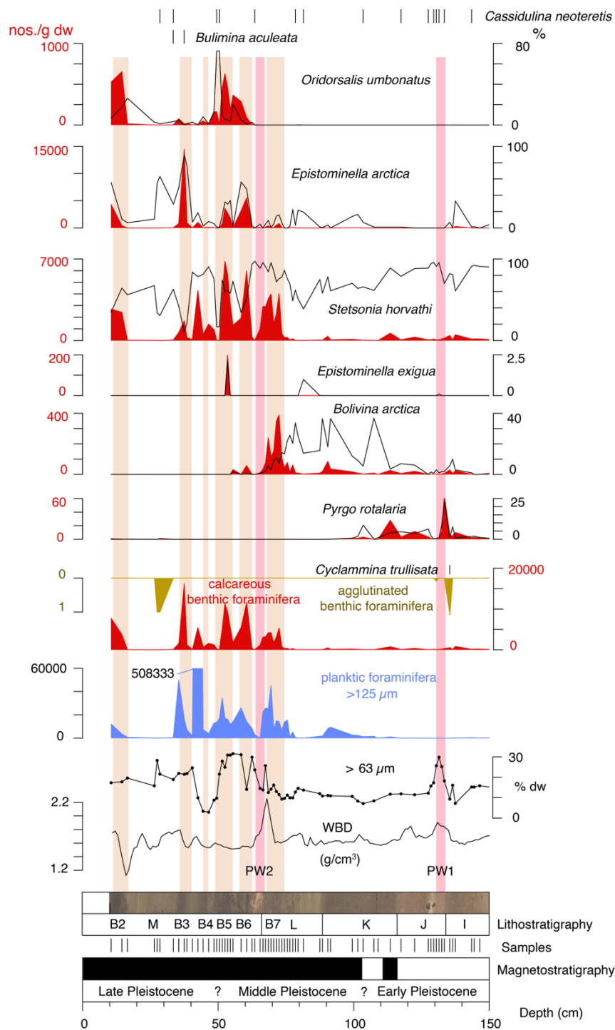
Figure 3: Stratigraphic distribution of selected benthic foraminifera (> 63 \mu m) in sediment core PS72/396-5 from the western
