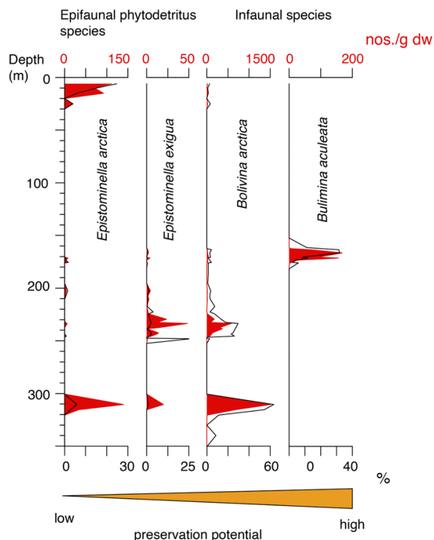
770 Figure 12: Influence of the preservation potential (qualitative assessment based on Appendix B: Ecology, shell characteristics, and preservation of main calcareous taxa) of Epistominella arctica , E. exigua , Bolivina arctica and Bulimina aculeata on the formation of absolute abundance maxima in core PS2185-6. The more robust species are successively enriched with increasing selective dissolution.
