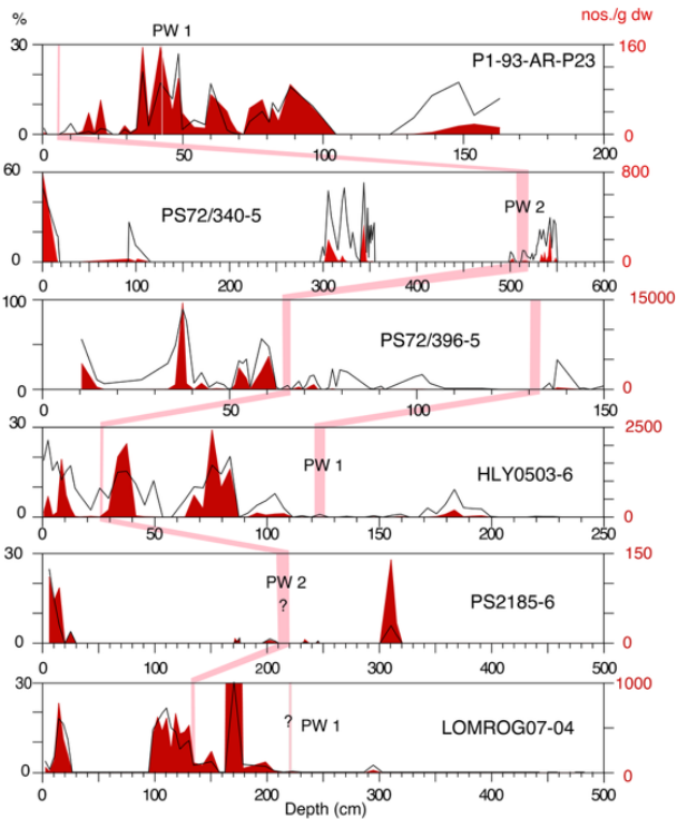
515 Figure 10: Stratigraphic occurrence of E. arctica across the Arctic Ocean. Core locations are shown in Figure 1. Absolute abundances (>63µm) of cores P1-93-AR-P23, HLY0503-6, and LOMROG07-04 are from Lazar and Polyak (2016). The depth intervals of the pink-white layers in these cores are from Cronin et al. (2014). %: relative abundances; nos./g dw: absolute abundances.
