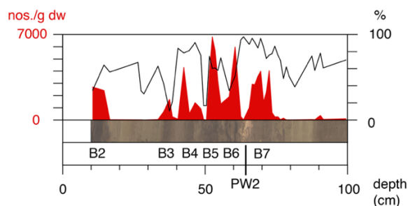
Figure 2: Digital image of core PS72/396-5 and relative (%) and absolute (nos./g dw) abundances of Stetsonia horvathi . This species dominates in most assemblages but only shows distinct absolute abundance maxima in the brown layers and in the pink-white layer PW 2. Please note that bioturbation has blurred the clear distinction between foraminifer-rich brown and foraminifer-poor grey layers, making distinction of specific brown layers difficult. Brown layer terminology after Polyak et al. (2004) and Stein et al. (2010b).
