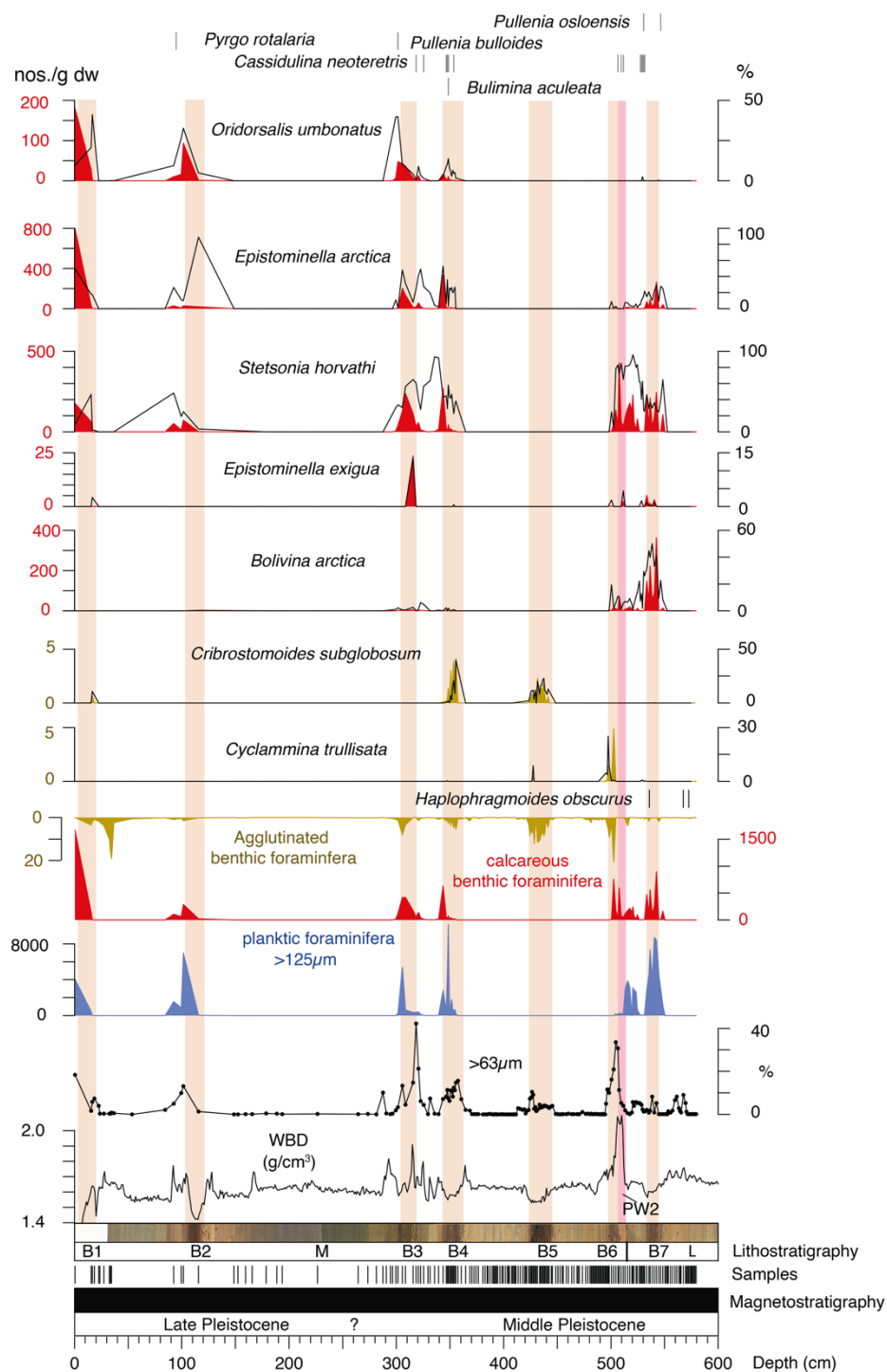
Figure 4: Stratigraphic distribution of selected benthic foraminifera in sediment core PS72/340-5 from the western Mendeleev Ridge area. Only the presence of Bulimina aculeata , Cassidulina neoteretis , Pullenia bulloides , Pullenia osloensis and Pyrgo rotalaria is noted
