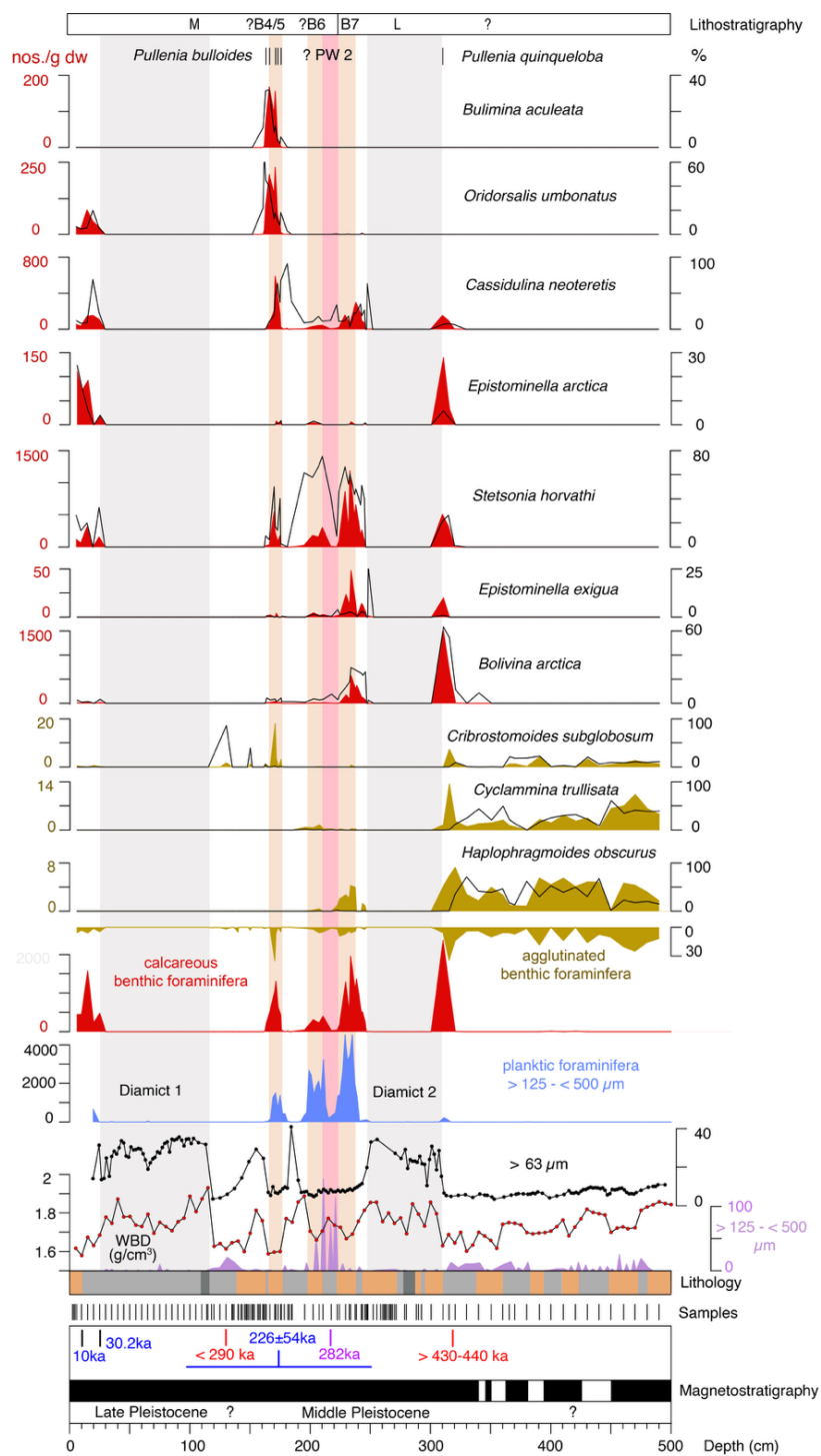
Figure 5: Stratigraphic distribution of selected benthic foraminifera in sediment core PS2185-6 from Lomonosov Ridge. Only the
