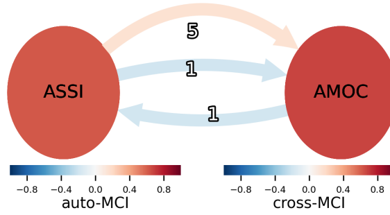
Figure F2. The causal network of the applied experiment (Fig. 5) without Arctic temperatures.
