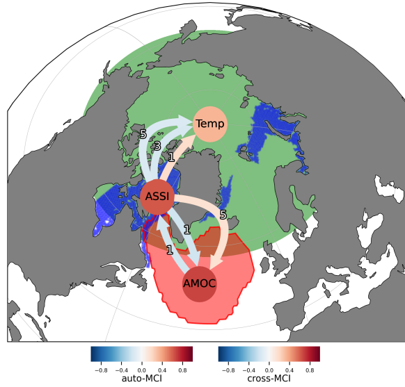
Figure 5. Causal network between Arctic summer sea ice ASSI (blue), the AMOC (red), and Arctic temperatures (green), as detected by the PCMCI method. A bidirectional stabilizing interaction of Arctic sea ice ASSI and the AMOC is found, while a confounding effect of Arctic temperatures is refuted. The arrow shading indicates the sign and significance derived by PCMCI. Note that the positive highest effect strength for the interaction coefficient from Arctic summer sea ice ASSI to the Arctic temperatures implied by the arrow shading does not correspond to the strongest effect is found at a lag of the three delays months, for which the coefficient is negative , implying an inversely proportional effect.
