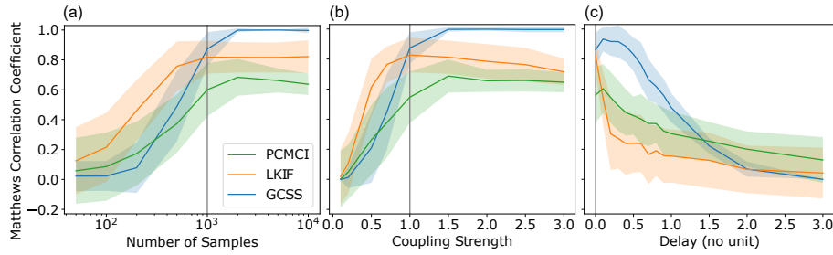
Figure 2. Relationship between basic data parameters and prediction scores of the algorithms and basic data parameters : (a) Prediction scores increase between 200 and 1000 provided samples, with LKIF being most reliable in intermediate numbers of samples, and GCSS most reliable for larger numbers. (b) Similar development for coupling strengths between variables, where scores increase massively from strengths of 0.1 strength and 1.0, with a higher convergence for GCSS than for LKIF and PCMCI. (c) Delays of interactions decrease performance for all algorithms delay length (default: 1000 samples, GCSS can handle small delays well coupling strength 1, no delay). Grey vertical lines indicate default values. Shaded areas indicate one standard deviation.
