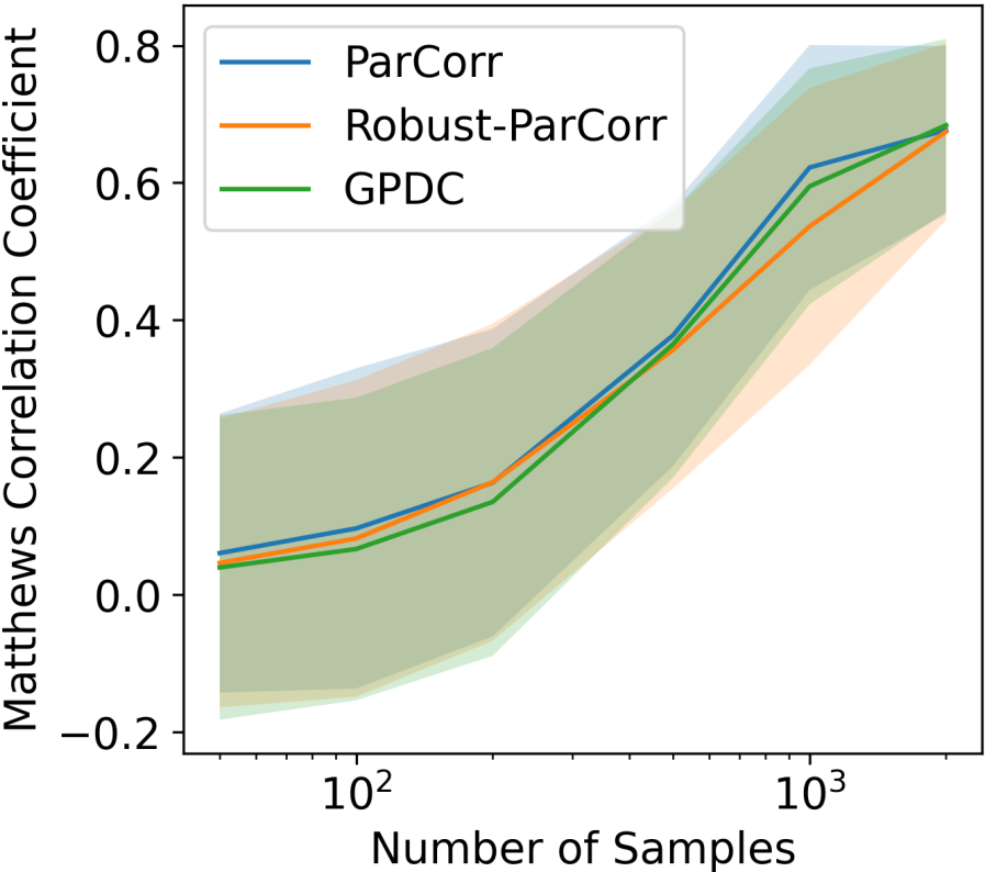
Figure D1. The performance MCC scores of PCMCI with the three compared different conditional independence tests is highly similar, with a small advantage of the partial correlation test over the other two.
